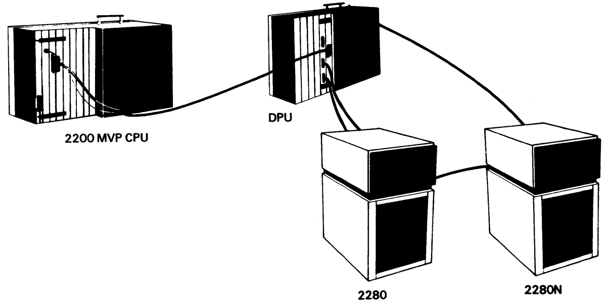
Figure 2-2. Model 2280/2280N Dual System Configuration
