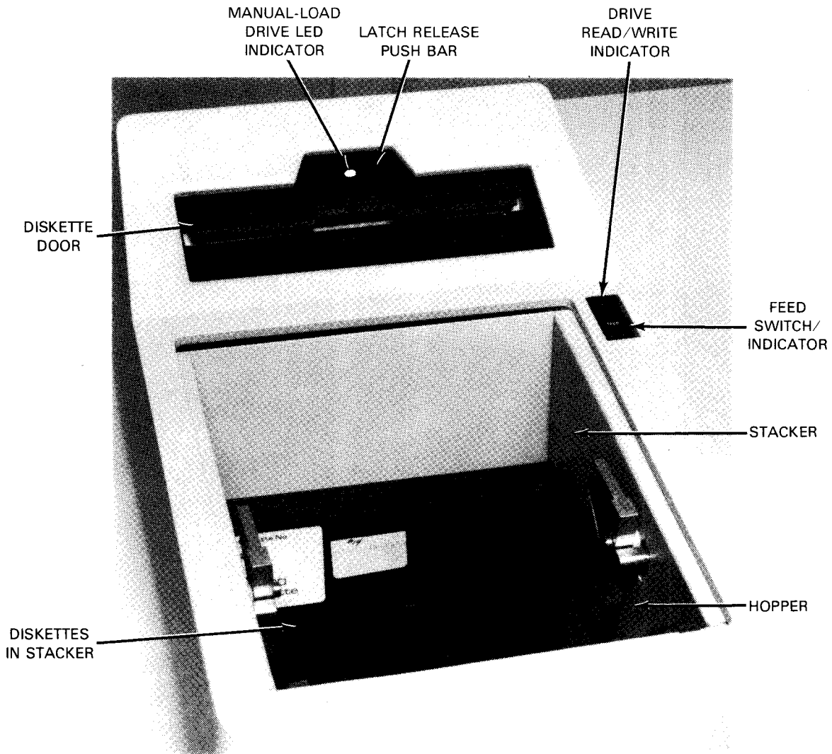
Figure 4-2. Autoload Diskette Drive FEED Switch and Indicator
