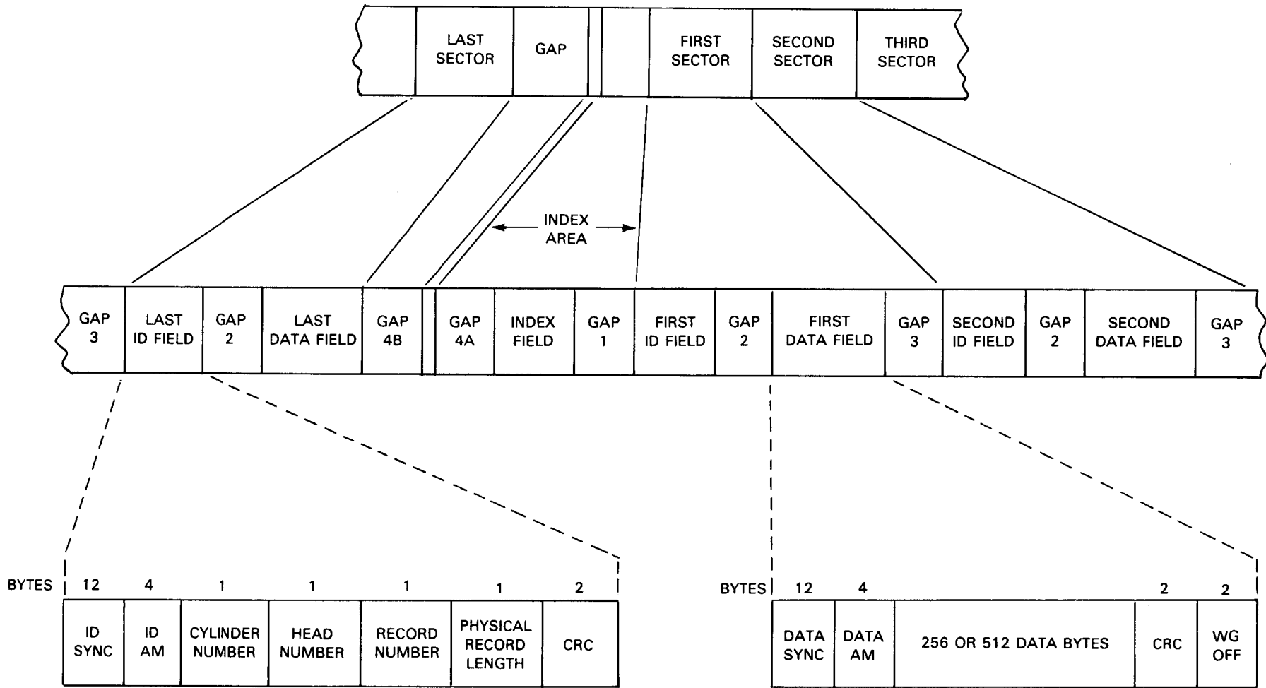
Figure 2-5. MFM Track Format
