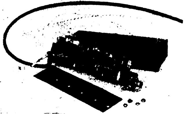
Fig. 3—Typical 5-stage intermediate-frequency amplifier using subminiature components. This amplifier chassis is 6\frac{1}{2} inches long by 1\frac{1}{4} inches wide.
