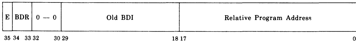
X_a After Execution of LDJ, LIJ, or LBJ instruction
