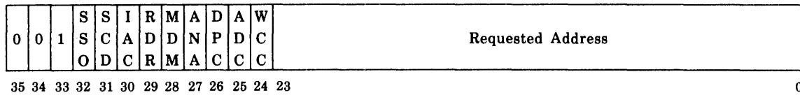
Figure 6-2. SIU/MSU Interface Storage Check Interrupt Status Format
