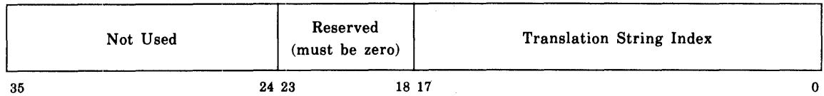
Translation Table Index Register
