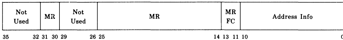
MSU Maintenance Operation Format (Internal Storage)
