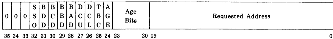
Figure 6-1. Internal SIU Storage Check Interrupt Status Format
