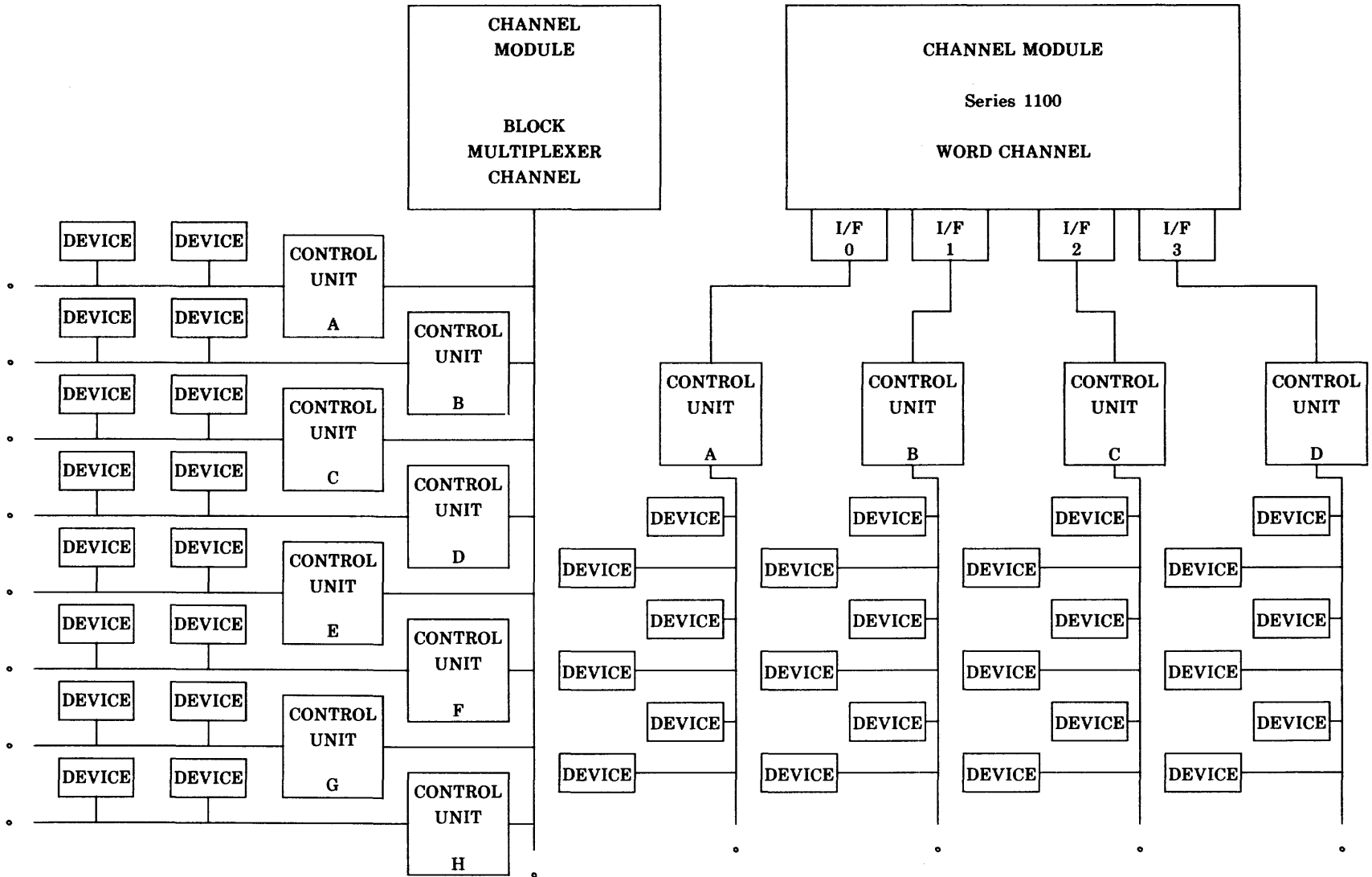
Figure 4-2. Block Multiplexer Channel Compared to Word Channel
