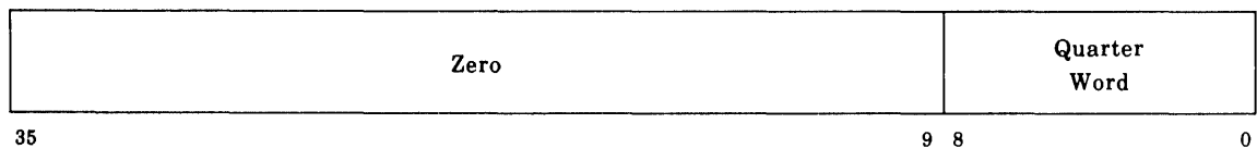
Destination A_a -Register
