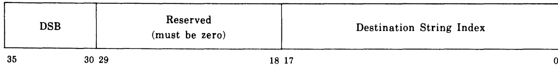
Destination String Index Register
