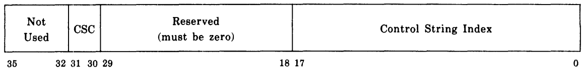
Control String Index Register
