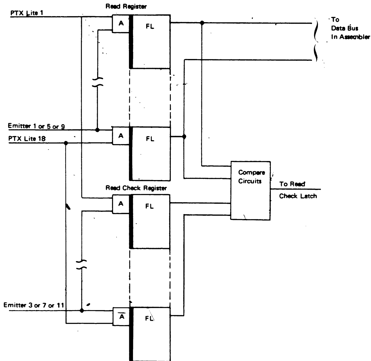
Figure 2-5. Read Register and Read Check Register
