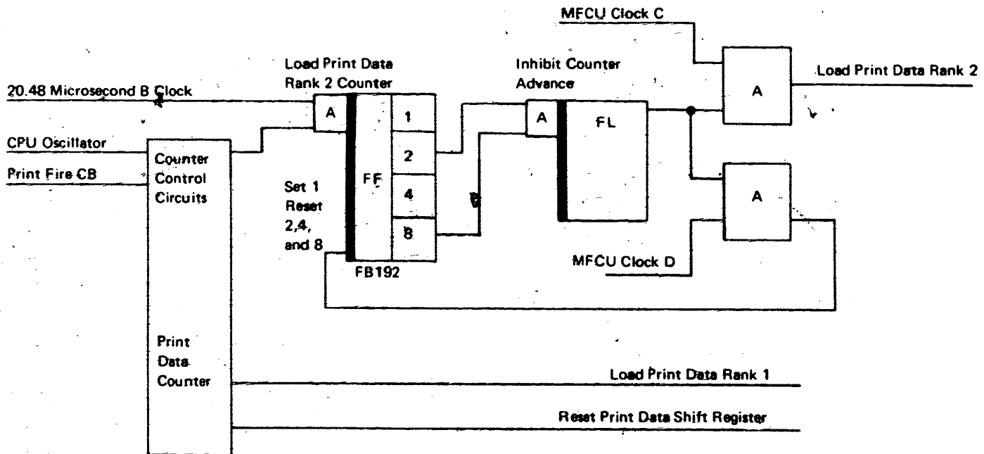
Figure 2-14. Load Print Data Rank 2 Counter
