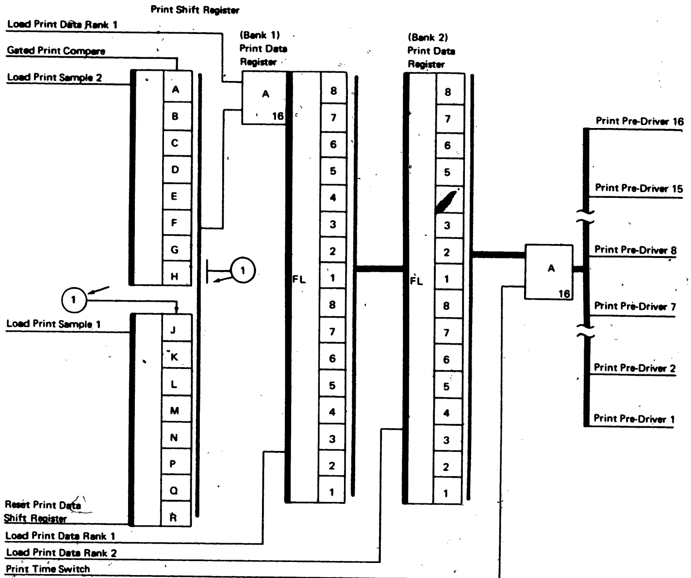
Figure 2-15. Print Shift Register and Print Data Registers
