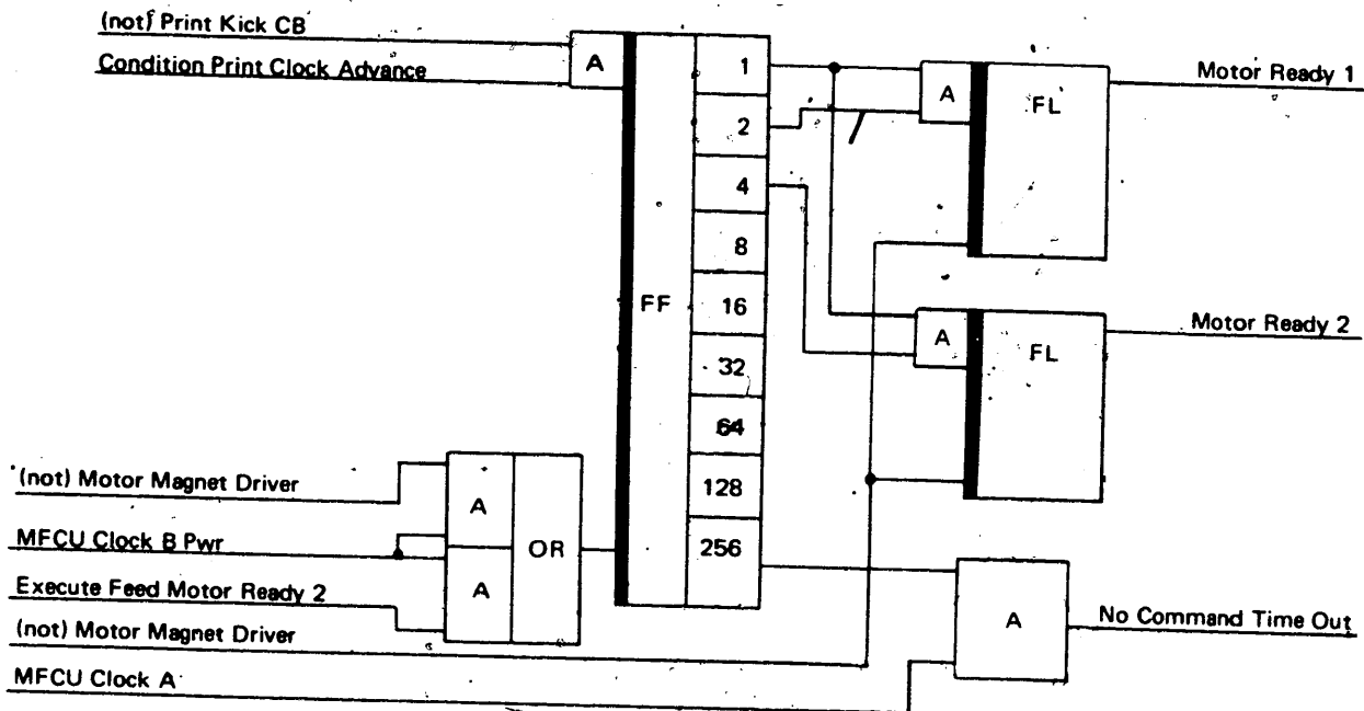
Figure 2-19. Nine Stage Time Delay Counter
