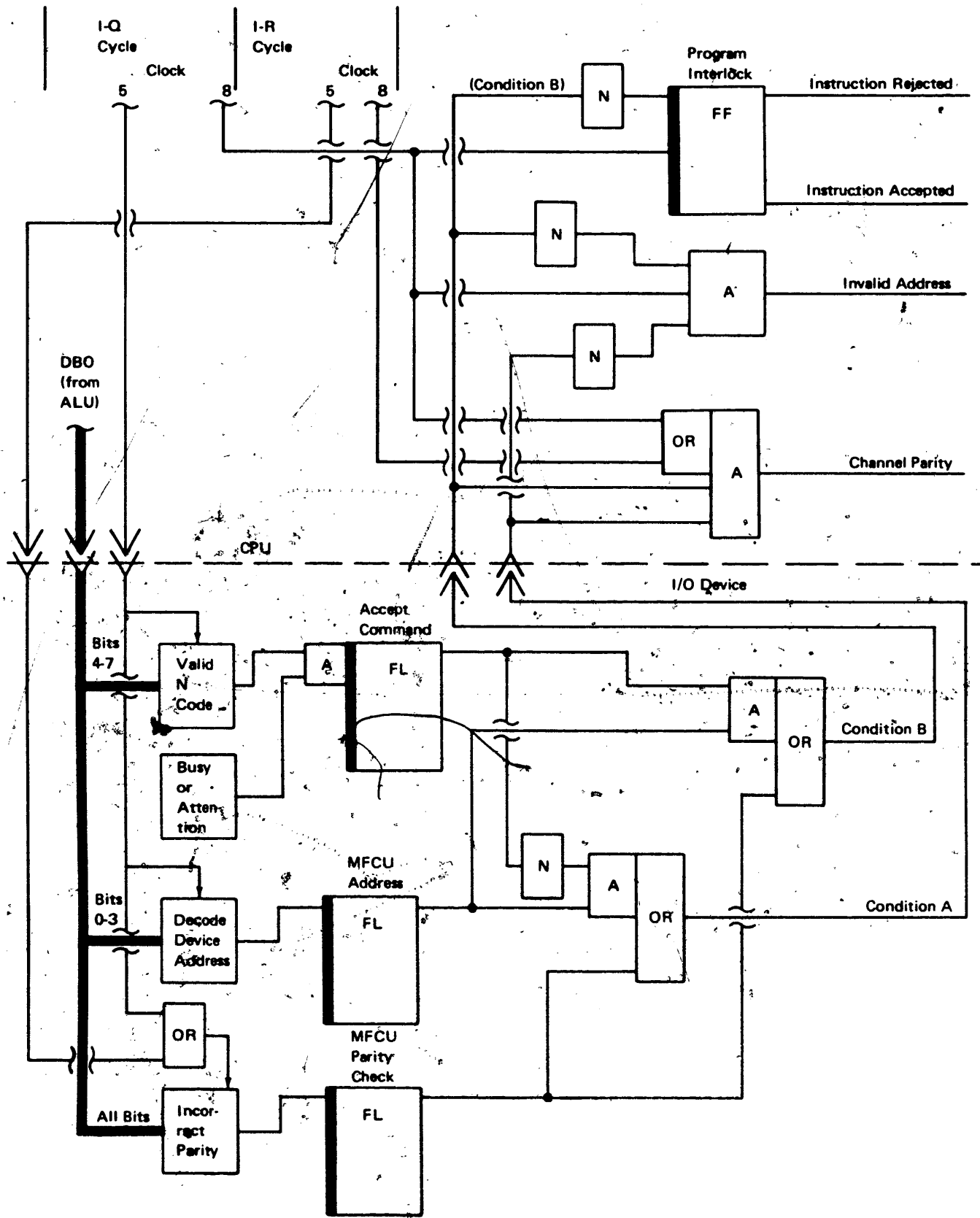
Figure 1-2. SIO-CPU/MFCU Control
