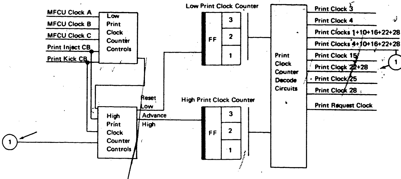
Figure 2-11. Print Clock Counters
