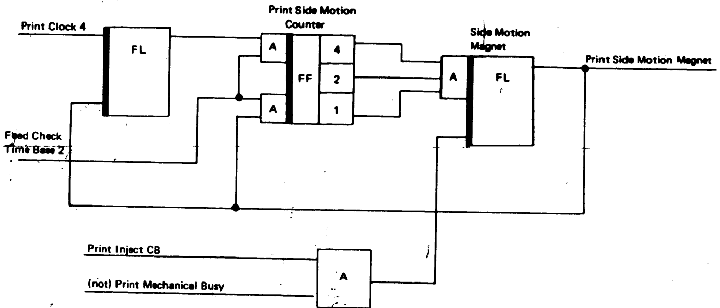
Figure 2-12. Print Side Motion Counter and Control
