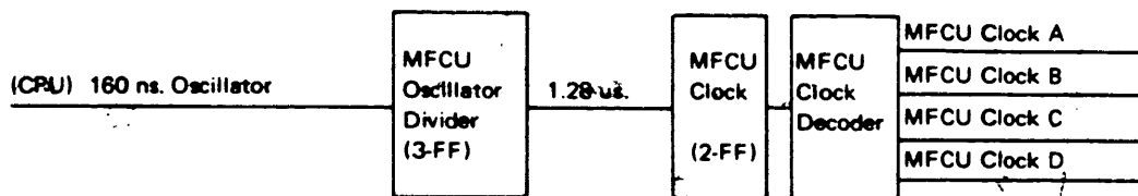
Figure 2-1. MFCU Clock
