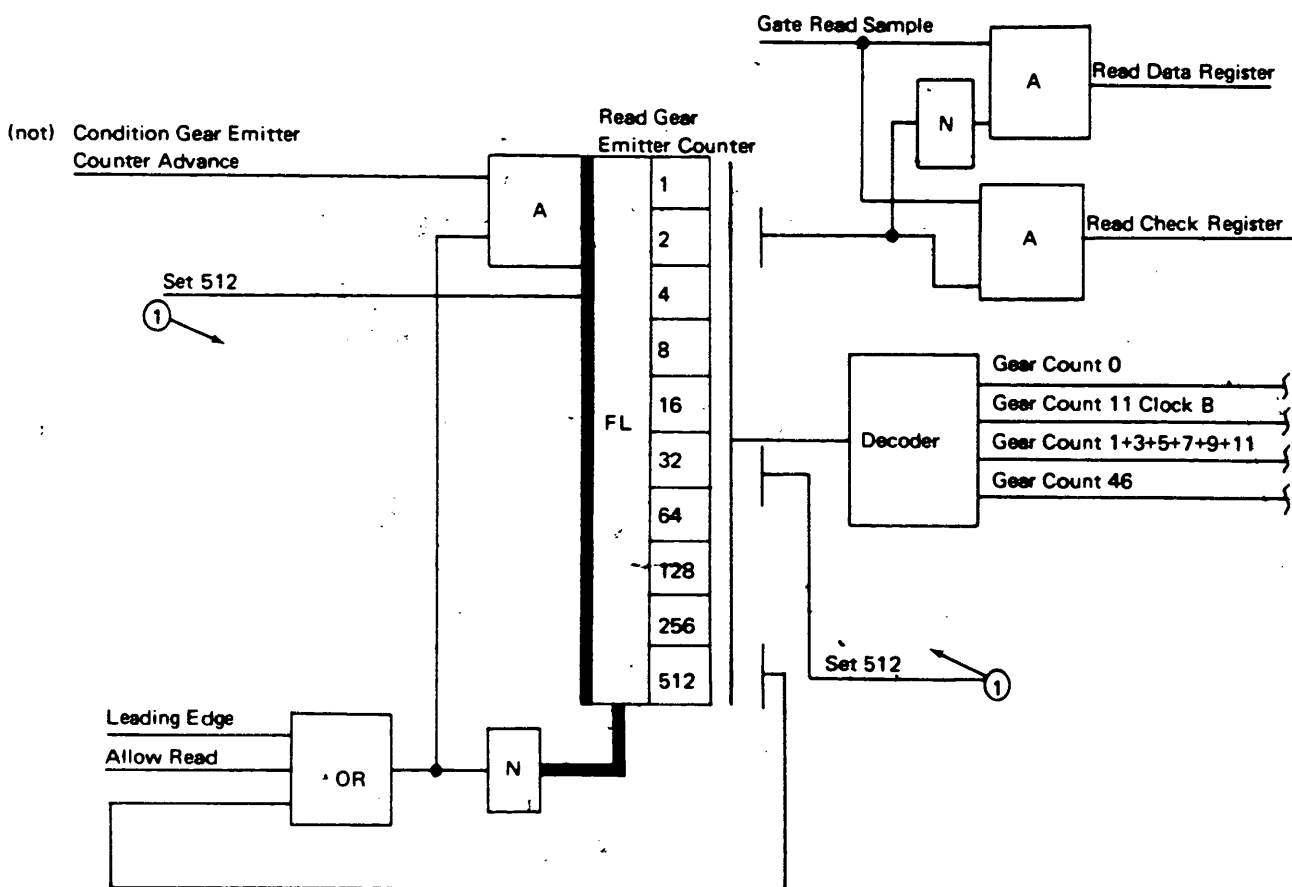
Figure 2-4. Read Gear Emitter Counter and Decoder
