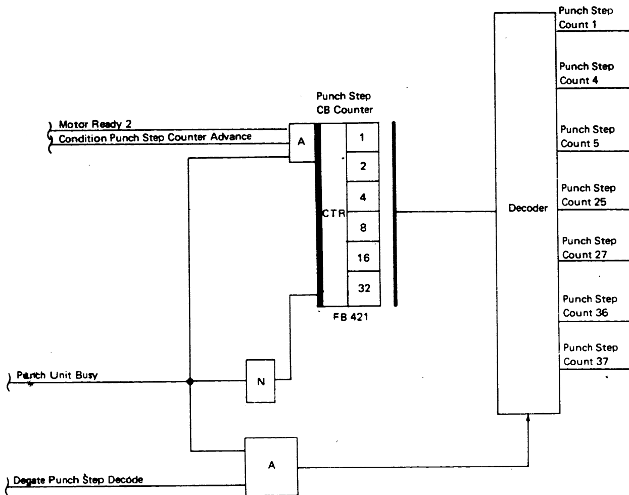
Figure 2-7. Punch Step CB Counter and Decoder
