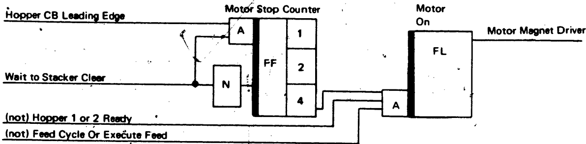
Figure 2-20. Motor Stop Counter
