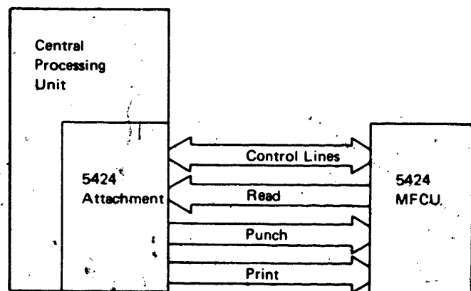
Figure 1-1. 5424 Data Flow
