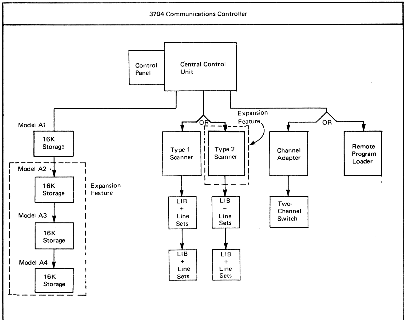
Figure 2-3. Maximum Hardware Configuration of the 3704
