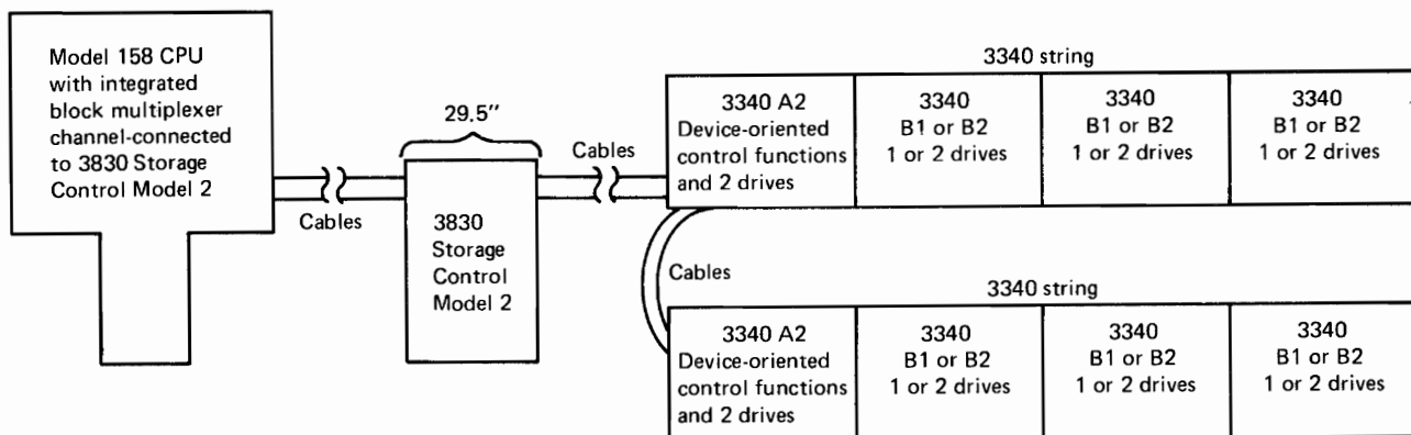
Figure 50.15.7. A Model 158 configuration with 3340 disk storage attached via 3830 Storage Control Model 2
