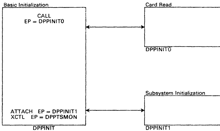
Figure 3-5. The Special Real Time Operating System Initialization
