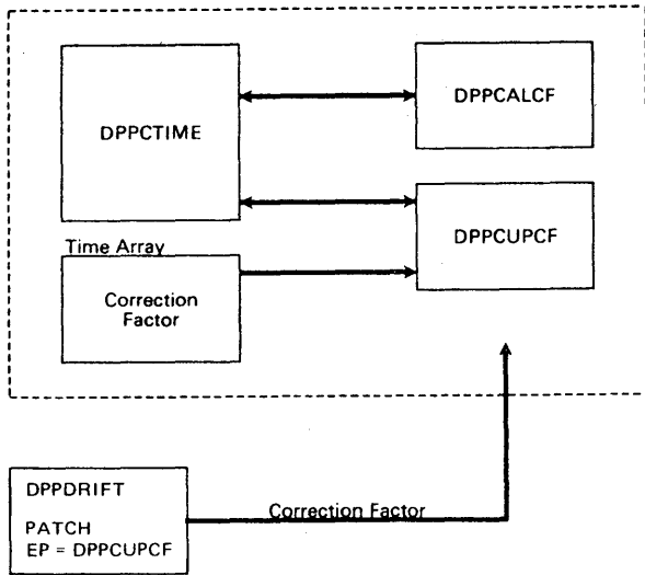
Figure 2-8. Time Drift-Special Real Time Operating System Time Relationship
