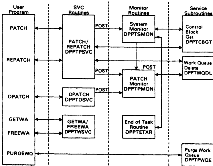
Figure 2-2. Task Management Overview
