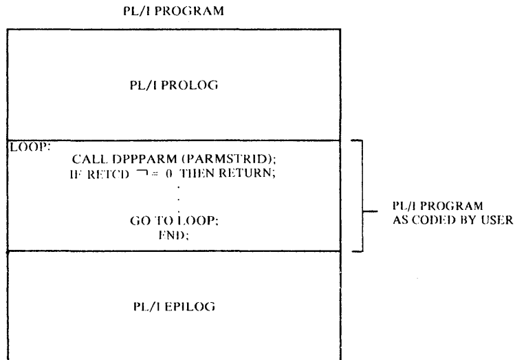
Figure 2-14. PL/I Example
