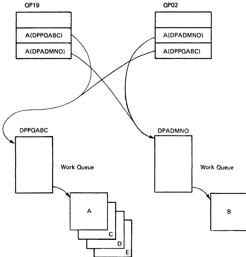
Figure 2-6.1. Task/Queue Structure
