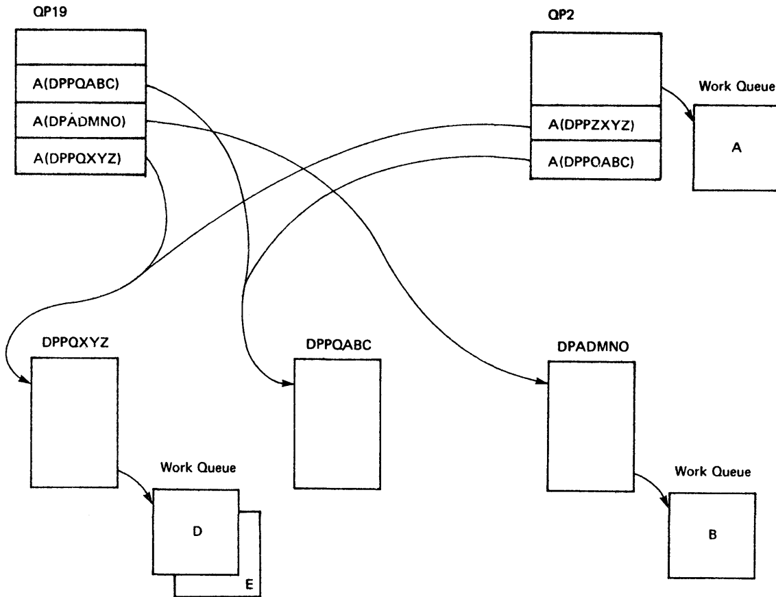
Figure 2-6.4. Task/Queue Processing
