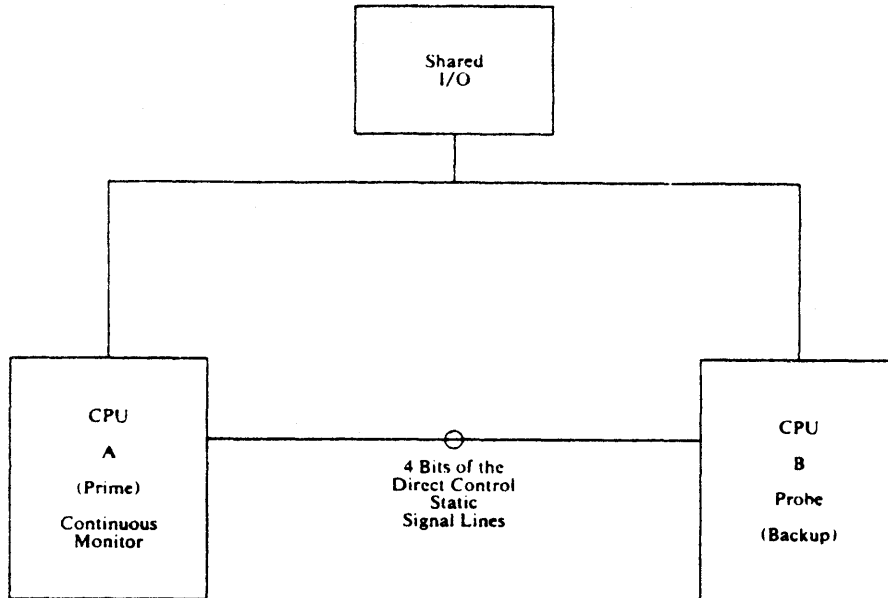
Figure 2-28. Probe Function Failure/Restart Feature
