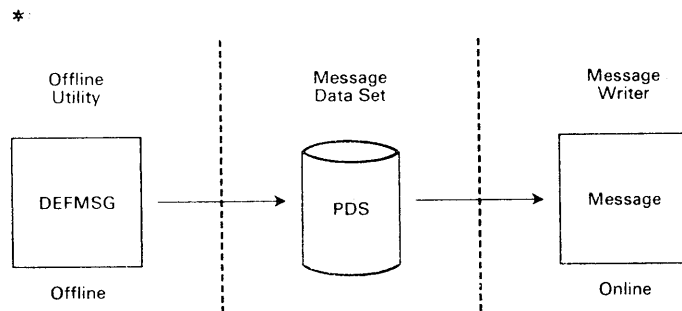
Figure 2-9. Real Time Message Handler Components
