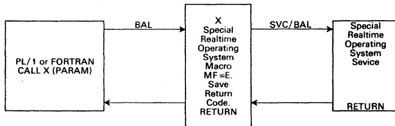
Figure 2-13. High-Level Language Interfaces for the Special Real Time Operating System Services
