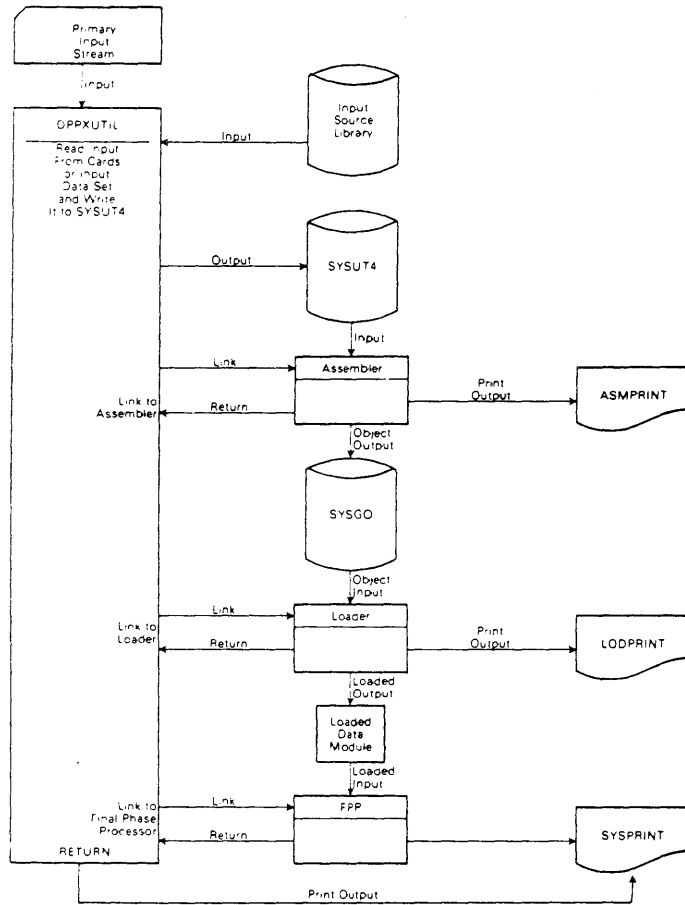
Figure 3-9. Online Data Set Processing Overview
