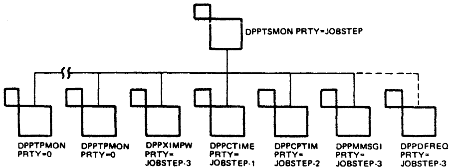
Figure 2-3. The Special Real Time Operating System Task Structure and Priorities
