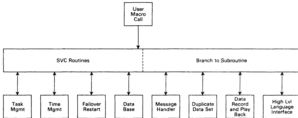
Figure 2-1. The Special Real Time Operating System Overview of the Online System
