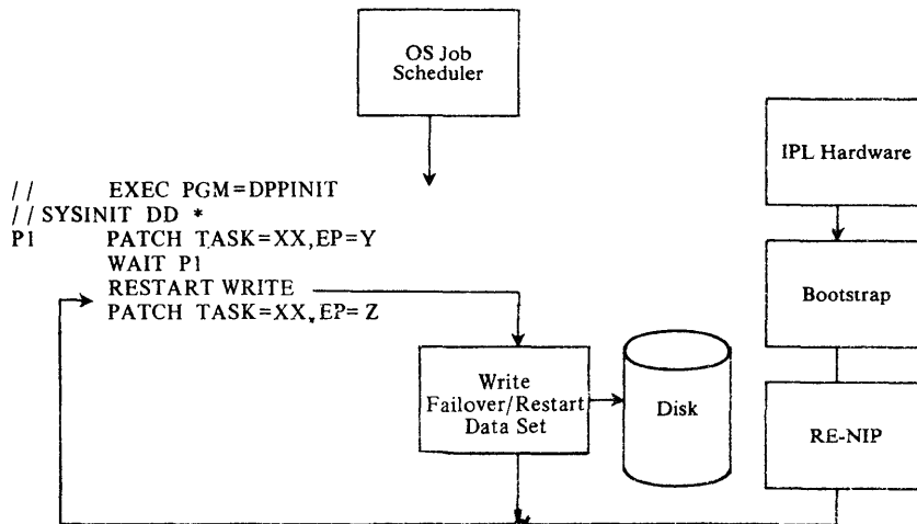
Figure 2-27. Restart Process
