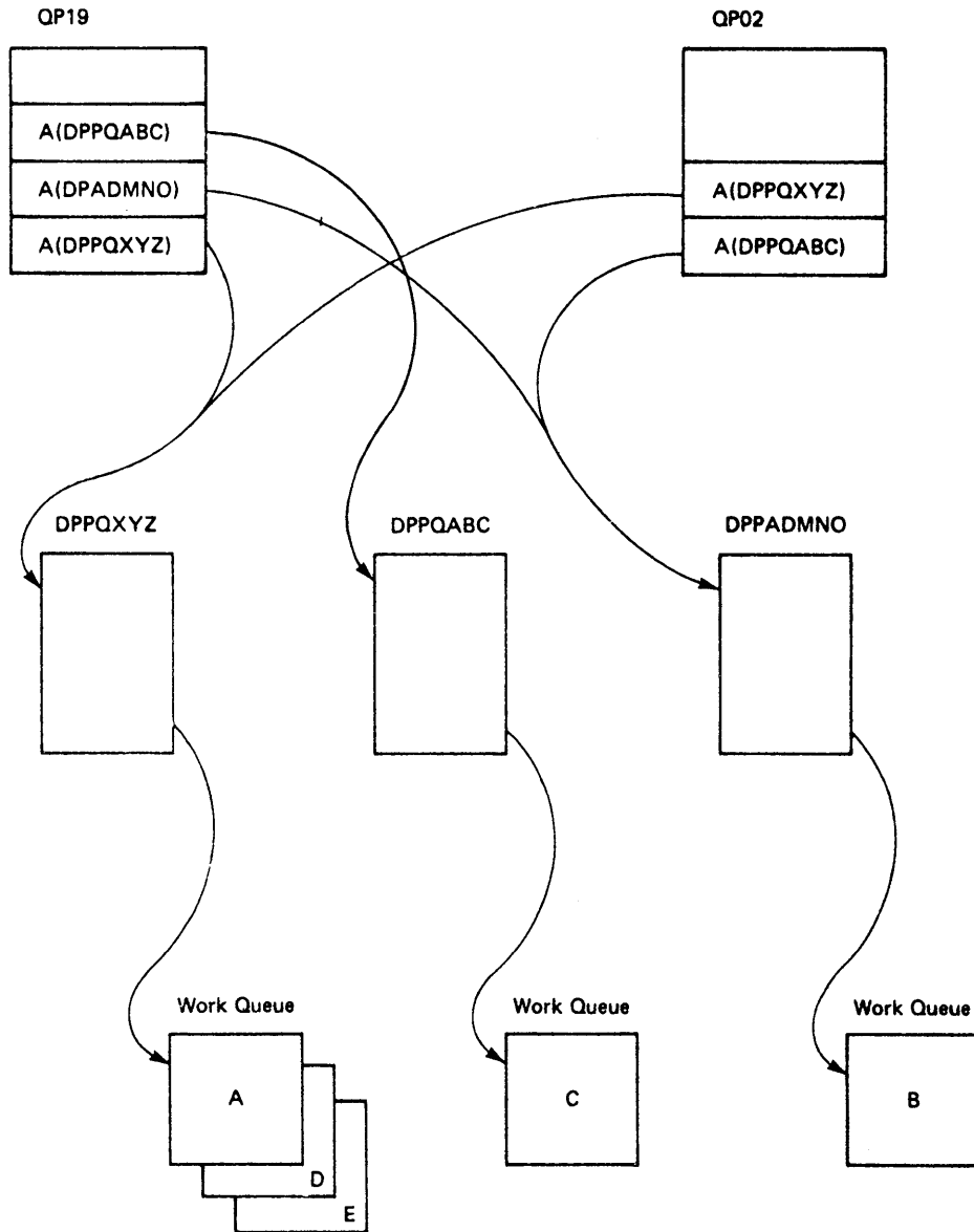
Figure 2-6.3. Task/Queue Structure
