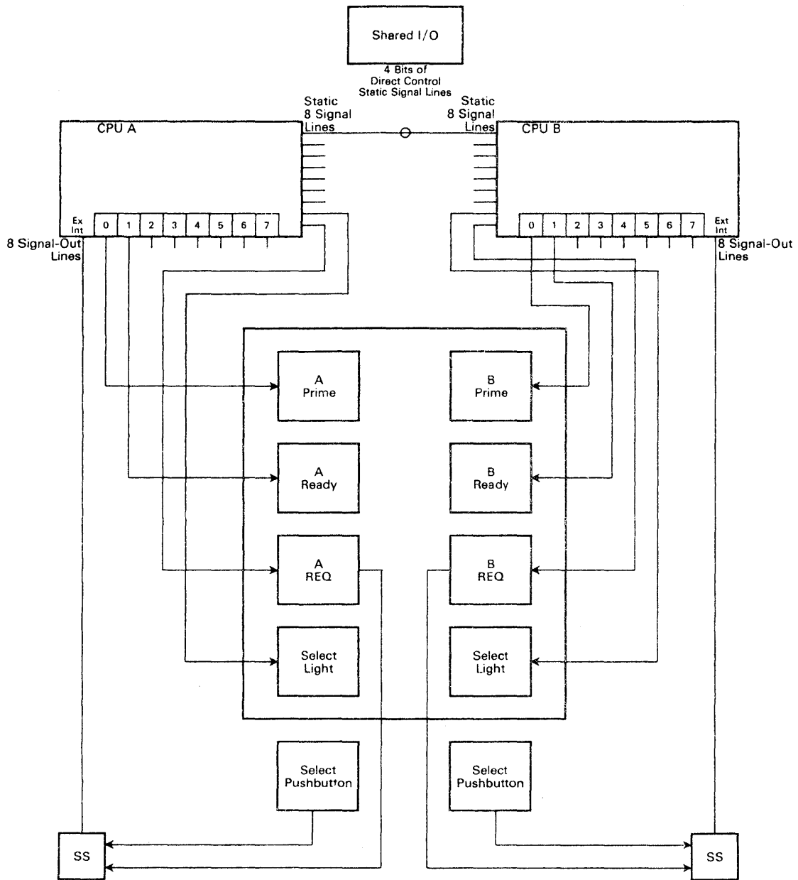
Figure 2-32. Computer Status Panel Connections (Functional)
