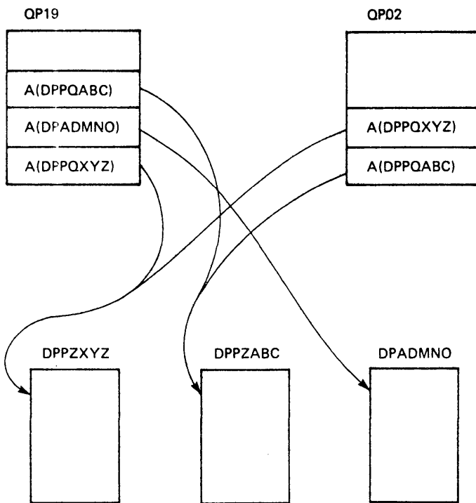
Figure 2-6.2. Queue Processor/Queue Holder Structure
