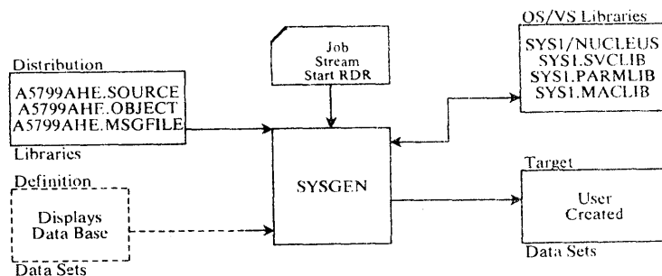
Figure 3-3. The Special Real Time Operating System SYSGEN - Stage II
