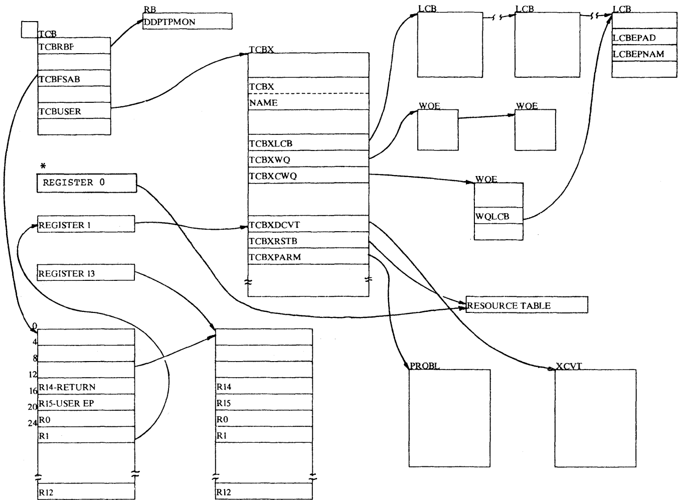
Figure 2-33. Control Block Format Entry to PATCHed Program
