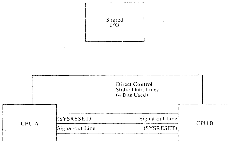
Figure 2-29. Remote System Reset Feature
