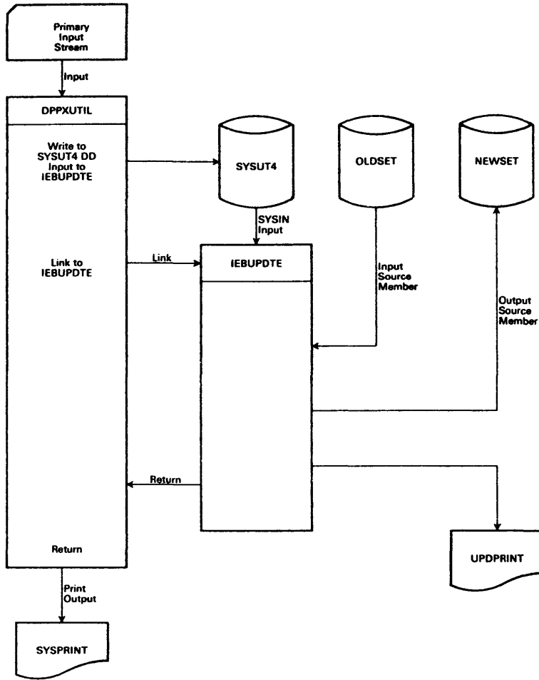
Figure 3-8. Update Processing Overview
