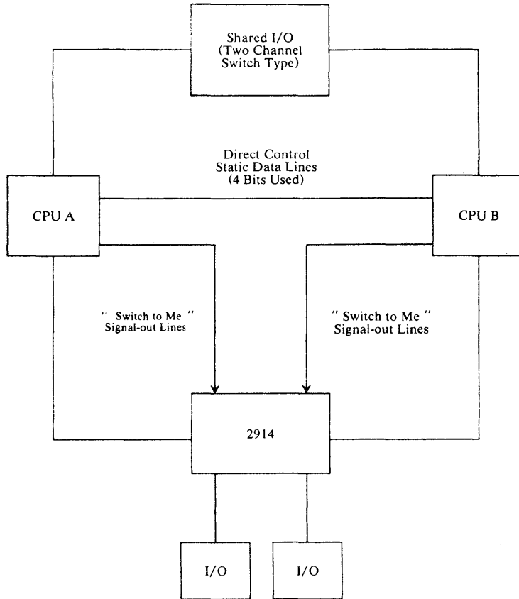
Figure 2-30. System With Automatic 2914 Switch
