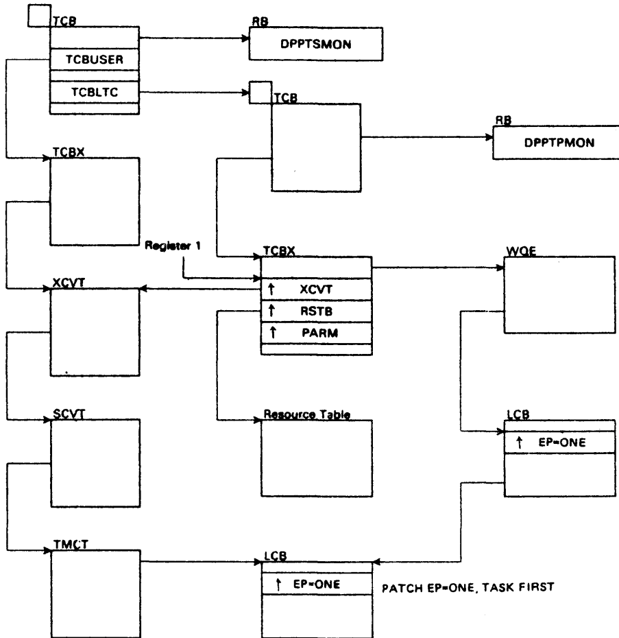
Figure 2-4. Task Management Control Blocks
