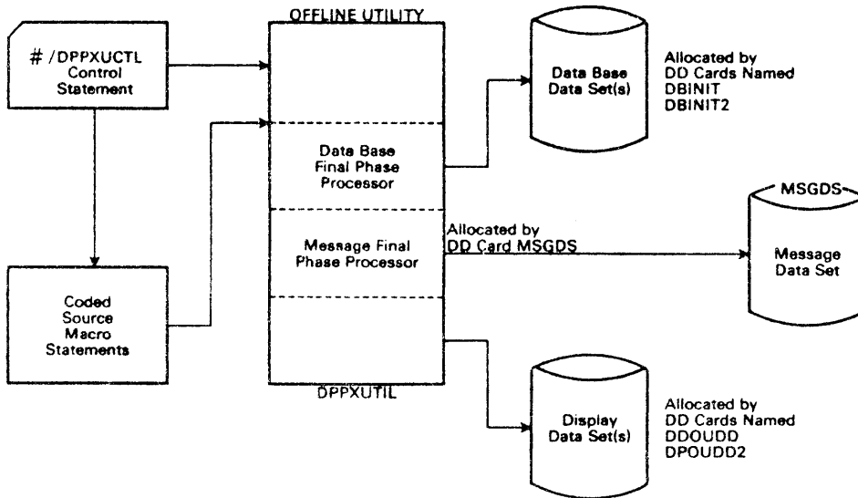
Figure 3-7. Offline Utility Processing Overview
