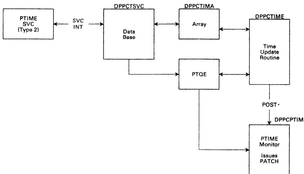
Figure 2-7. PTIME Logic and Control Flow
