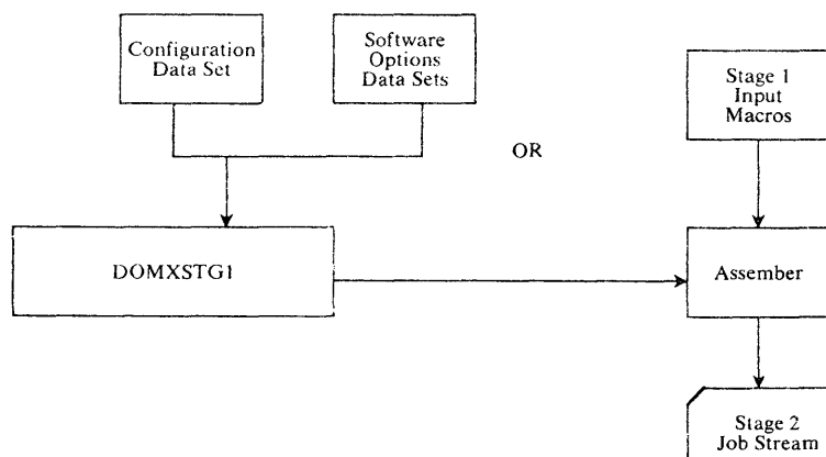
Figure 3-2. The Special Real Time Operating System - SYSGEN - Stage I
