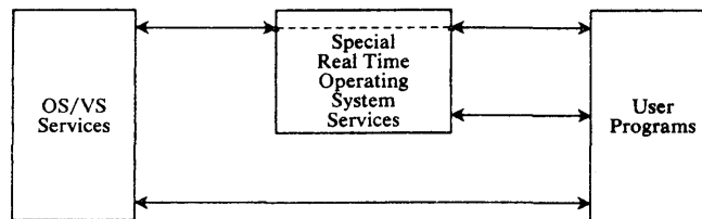
Figure 1-1. -User Special Real Time Operating System-OS/VS Interface
