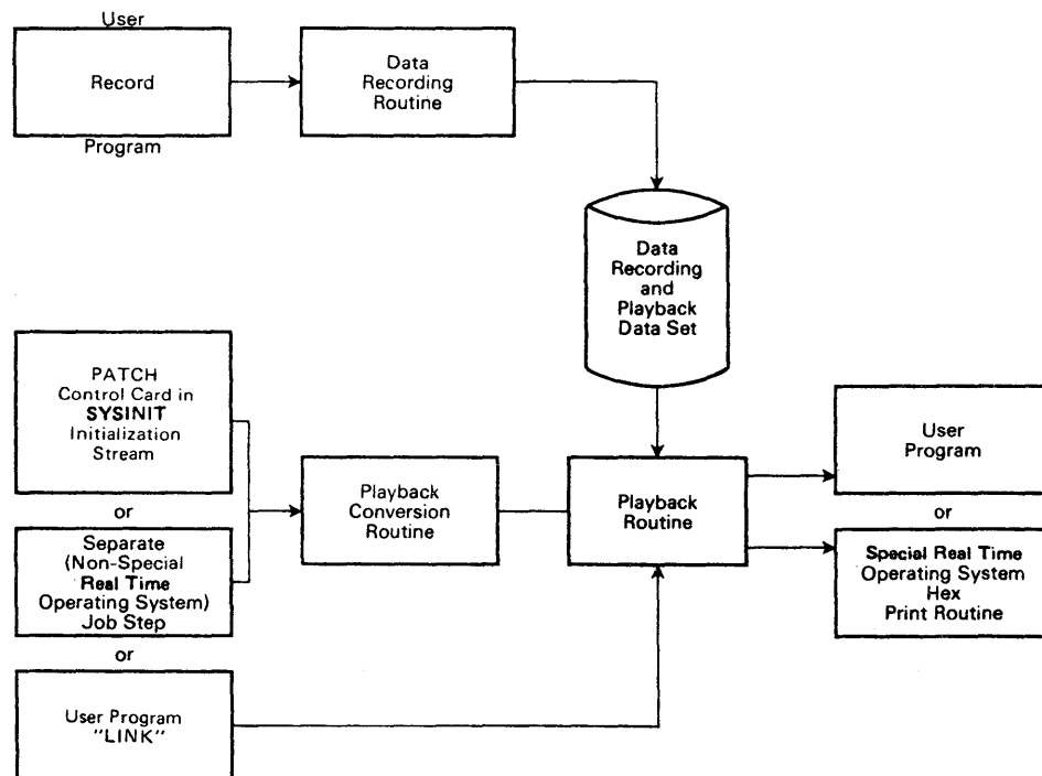
Figure 2-11. Data recording and Playback Processing Overview
