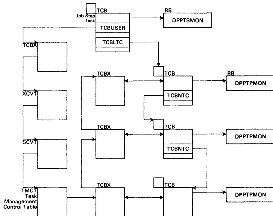
Figure 2-6. Control Blocks After Initialization
