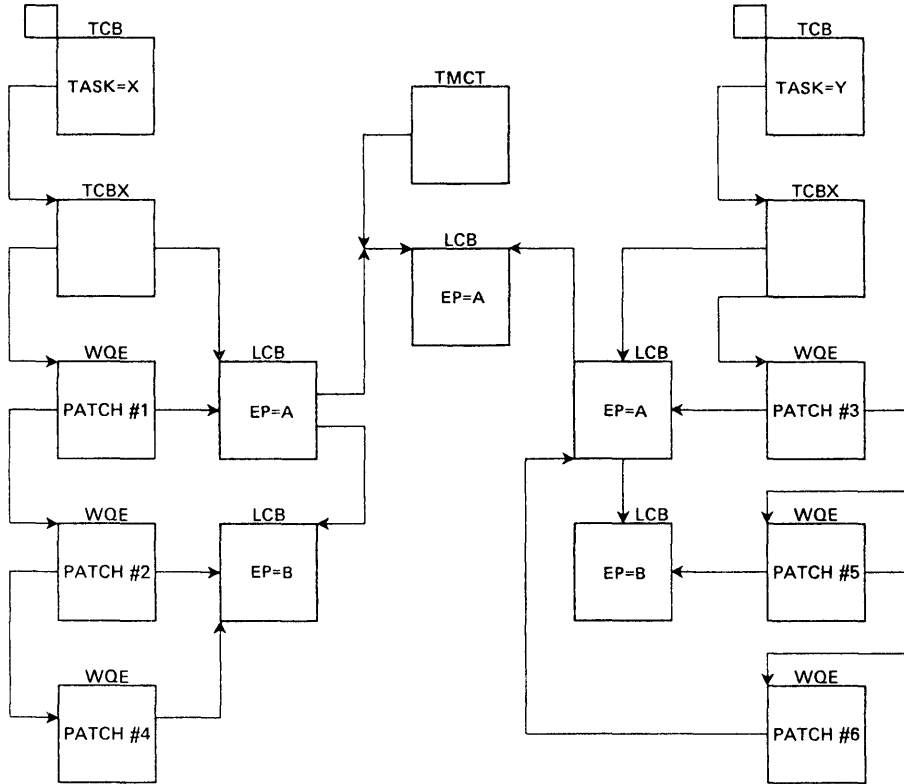
Figure 2-5. Control Blocks Built for Example 1
