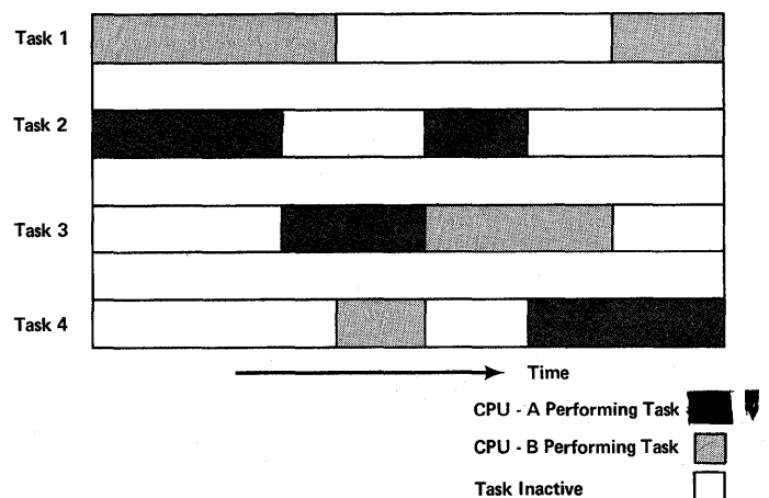
Figure 60. Two CPUs in Multisystem Mode, Balancing the Execution of Four Tasks
