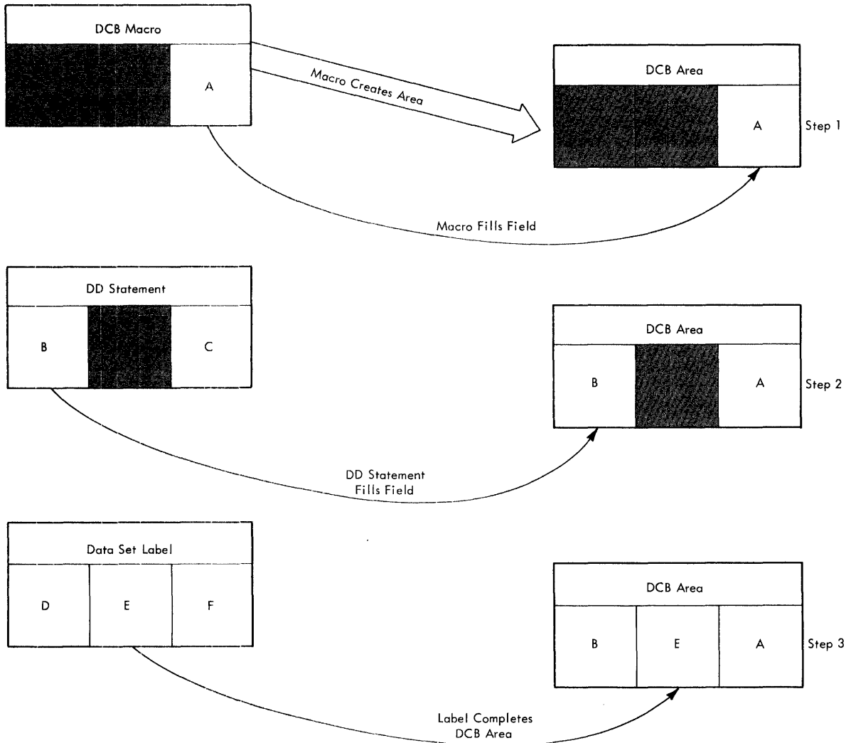
Figure 4. How the Data Control Block Is Filled
