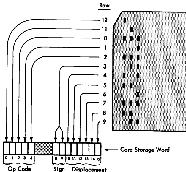
Figure 40. Load Mode Read
