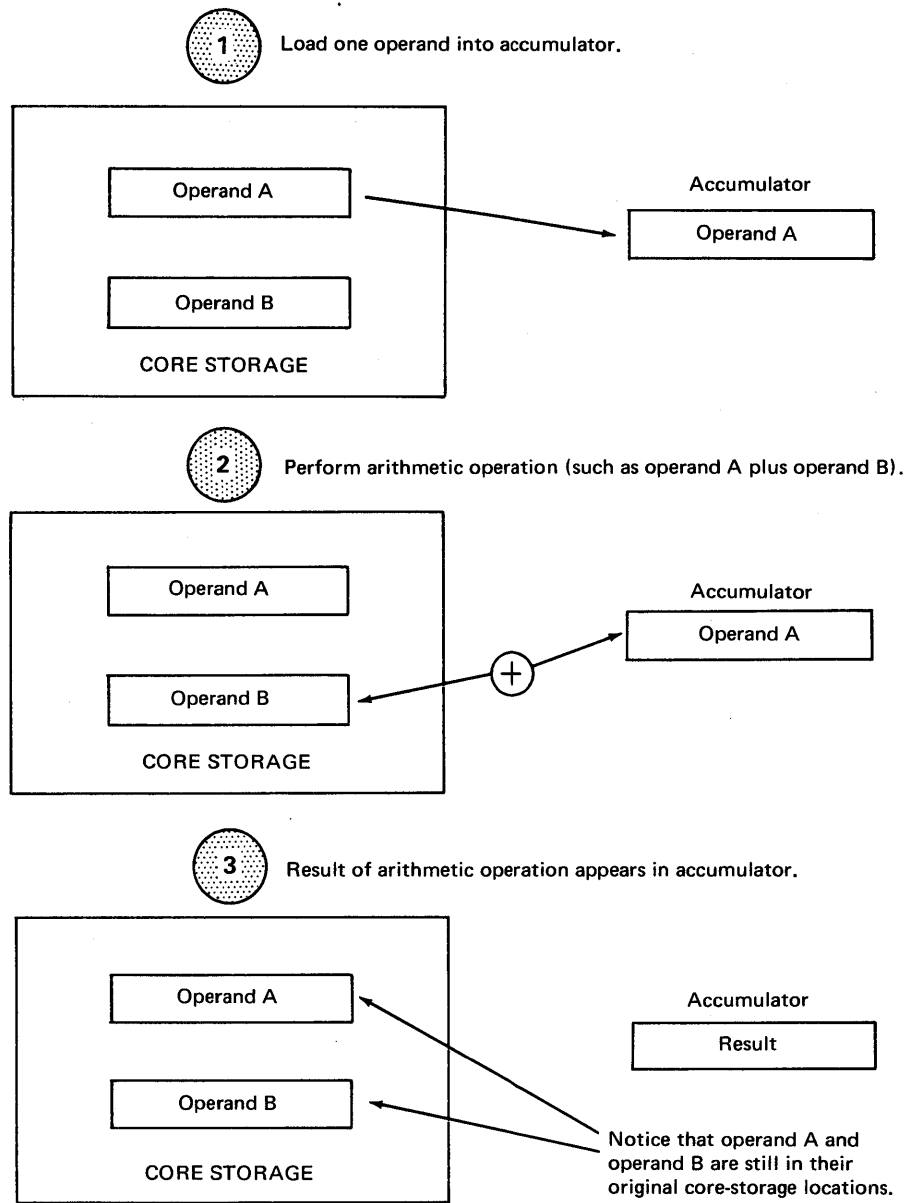
Figure 12. Use of the Accumulator in Arithmetic Operations
