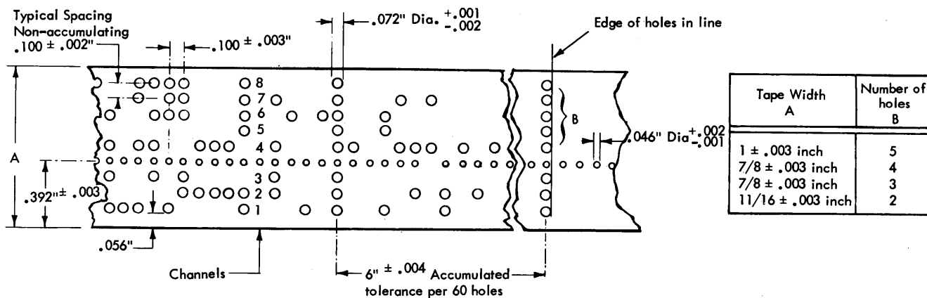
Figure 47. Tape Specifications
