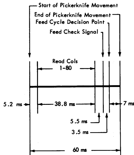
Figure 44. 2501 Timing Schematic
