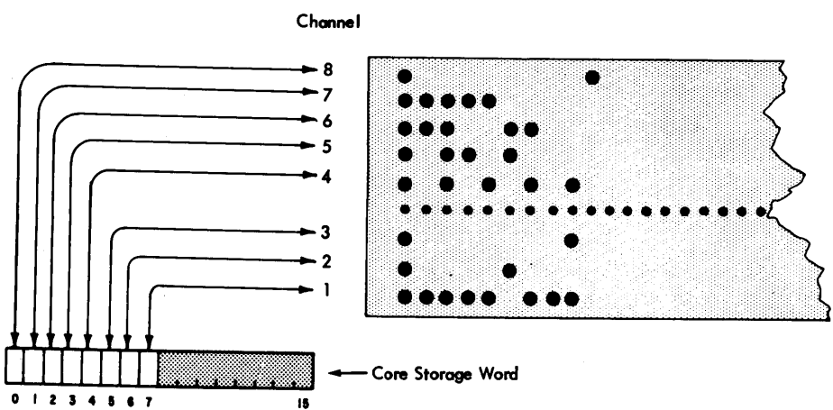
Figure 48. Paper Tape/Core Storage Format
