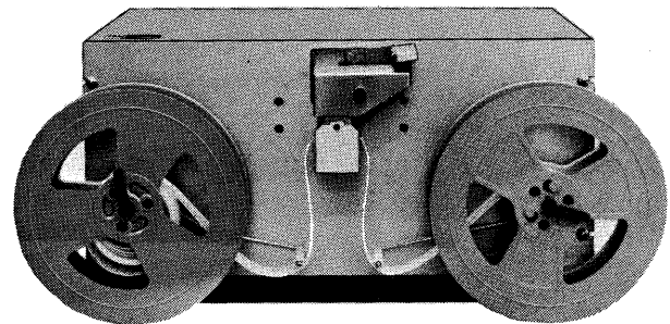
Figure 46. IBM 1134 Paper Tape Reader
