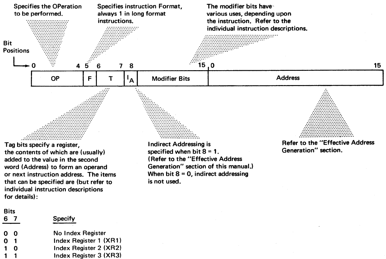
Figure 6. Long-Instruction Format
