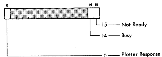
Figure 61. 1627 Device Status Word
