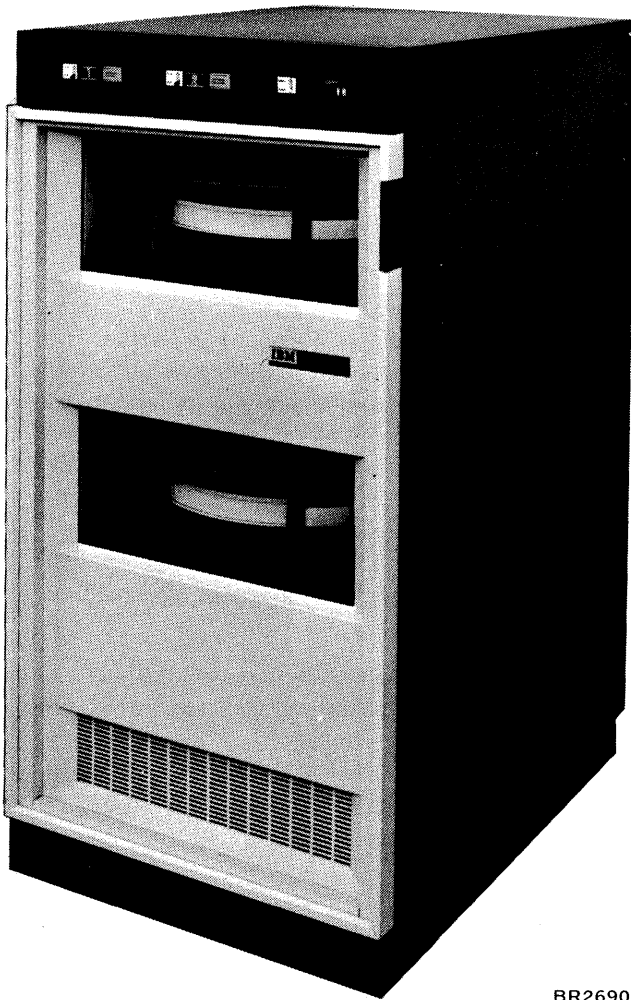
Figure 35. IBM 2310 Disk Storage Model B2
