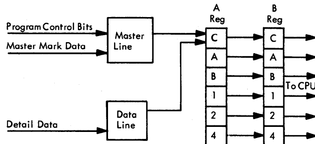
Figure 65. IBM 1231 Data Flow
