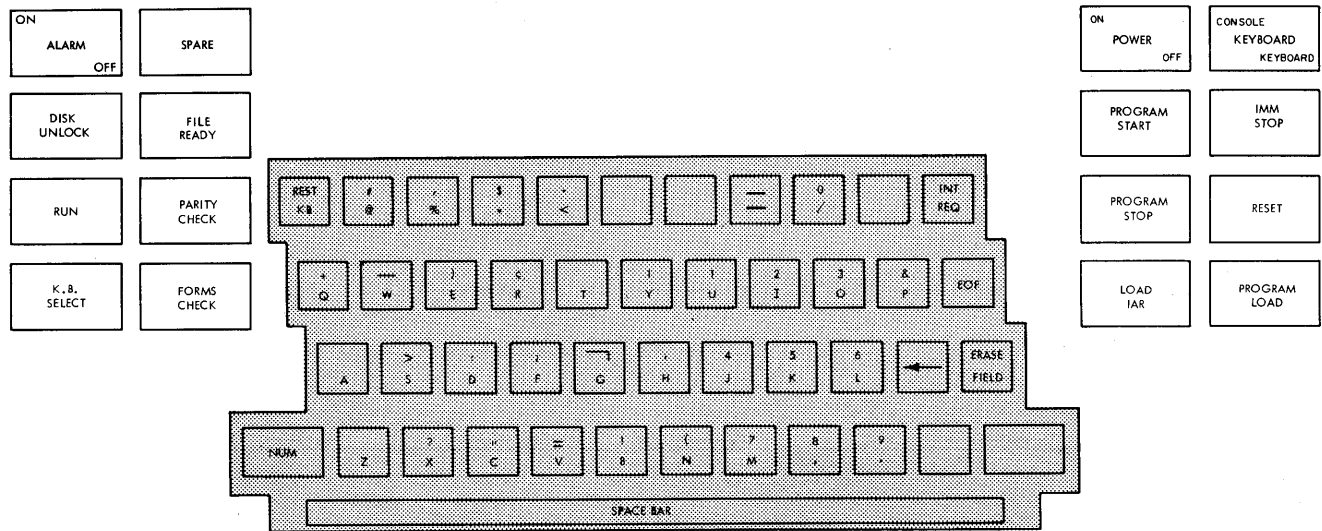
Figure 28. Console Function Lights and Switches
