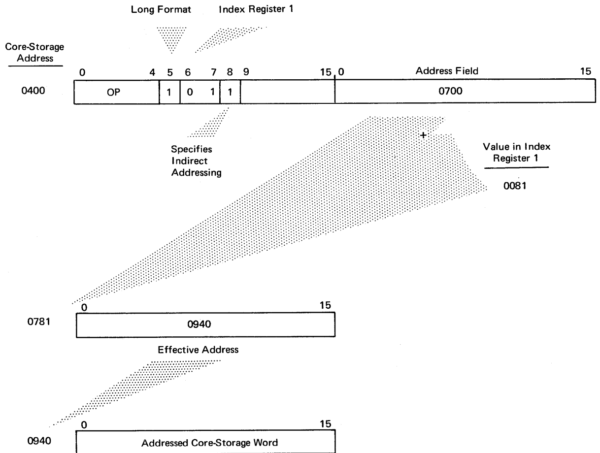
Figure 10. Indirect Addressing (Long-Format Instructions Only)
