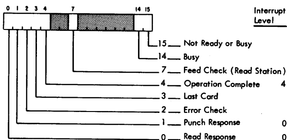
Figure 41. 1442 Device Status Word
