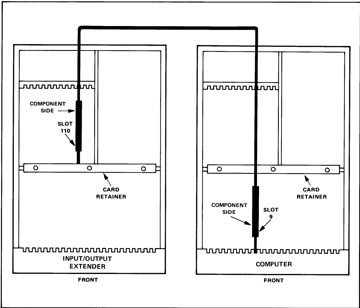
Figure 1. Installation Details
