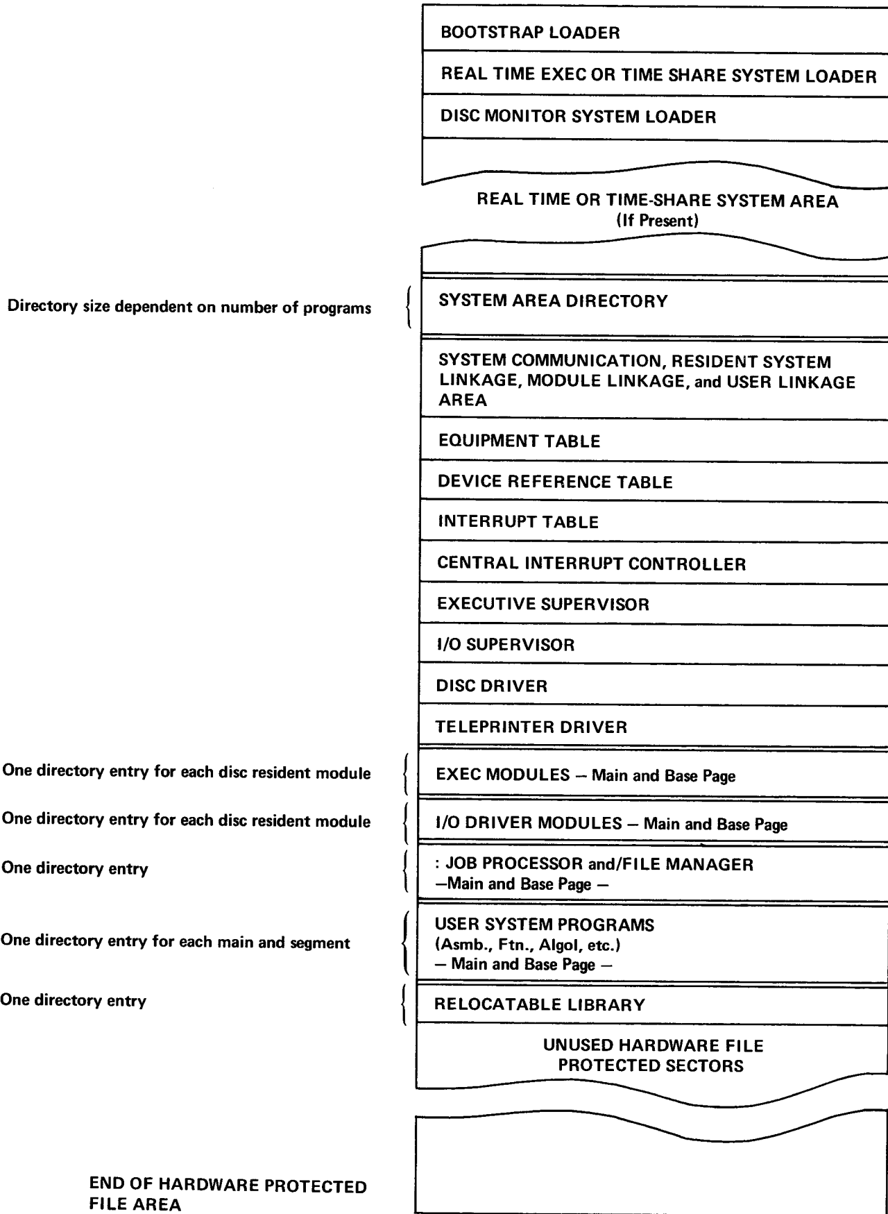
Figure A-5. Disc Allocation in System Area
