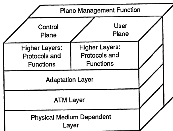
Figure 6. B-ISDN Protocol Model for ATM
