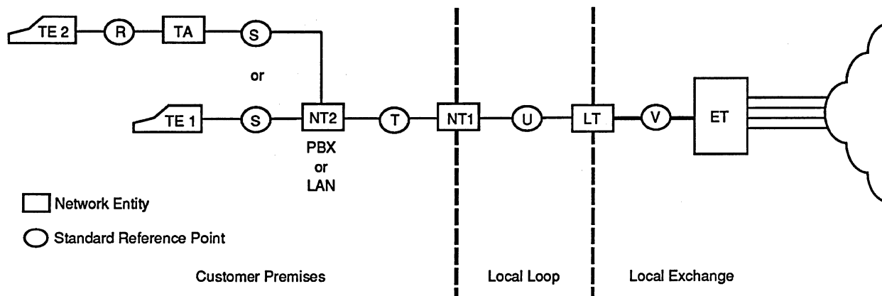
Figure 2. Schematic Overview of the ISDN User Interfaces
