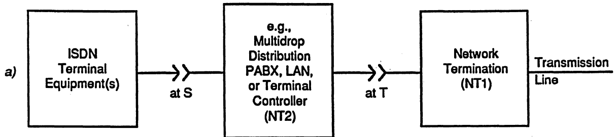
Figure 4. Sample Implementations of NT1 and NT2 Functions
