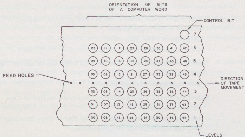
Figure 3-2. Seven-Level Punched Paper Tape (Assembly Mode)
