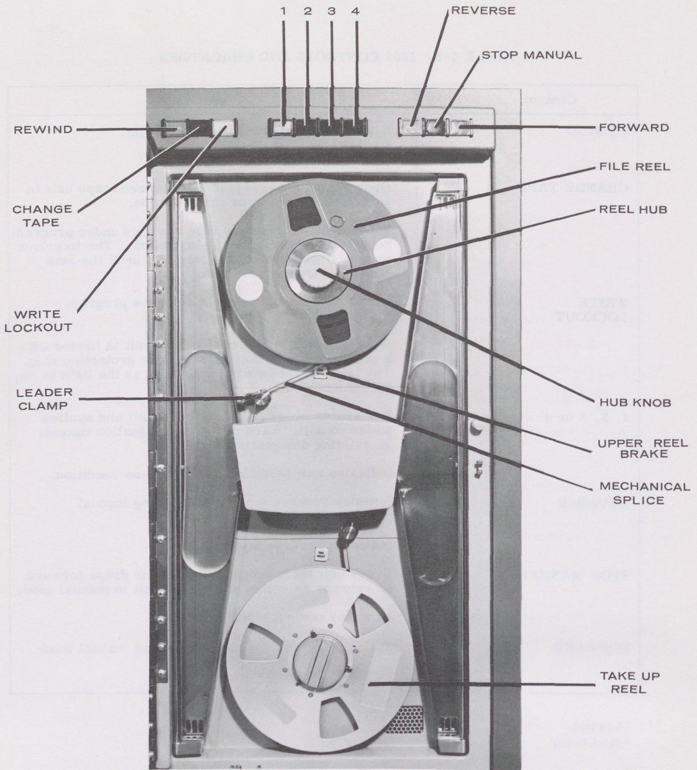
Figure 4-9. 1607 Tape Unit
