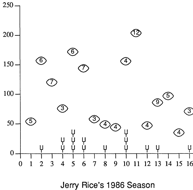
Figure 1-6. A more complicated graph
