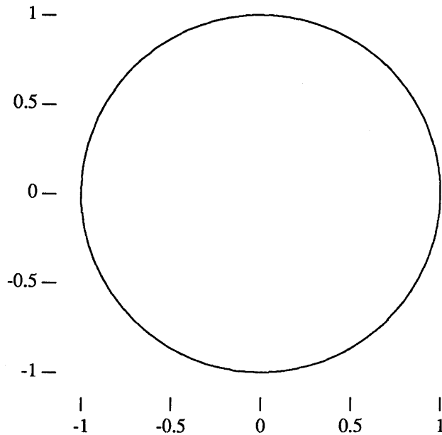
Figure 9-12. A graph circle
