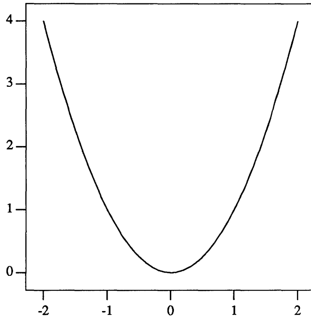
Figure 9-7. Plotting a simple curve
