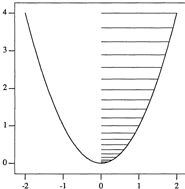
Figure 9-8. Shading part of a curve
