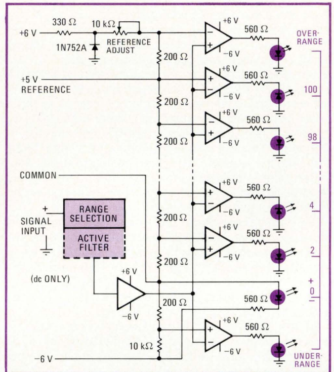
2. Diode row. For a linear display in a row-of-LEDs bar graph, the values of the reference resistors in this Simpson Electric circuit are made equal. For a logarithmic or otherwise nonlinear output, the resistors can be selected for the proper conversion.
