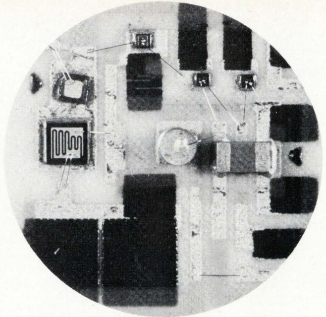
13. Hybrid heater. Thick-film resistors are used as heating elements in a 25-watt thermistor-controlled heater on a \frac{3}{4} -by- \frac{1}{2} -inch beryllia substrate. The heater, built by Integrated Microsystems Inc., is used in a solid-state oscillator manufactured by Watkins-Johnson.
