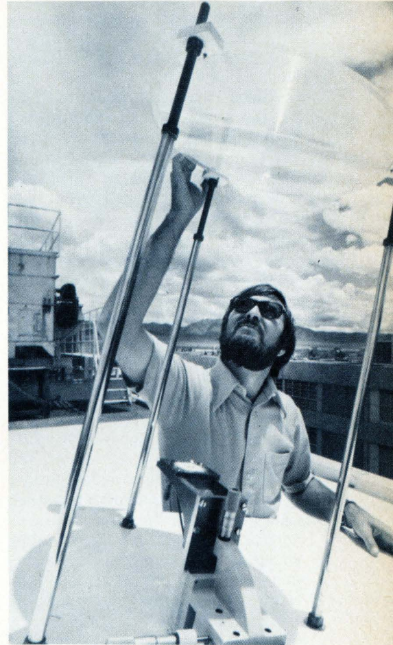
Bright outlook. Sandia Labs' approach to solar energy uses a Fresnel lens to concentrate the sun's rays on a cell. Technique is called a concentrator subsystem.
