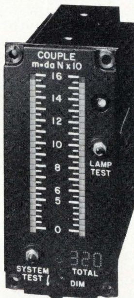
1. Glowing column. Incandescent lamps feeding light through optical fibers form a bar-graph display in this meter from Canadian Marconi. Its rugged package and bright display are designed to withstand the environment of aircraft cockpits.
