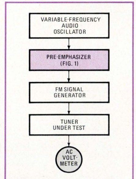
2. Flat-out testing. With pre-emphasizer that uses same frequency-selective network as tuner, this test circuit gives a flat audio output for a good tuner. The pre-emphasizer could be put between the tuner and the volt-meter, but the arrangement shown gives a better signal-to-noise ratio.
