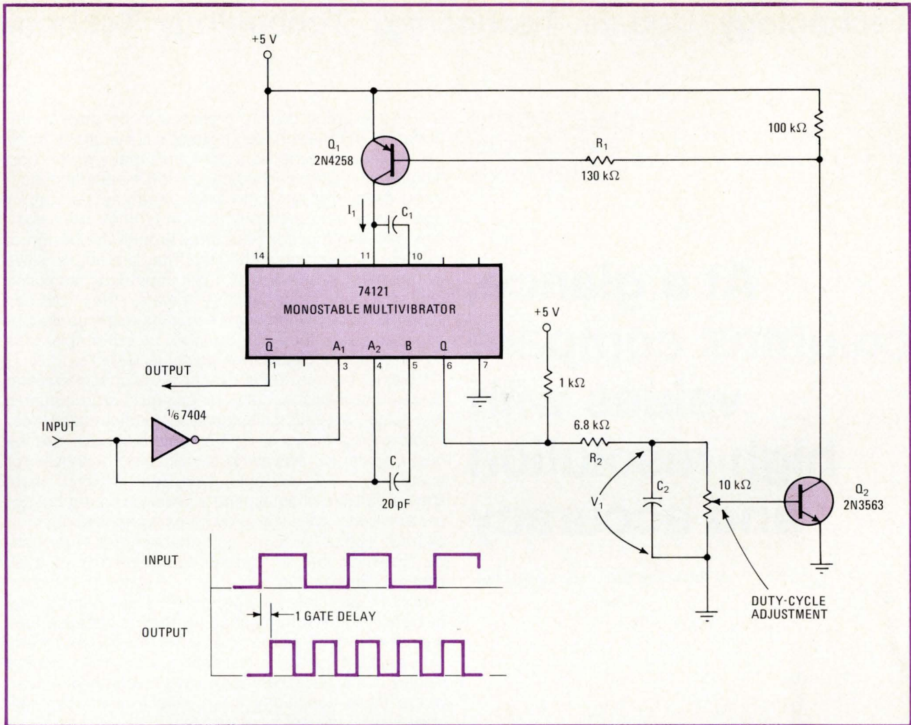
2. Constant duty cycle. Addition of feedback loop to circuit of Fig. 1 makes duty cycle of output wave independent of input frequency. Triggering of output pulses is the same as in the basic circuit, but the pulse width is automatically adjusted for the duty cycle set by the potentiometer. Here the pot setting gives a square wave at the doubled frequency. Delays of 30 or 40 ns are negligible at frequencies below 1 MHz.
