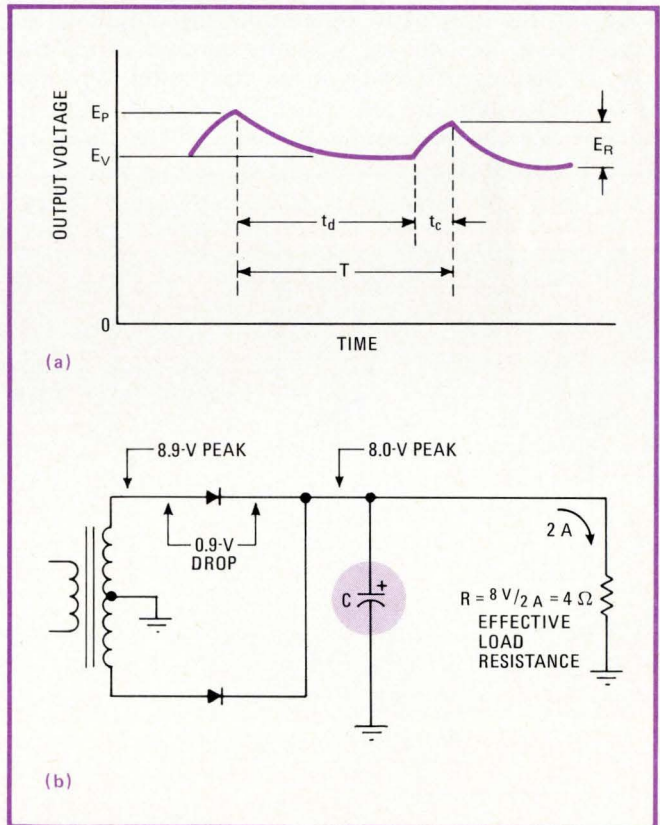
How much C? For a given amount of ripple in output of rectifier/filter power supply, the minimum value of capacitor C is closely approximated by expression E_R/E_P = T/RC . Output waveform is shown in (a), and full-wave rectifier circuit is shown in (b). Numerical values are those of example in text.
