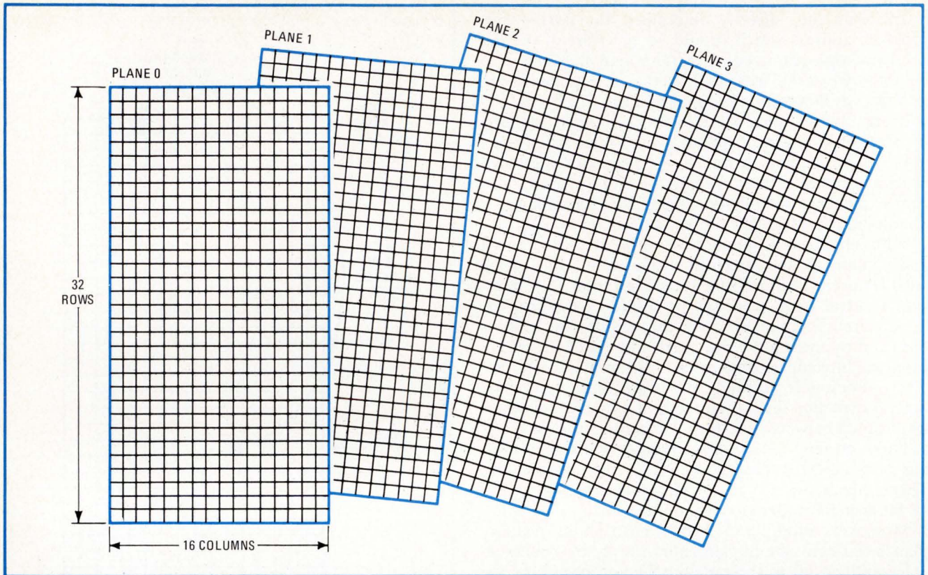
8. Multiplanar addressing. If required, multiple planes, each carrying 512 microinstructions, can be implemented without any sacrifice in the speed of the system. Moreover, jumping is possible in three address dimensions with such a configuration.
