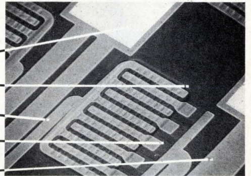
ONE OF THE 48 INDIVIDUAL CELLS ON THE 60 x 165 MIL MRF306 CHIP
