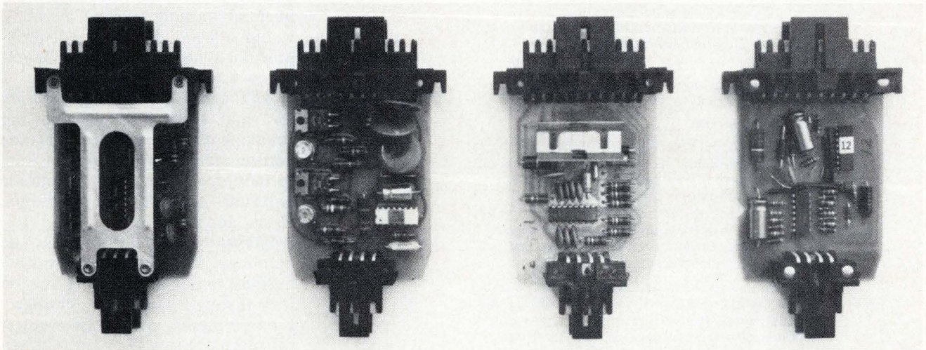
To be changed? Logic modules for GM's 1974 seatbelt interlock system would have to be redesigned if law is changed.
