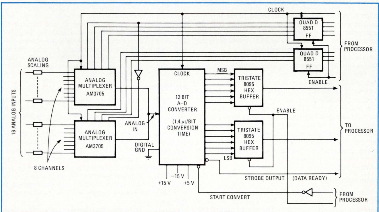
2. Input. Front end of data-acquisition system employs two analog multiplexers to handle either 16 single-ended inputs or eight differential inputs. Successive-approximation a-d converter has a maximum resolution of 12 bits. However, it can operate at reduced resolution, for increased speed, when it receives instructions to do so from the microprocessor.
