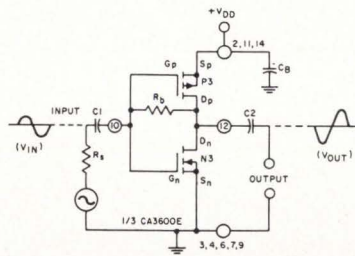
CA3600E transistor pair biased for linear-mode operation
