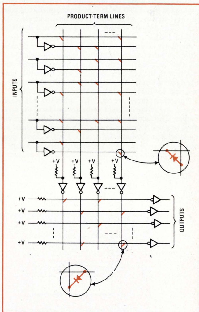
1. Programed logic array. Like a ROM, a PLA is a matrix, but addresses are programmed, as well as data. Using optional bits in an address permits two or more addresses to point to one word.
