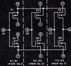
CA3600E schematic diagram
