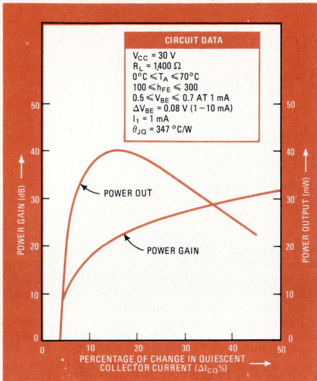
2. Trading off gain and swing. For large variations in quiescent collector current, power gain increases, but power output decreases because the output-voltage swing becomes smaller. The change in collector current should be some reasonable value like \pm 20\% .
