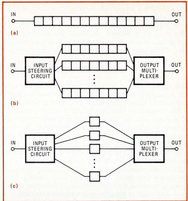
4. Signal processing variety. The simplest analog delay line (a) is a single line, where transfers are made serially from input to output. The parallel lines in (b) and (c) reduce dispersion with multiplexing techniques but require more complex structures.
