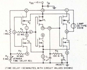
Analog timer using CA3600E
