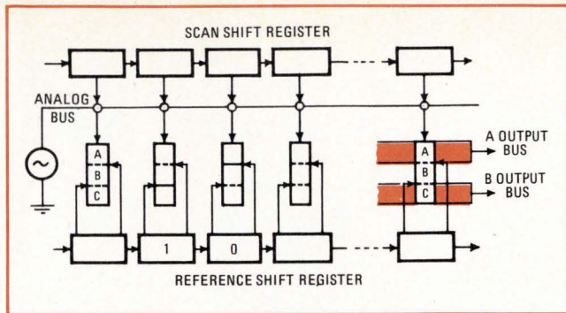
7. Sloshing charge. In GE's method of tap-weight control, charge in a pair of elements is moved back and forth so that the output signal is proportional to the total charge moved.
