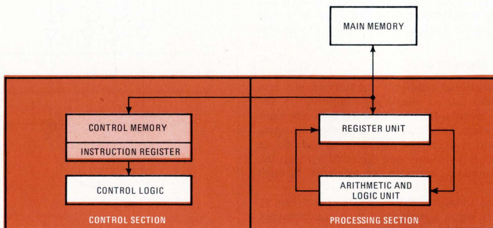
2. Microinstruction control. Basically, the operation code of an instruction in the user's program (external) is interpreted as an address specifying, in the microprogram (internal), the beginning of the routine that executes the external instruction.
