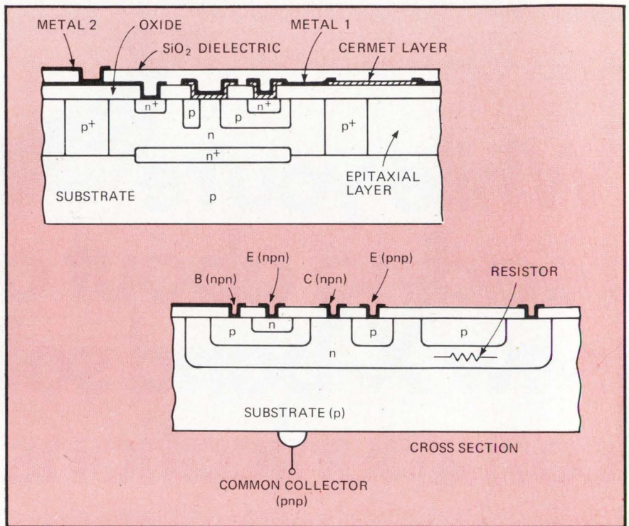
Together. Pair of LSI digital correlators from TRW. Top device is made by conventional epitaxial fabrication; bottom one by triple-diffusion method using arsenic as a collector dopant.
