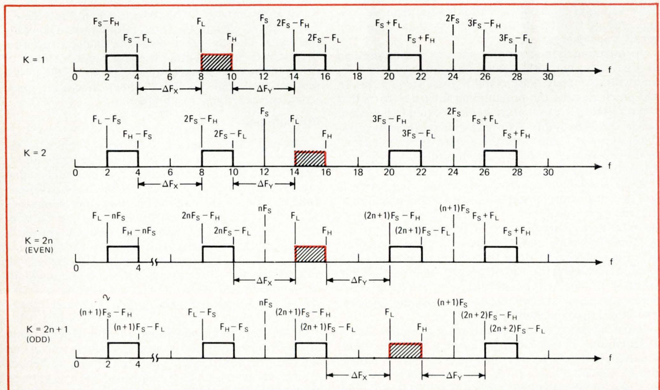
6. Edge definitions. With these spectral edge definitions of multiple spectra resulting in either odd or even values of K, the actual values of separation between neighboring spectra can be computed for both optimum and non-optimum sampling frequencies.
