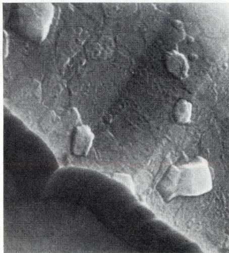
6000 X magnification shows excellent metal coverage over an oxide step, eliminating intermittent opens, thereby enhancing reliability. The scanning electron microscope has become a major tool in RCA's diagnostic and high-reliability procedures.
