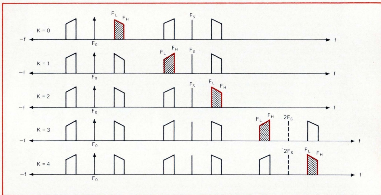
5. Spectral density. The sampling frequency depends on the width of the passband, shown here as the same for five different cases. Computation of the actual sampling frequency for a given case depends on the spectral density, K , the number of spectra below the original band.
