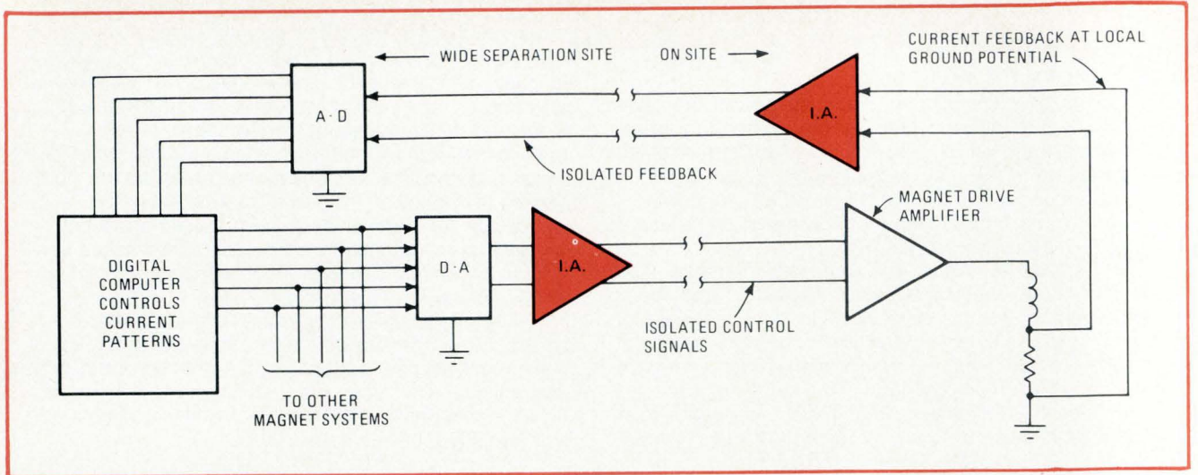
3. Ground separation. Isolation amplifiers keep analog and digital signals separated in this digitally controlled magnet system.
