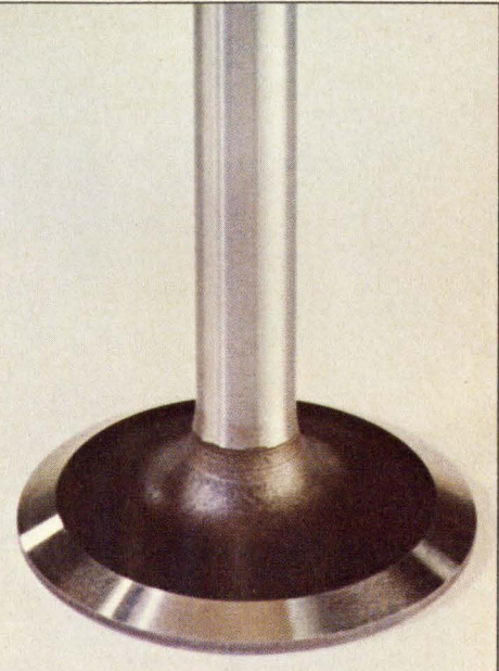
Checking surface geometry of valve section to ensure proper seating.
