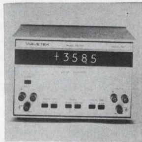
Precision digital phase meter model 750 features stable, long-term phase measurements. Frequency is 10 Hz to 1 MHz. Impedance is 1 megohm shunted by 30 pF. Recorder output is 0 to +3.6 V for 0° to 360°. Input voltage is 1 mV to 300 V rms. Resolution is 0.1°. Accuracy is ±0.1% full scale. Price is $1,500. Wavetek, P.O. Box 651, San Diego, Calif. [362]
