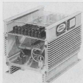
Servo amplifier AD-7200 is the heart of remote closed loop position control. It operates from either a 12 or 24 v d-c battery and positions fractional h-p permanent magnet motors. A typical application is positioning of directional control valves on cranes, tractors and other heavy mobile equipment. Price is $165. Jordan Controls Inc., 5607 W. Douglas Ave., Milwaukee, Wis. [386]
