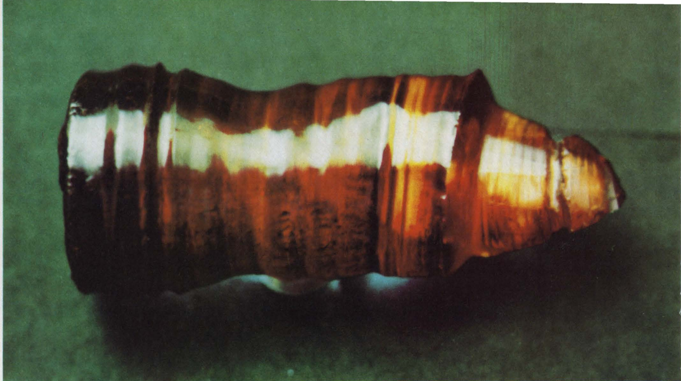
Growth plan. This crystal of bismuth germanium oxide was grown by the Czochralski pulling technique. Crystals 6 inches and longer are becoming available that will provide delays of 100 microseconds.
