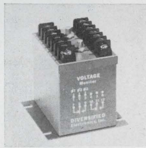
Three-phase voltage band monitors series PB protect electrical and electronic equipment required to operate between 2 voltage limits. Each of the 3 phases is monitored for an under or over voltage limit. The monitor can be used to sound an alarm, light warning lights, shut down or remove equipment from the line. Diversified Electronics Inc., Box 6231, Evansville, Ind. [383]
