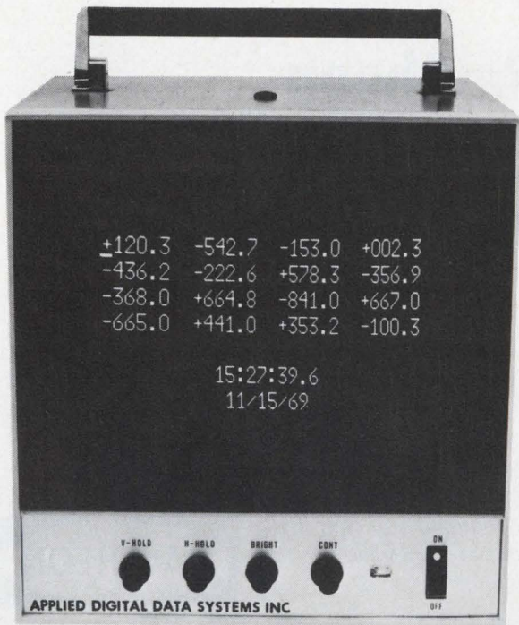
New CRT readout—low cost, high flexibility.
