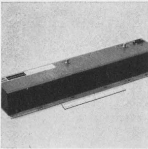
Microwave amplifier WJ-1115, covering 7 to 11 Ghz, is for use in airborne ecm or data link systems. It features integral power supply and provides 3 w power output, 45 db small signal gain and 22 db maximum noise figure in X-band. Unit weighs less than 6 lbs and comes in a package 2.3 x 3 x 16 in. Watkins-Johnson Co., Stanford Industrial Park, Palo Alto, Calif. [401]
