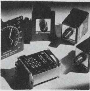
On/off temperature controllers series 9317 may be actuated by thermocouples or resistance temperature detectors. They contain solid state circuits in conjunction with a relay output. The output relay de-energizes when the setpoint temperature is reached and energizes after temperature falls below the setpoint. Sigma Instruments Inc., 170 Pearl St., Braintree, Mass. [381]
