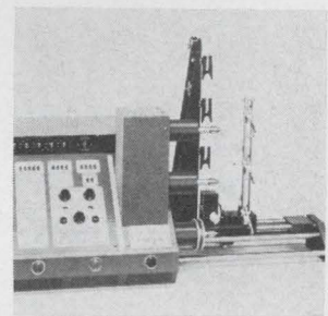
Automatic coil winder type 3S utilizes 3 spindles to triple high production output of precision coils. It can be programmed by IBM card or set up by switches from a data sheet, for winding at speeds to 8,000 tpm to precise tolerances. Unit handles coils up to 8 in. long and 5 in. o-d, and wire sizes from 16 to 50 Awg. Eubanks Engineering Co., Monrovia, Calif. [424]
