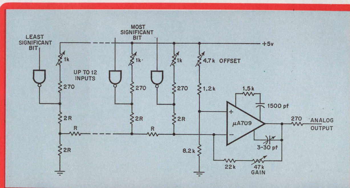
Weighted. A resistive ladder network weights the currents switched by the logic gates according to the significance of their input bits on the binary scale. The ladder network supplies the operational amplifier with a current proportional to the value of the digital input.
