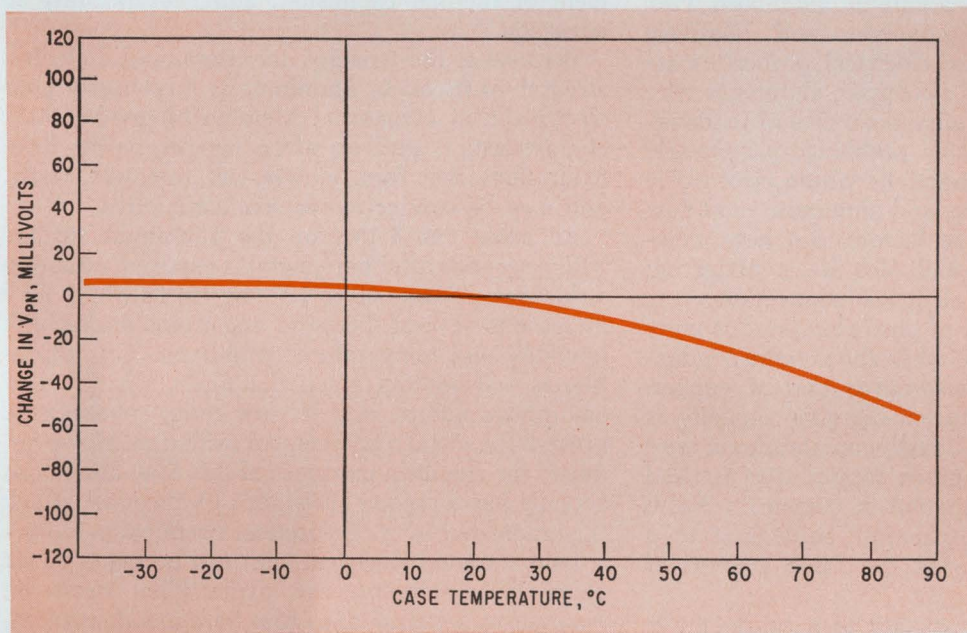
Temperature effect. Compensation keeps thermal coefficient to 40 parts per million per °C, so stabilized voltage varies only a few millivolts from one temperature extreme to the other.
