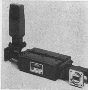
Four-part, differential-phase-shift circulator H62DA1 is for use as a duplexer or isolator in the frequency range of 15 to 17.5 Ghz. The unit can handle up to 1 kw of average power and up to 10 kw of peak power with a load vswr of 2:1. Cooling of the 4-lb circulator is through natural air convection. Varian Microwave Components Operation, 611 Hansen Way, Palo Alto, Calif. [406]
