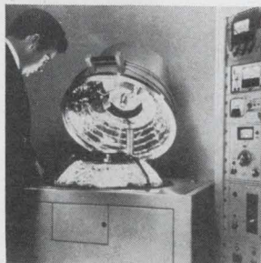
Vacuum coating system NRC 3111 is for high volume, high capacity, thin film deposition production. Tailored to meet the needs of IC makers, it employs the VHS-6 diffusion pump, rated at 2,400 liters/sec, and contains planetary tooling for high deposition rates from multiple resistance evaporation sources or an electron beam source. Norton Co., Charlemont St., Newton, Mass. [426]
