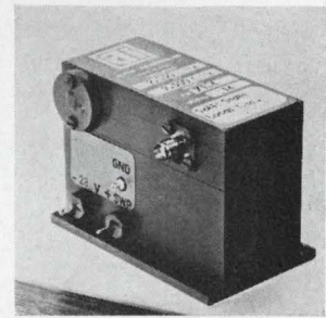
Voltage-tuned oscillator model PM7152 is for application as a local oscillator in X-band exhibiting a frequency stability vs temperature of \pm 0.2\% . Specifications include: frequency range, 9.35-9.50 Ghz; tuning voltage, +2 to +30 v; output c-w power (min/max), 10/30 mw; output power flatness, \pm 1.5 db. Alpha Industries Inc., 381 Elliot St., Newton Upper Falls, Mass. 02164 [404]
