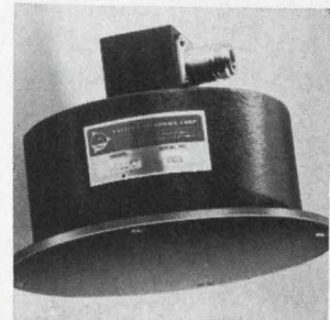
Cavity-backed Archimedes spiral antennas are broadband units that are circularly polarized with essentially constant impedance and radiation characteristics. Model S6510 illustrated operates over the 2 to 11 Ghz range. Nominal performance characteristics are: gain, 5 db; vswr, 2:1; axial ratio, 2 db; and beamwidth, 75^\circ . Eastern Microwave Corp., 139 Swanston St., Winchester, Mass. [408]
