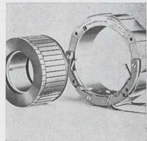
D-c torque motor series 235-100 features a thin, pancake-shaped wrap-around rotor which can be applied directly to, or around, shafts or hubs. Developed for control of rocket motor thrust vectoring systems, the motor can be used wherever precision high-torque positioning and speed control are requisites. Magnadyne Inc., 5580 El Camino Real, Carlsbad, Calif. 92008 [388]
