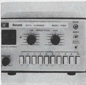
Four-pole, 10-channel reed switch matrix-data scanner 508A is suited equally to low-level guarded multiplexing of 3 or 4 analog signals and to 4-line-per-digit data transfer, commutation or steering. Its reed relays may be energized to connect a set of 4 input terminals to a corresponding set of 4 output terminals. Monsanto Electronic Instruments, W. Caldwell, N.J. [361]
