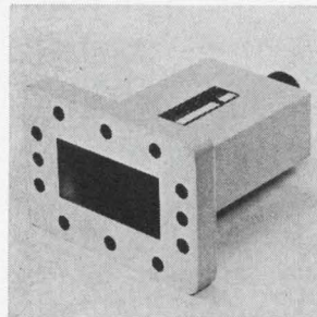
Waveguide-to-coaxial adapters WR229 feature an end launch configuration and provide extremely low vswr of 1.10 max. over the communication satellite band of 3.7 to 4.2 Ghz. They can be obtained with either precision N connectors (male or female) or the new high precision APC 7, 7 mm connector. Maury Microwave Corp., 8610 Helms Ave., Cucamonga, Calif. 91730 [407]
