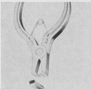
DIP extractor plier 4916 removes all 14-16-24- and 36-lead dual in line packages. It withdraws the IC straight up out of the board without bending leads, will not lift socket pads or pop up into operator's face. Metal teeth for durability and self-closing metal construction combine to provide a tool for fast DIP removal. Techni-Tool Inc., 1216 Arch St., Philadelphia. [425]
