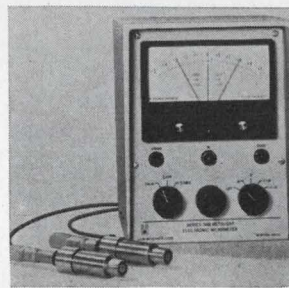
Electronic micrometer series 300 is capable of non-contact measurement of objects with a resolution of 0.000010 in. The objects being measured may be either stationary or moving. Meter readout as well as ±5 V analog output is available. Unit is designed to provide a continuous 100% inspection of production pieces. Lion Research Corp., 60 Bridge St., Newton, Mass. 02195 [363]
