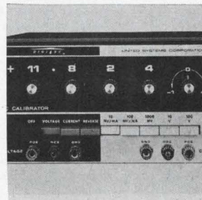
Precision calibrator model 311 offers 0.01% accuracy in both voltage and current. Five voltage and two current ranges are available and afford complete instrument calibration facilities. Current resolution is µA and voltage resolution is 1 µV. Rated load is 100 mA, which allows for use as a lab power source. United Systems Corp., 918 Woodley Rd., Dayton, Ohio 45403 [367]
