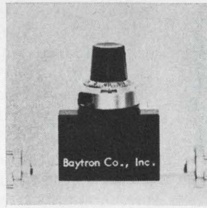
Dial calibrated variable phase shifter features a precision ball bearing mechanism with a differential drive counter that assures accuracy and reliability with fine readout definition. Model 3E-13 (60-90 Ghz) features calibration accuracy to \pm 3^\circ at any desired frequency. Vswr is rated at 1.20 max, with minimum phase shift of 180^\circ . Baytron Co., Medford, Mass. [403]
