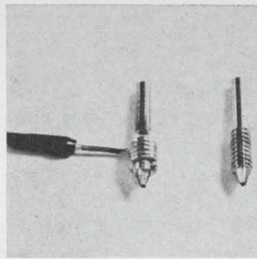
Beam lead bonding tools come in any size or style for any chip application and in any desired quantity. Users have a choice of materials, including carbide, tungsten or Inconel alloys. Tools can be supplied for either wobble tool or self-aligning tool application and can be specified with heater soldered on or separate and replaceable. Micro-Swiss Inc., Cherry Hill, N.J. [423]
