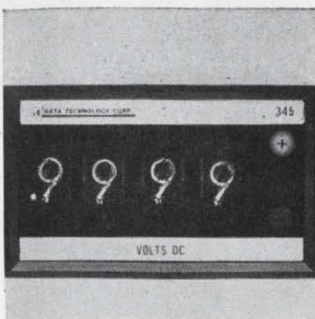
Four-digit panel meter model 345 is a highly accurate (0.03%) unit for measuring d-c volts from 100 \mu v to 1,000 v in any one of four d-c ranges. In addition to this capability, automatic polarity and overrange indication are standard. Unit price is $295, and is $225 in 100-lot quantities. Data Technology Corp., 1050 E. Meadow Circle, Palo Alto, Calif. 94303 [3611]
