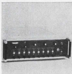
Noise-loading test set 330A measures effects of intermodulation noise products on the performance of multichannel communications networks. It can be used on multiplex networks having from 12 to 2,700 active channels. Model 330A consists of a white noise generator (330A-G), a receiver (330A-R) and appropriate filters. Philco-Ford Corp., Newport Beach, Calif. [3661]
