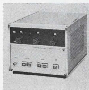
Audio-range noise generator model 8057A synthesizes noise with a stable output level, a level so predictable (within 0.2 db at full amplitude) that amplitude accuracy is determined primarily by the instrument's wide-range output attenuator, which is accurate within \pm 0.5 db. Price is $775; delivery, from stock. Hewlett-Packard Co., 1501 Page Mill Road, Palo Alto, Calif. [3671]
