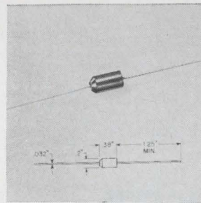
Silicon rectifiers in the BH series are offered up to 5 kv piv, 250 ma in the 0.2 in. diameter x 0.38 in. long DO-27 package. Suited for p-c board mounting, they can be used in twt amplifiers, lasers, radio transmitters, screen supplies, electronic ignition, Xenon flash power supplies, and similar h-f applications. Electronic Devices Inc., 21 Gray Oaks Ave., Yonkers, N.Y. [438]
