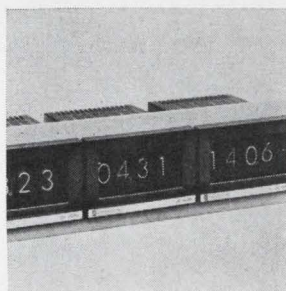
Digital panel meter X-MOD/DPM is a 3-digit and sign integrating digital unit with 100% over-range. It features automatic polarity indication and accuracy of 0.1% \pm 1 digit. Unit is provided with one fixed full scale in either d-c voltage ranges from 1.999 mv to 1,999 v on d-c ranges from 19.99 \mu a to 199.9 ma. Preston Scientific Inc., 805 E. Cerritos, Anaheim, Calif. [3621]
