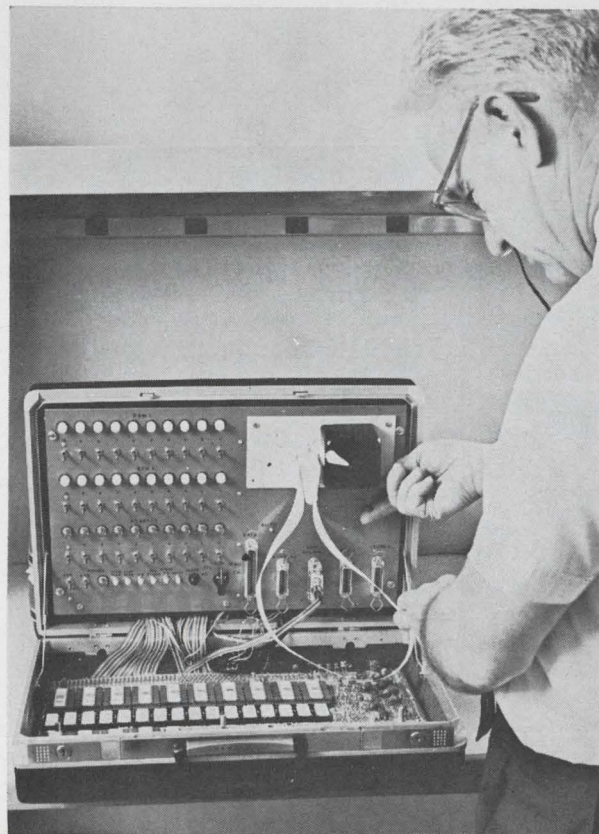
Good case. Read-only memory simulator in attache case enables users to alter bit pattern quickly before deciding on final design of memory.
