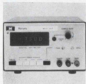
Integrating d-c digital voltmeter model 200A features 7-segment light-emitting solid state numeric readout. It measures d-c voltages to 1,000 v in 4 ranges with resolutions of 100 \mu v (0 to \pm 1.999 v d-c), 1 mv (0 to \pm 11.999 v d-c), 10 mv (0 to \pm 119.99 v d-c) and 100 mv (0 to \pm 1,000 v. a-c). Monsanto Co., Passaic Ave., W. Caldwell, N.J. [3681]
