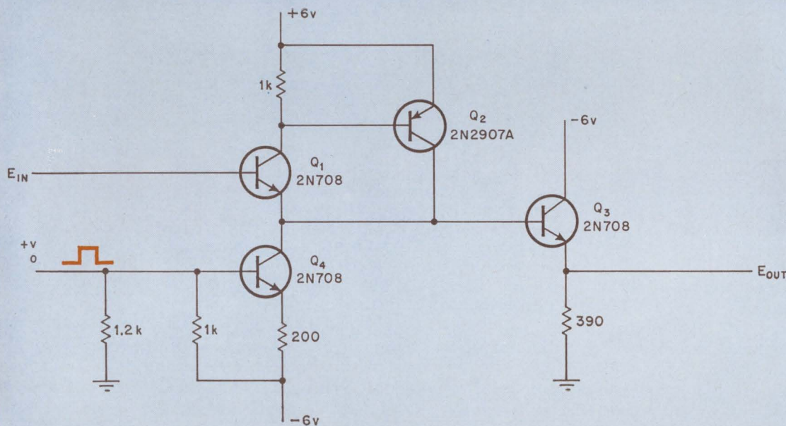
Buffer. This unity-gain buffer amplifier employs heavy degenerative feedback to get a high input impedance. Q_1 and Q_2 are connected in a complementary arrangement and effectively cancel any d-c offset at the amplifier's input. The gated d-c level remains stable within 0.1 db from -30^{\circ}\text{F} to +160^{\circ}\text{F} .
