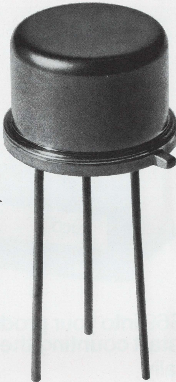
Companion types: RCA-TA7408 & TA7409 (actual size)
