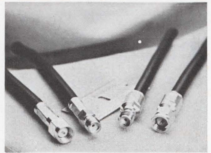
Links. Connectors for RG-58 and RG-223 cables have crimp plug and jack, left; clamp plug and jack, right.
