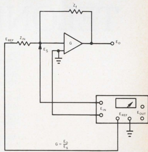
OP AMP OPEN-LOOP GAIN MEASUREMENTS WITH LOCK-IN AMPLIFIER.
