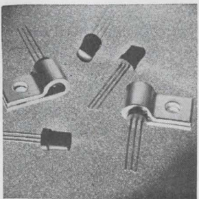
General purpose pnp and npn complementary transistors (D29E and D33D families) are available with or without heat sink in the TO-98 package. They are available with 25, 40 and 60 v breakdown ratings. The devices offer a power dissipation rating of 500 mw at 25^{\circ} C. Units are priced at 29 cents for pnp and 27 cents for npn in 10,000 lots. General Electric Co., Schenectady, N.Y. [440]
