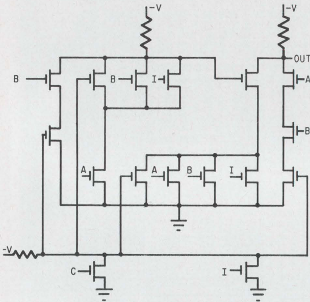
Iffy inverter. Conditional complementing circuit inverts the accumulator output if the input register and the carry bits are different and if the inhibit signal is off.
