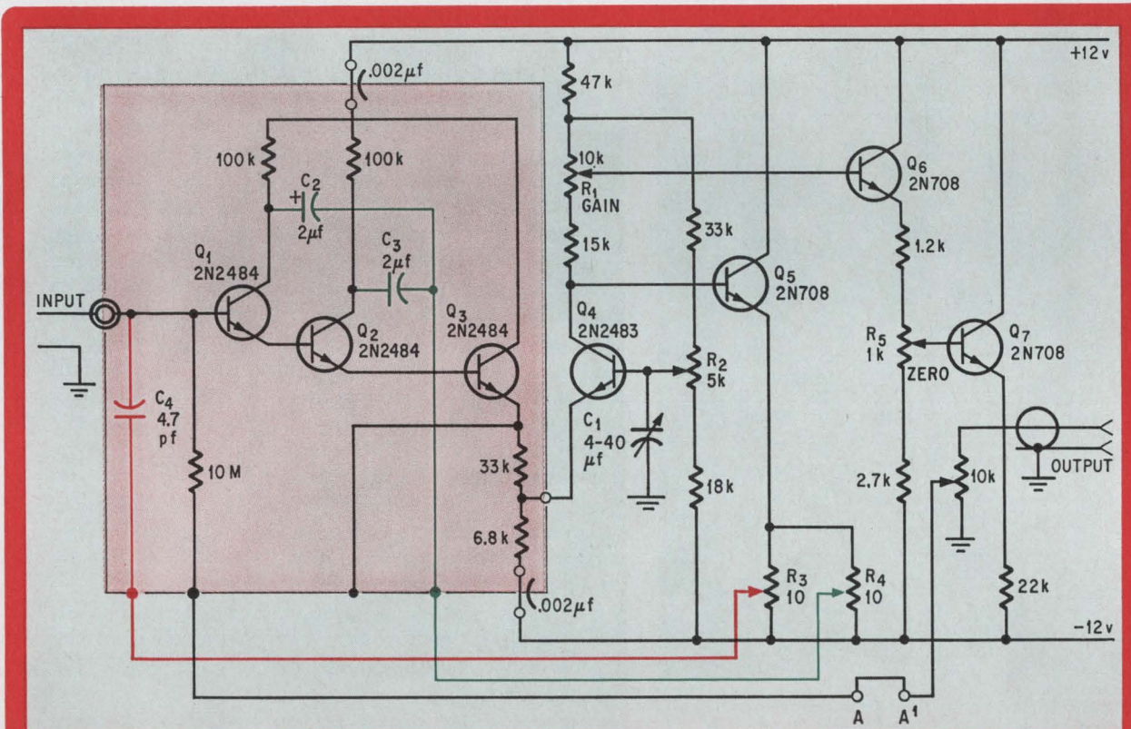
Probe circuit. Transistors Q_1 , Q_2 and Q_3 form a negative-capacitance impedance converter that is followed by d-c amplifier Q_4 and output emitter followers Q_5 and Q_7 . Zero input capacitance and high input resistance are assured by controlling R_3 , R_4 and C_1 .
