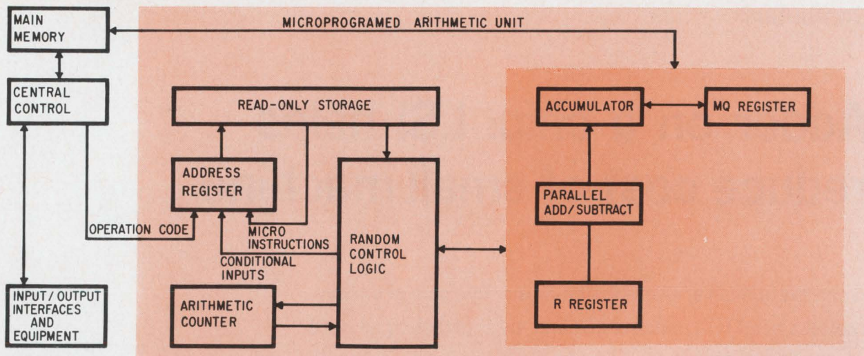
Typical small computer. Its design requires only a monolithic arithmetic unit (dark tint), monolithic read-only memory (light tint), small amount of random control logic, and conventional input/output and memory hardware.
