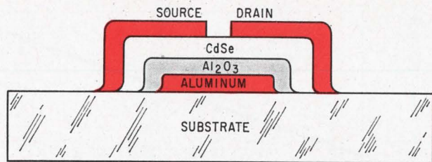
Inverted. With the gate deposited first, the aluminum oxide insulator can be formed directly on the gate lead.
