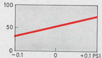
Pulse-width modulation. A variable pulse-modulated output results for a varying applied differential pressure. Input/output characteristics are linear for applied pressure.
