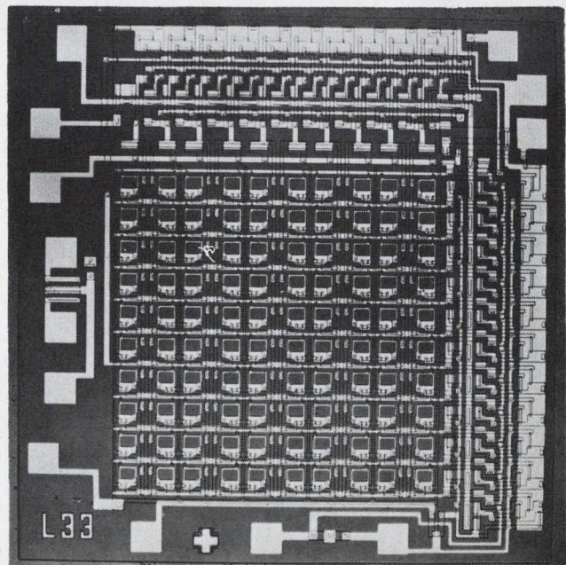
First reader. Plessey has readied for production this 10-by-10 MOS array of photodiodes, amplifiers, and scanning circuits on a single chip. Most likely first application: character readers.
