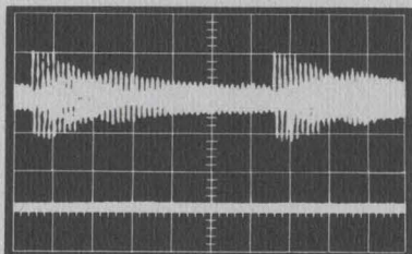
Fig. 4. Sylvania Schottky diodes exhibit much lower microphonics than point-contact diodes. Upper trace is microphonic response of a point-contact diode when subjected to a mild shock; lower trace shows the lack of microphonic response of a Sylvania Schottky D5754 when subjected to the same shock.
