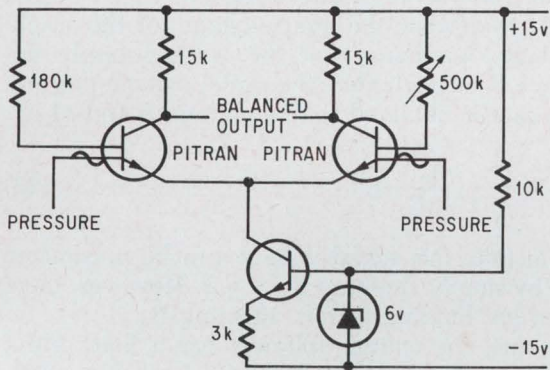
Differential amplifier. Differences between two applied pressures appears as output. High input impedance results from a constant current source.
