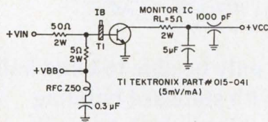
(SATURATED SWITCHING TEST CIRCUIT DIAGRAM FOR B-148000 & B-155000)
