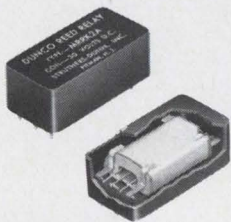
Cutaway view
