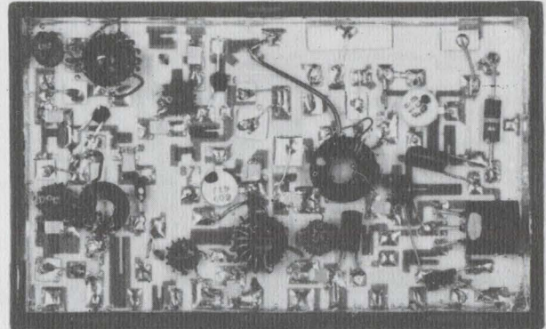
UHF Transmitter
