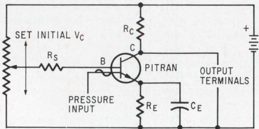
Wide temperature. Adding an emitter resistor R_E enables circuit to operate over wide temperature range. Capacitor, C_E , shunts R_E assuring the gain for a-c operation to be the same as for the d-c bias circuit.
