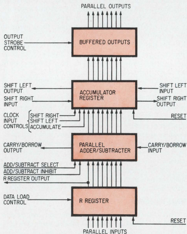
Four-in-one. Monolithic arithmetic unit comprises input register, adder-subtractor, accumulator, and output buffer, all for eight bits in parallel, plus connections to outside world or similar adjacent units.
