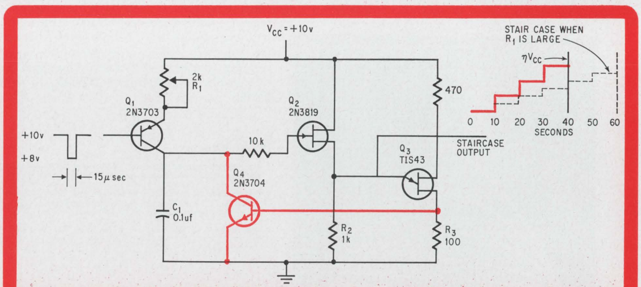
Pulse counter. Each pulse raises the voltage on capacitor C_1 in equal increments until it triggers the UJT into conduction. The voltage that appears across R_3 signals the summation of pulses and makes Q_4 discharge capacitor C_1 .
