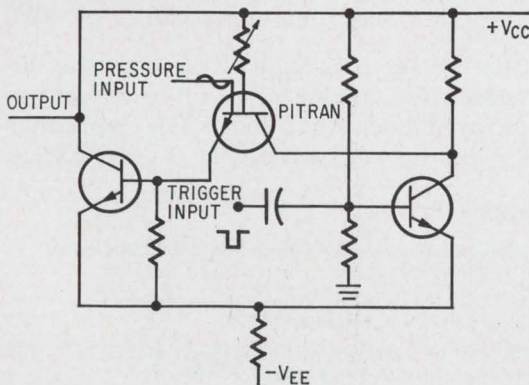
Pulse-width modulation. A variable pulse-modulated output results for a varying applied differential pressure. Input/output characteristics are linear for applied pressure.
