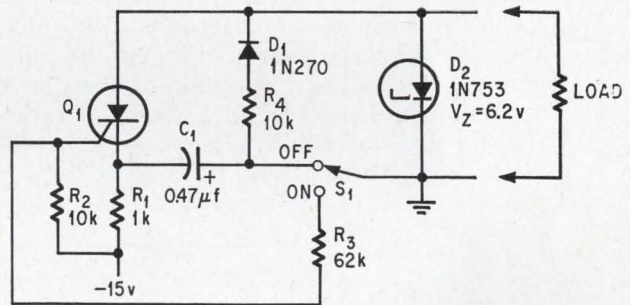
Tandem switch. Silicon controlled rectifier turns on and off with switch positions, but not with contact bounce.
