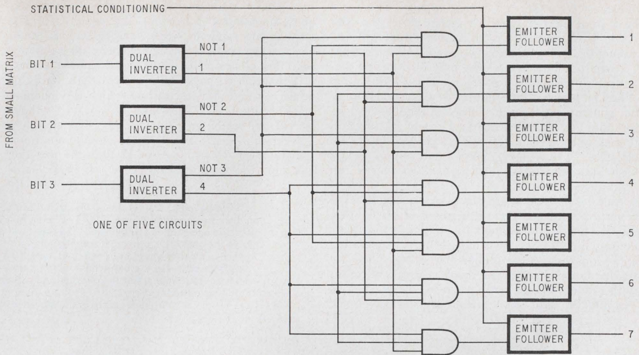
Decoder for expansion. The binary number in each row of the small matrix is decoded to set an individual flip-flop in the corresponding row of the expanded matrix. Statistical conditioning blocks some outputs at random.
