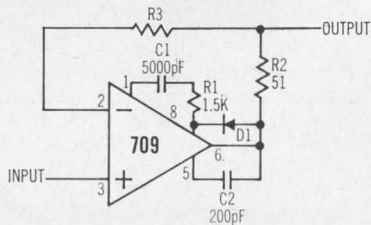
Voltage Follower
