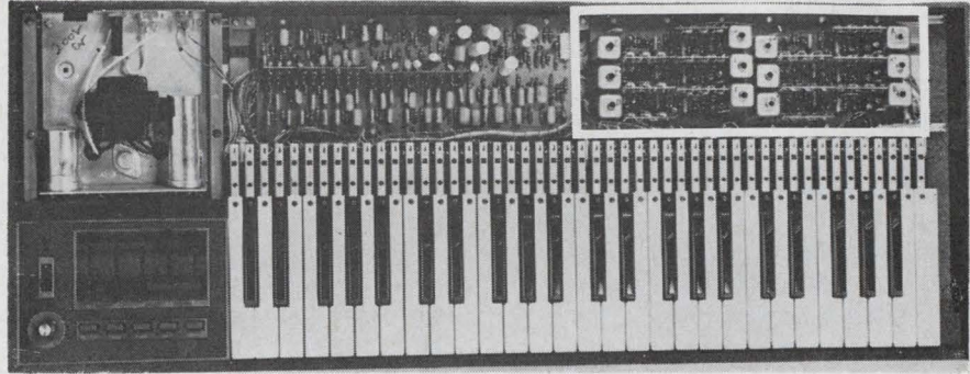
IC tone generators. Heart of lightweight organ is printed circuit board, upper right, which mounts 36 digital integrated circuits.
