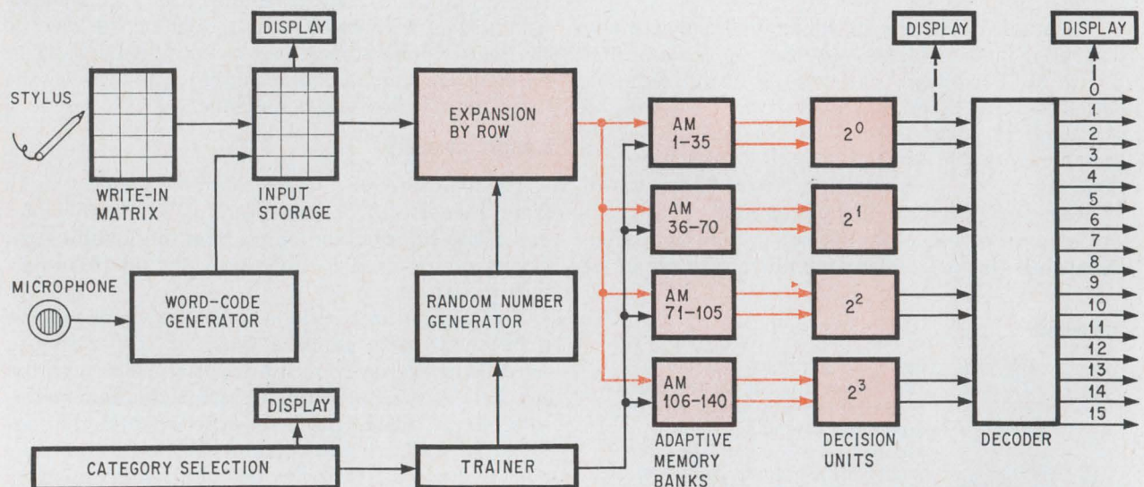
Graphics and voice. Both kinds of input set up patterns in the 3-by-5 input storage, which is expanded into a 7-by-5 matrix row by row. The expanded pattern gates weighted sums from the corresponding adaptive memory units to the decision units, which produce a binary output if they recognize the pattern.
