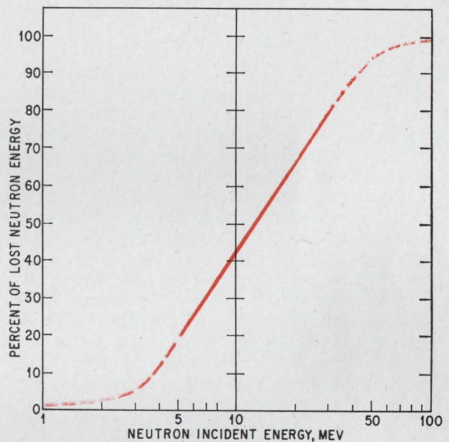
Silicon vs neutrons. Some of the energy lost by neutrons in silicon acts as ionizing radiation. The percentage of energy causing ionization increases with the incident energy of the neutrons.
