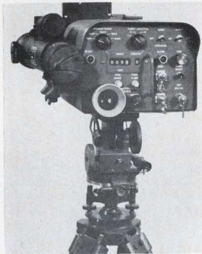
Eyes. Two-laser device for ranging, communications, intrusion alarm.
