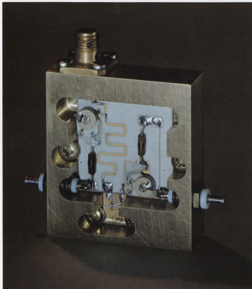
High powered. A hybrid 500-MHz oscillator built by Motorola produces a 2-watt power output. The device is mounted in a brass test fixture.
