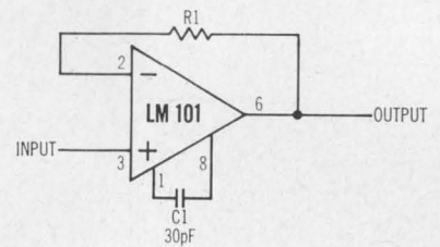
Voltage Follower
