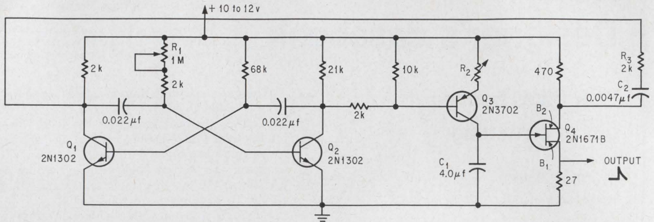
Timing circuit. Multivibrator Q 1 -Q 2 drives Q 3 until C 1 charges up V p and trips Q 4 generating a triggering pulse.
