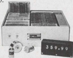
Figure 3. Model 5450 Automatic Angle Position Indicator. It measures shaft angles, converts them to digital data.
