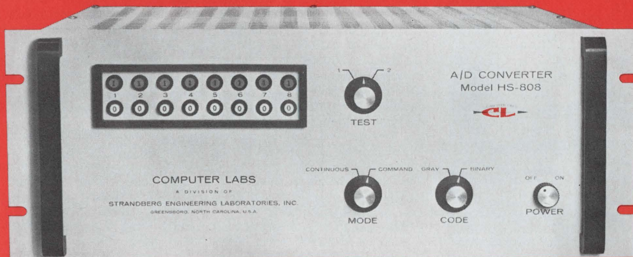
HS-808 A/D Converter 8-bit Conversion at 8 MHz
