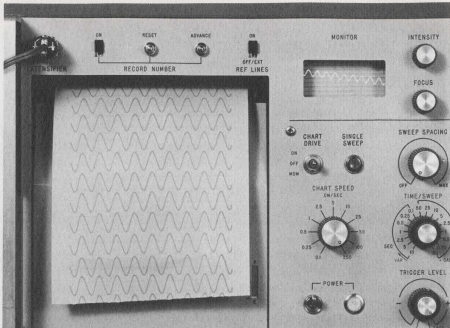
Honeywell Model 1806 CRT Visicorder
