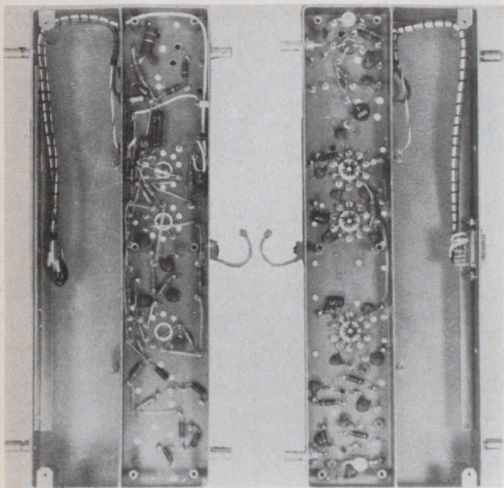
Package. The commercial version of the amplifier has the three integrated circuits in the center and the discrete transistor stages above and below.
