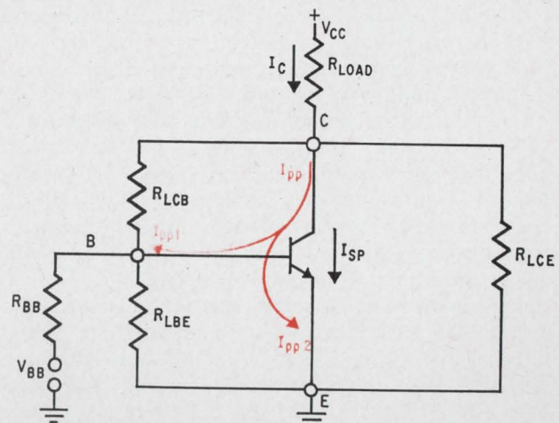
Irradiated transistor. Photocurrent produced in a transistor by ionizing radiation is amplified. The primary photocurrent splits two ways.
