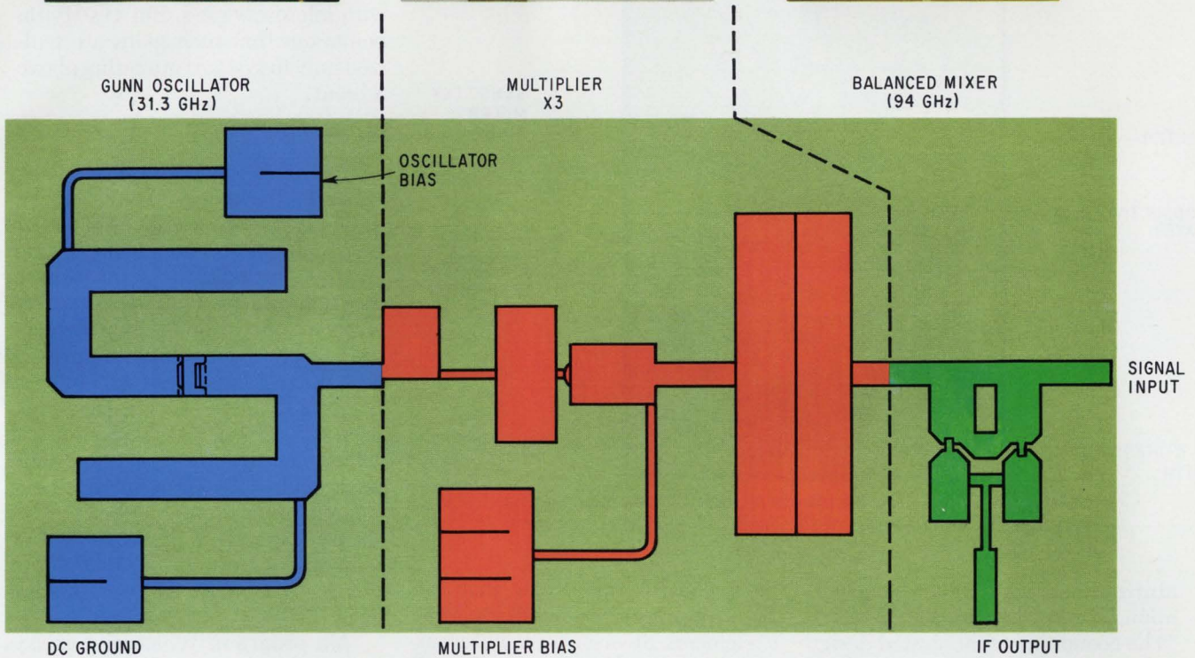
Three in one. This state-of-the-art device developed by TI for a 94-GHz receiver for the Air Force has three functions on a single monolithic chip. The circuit is fabricated on a 40-by-80-mil semi-insulating gallium-arsenide substrate.
