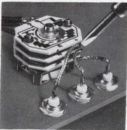
Switch plus. Wafer can have as many as 10 resistors screened on each side.
