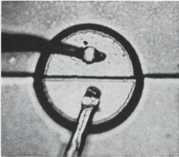
One micron or less separates the emitter electrode (top) and base electrode (bottom) of Sony's double diffused germanium pnp transistor. Used for high-frequency applications, it can be fabricated easily.
