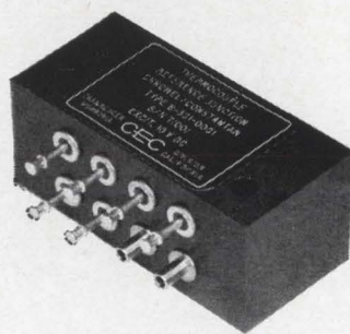
Type 8-301 Thermocouple Reference Junction
