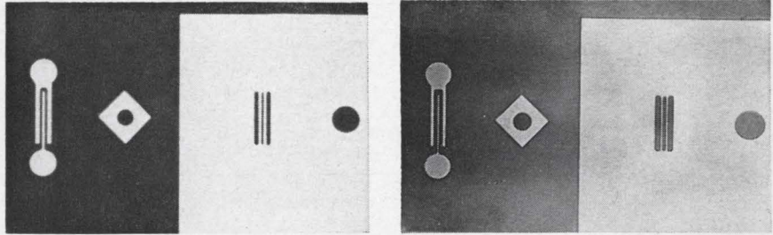
Submicron transistor patterns produced by optical masking. At left is a metal-film masking image; at right, pattern etched in silicon dioxide. Transistor's emitter line and base stripes are 0.65 micron wide, the wavelength of red light
