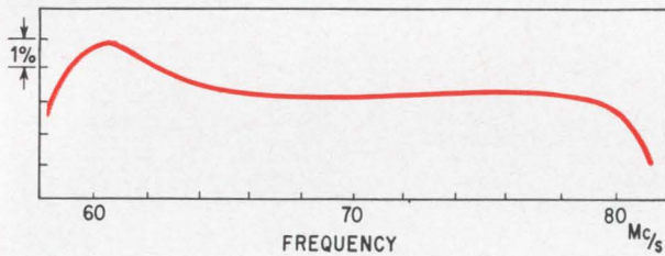
Frequency modulator (top), with four abrupt junction diodes (shown in color) in tuning circuit has linear output. Linearity, bottom, is within 1% over range of 70 Mc \pm 8
