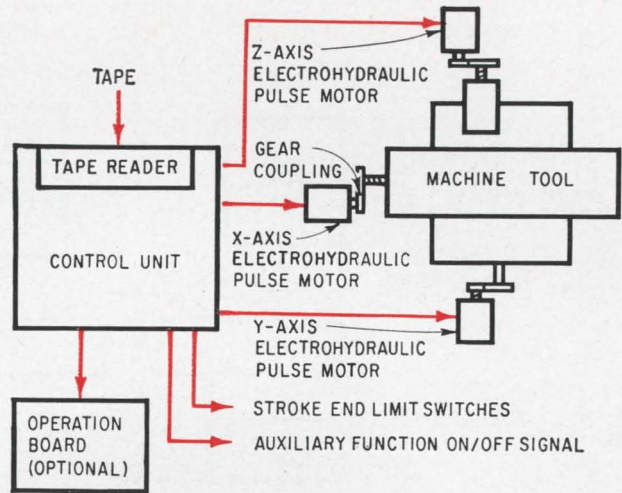
Main parts of Fanuc 260 are a transistorized control system and the electrohydraulic pulse motors that serve as digital-to-analog converters and power drives for feed screws
