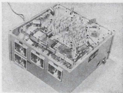
Probes push up through plenum chamber to contact circuit board. Board (not shown) is mounted above the array of probes.
