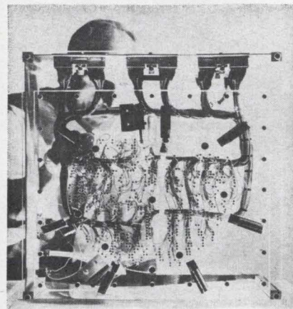
View through transparent chamber shows wiring harness between probe and multipin connectors, for connection to an automatic circuit analyzer.
