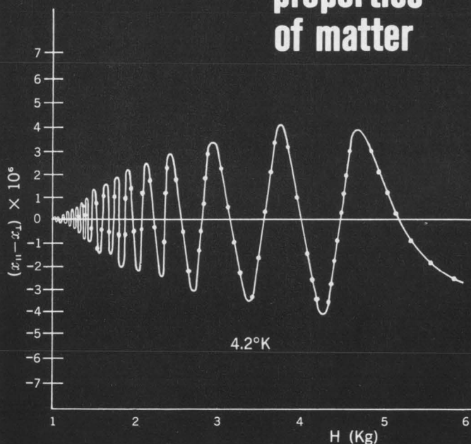
Typical deHaas-Van Alphen Effect
