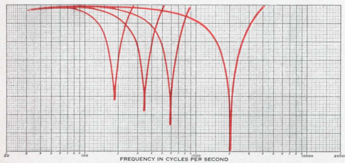
Recording of transmission characteristics of an adjustable notch filter for four different frequency settings. This plot is a permanent ink recording on 4-inch-wide chart paper. Dynamic recording range is 40 dB (20- and 80-dB dynamic ranges also available). Recorder chart speed and pen writing speed can be set over ranges of 2.5 to 75 in/min and 1 to 20 in/s, respectively.
