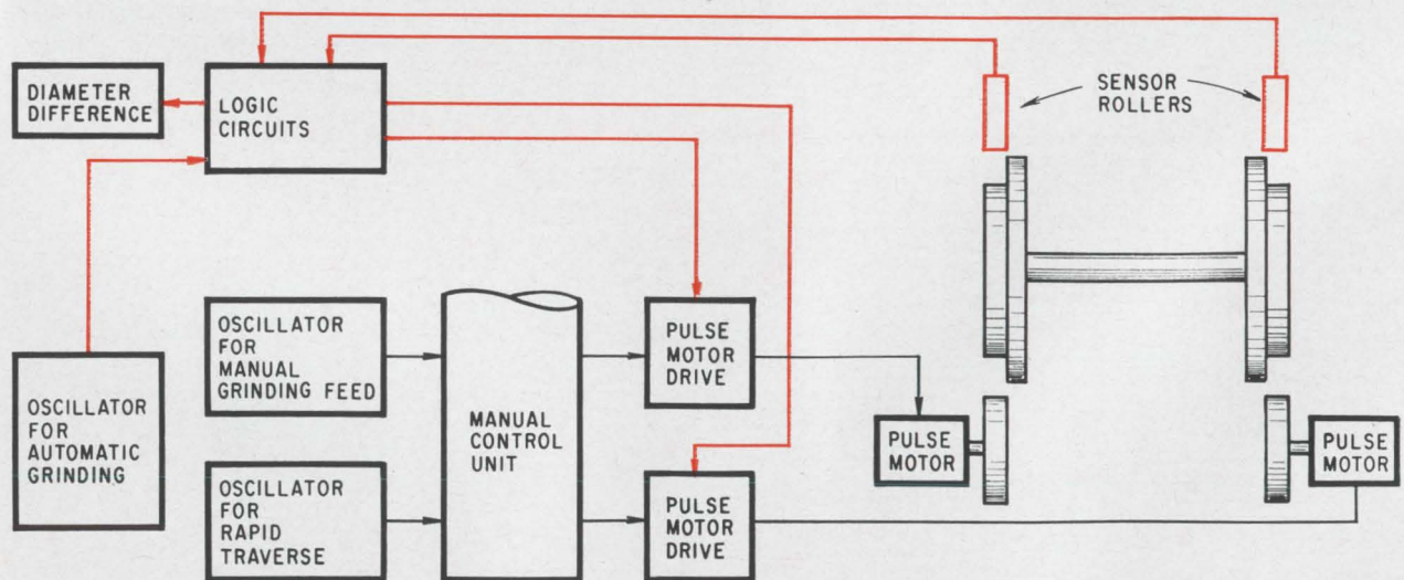
Truing of wheels is manually controlled in wheel grinder used by Japan National Railways on new Tokaido line. But diameter of wheels on the same axles are matched by automatic grinding (controls shown in color). In the 75-ton wheel grinder, four identical systems grind eight wheels of a car.
