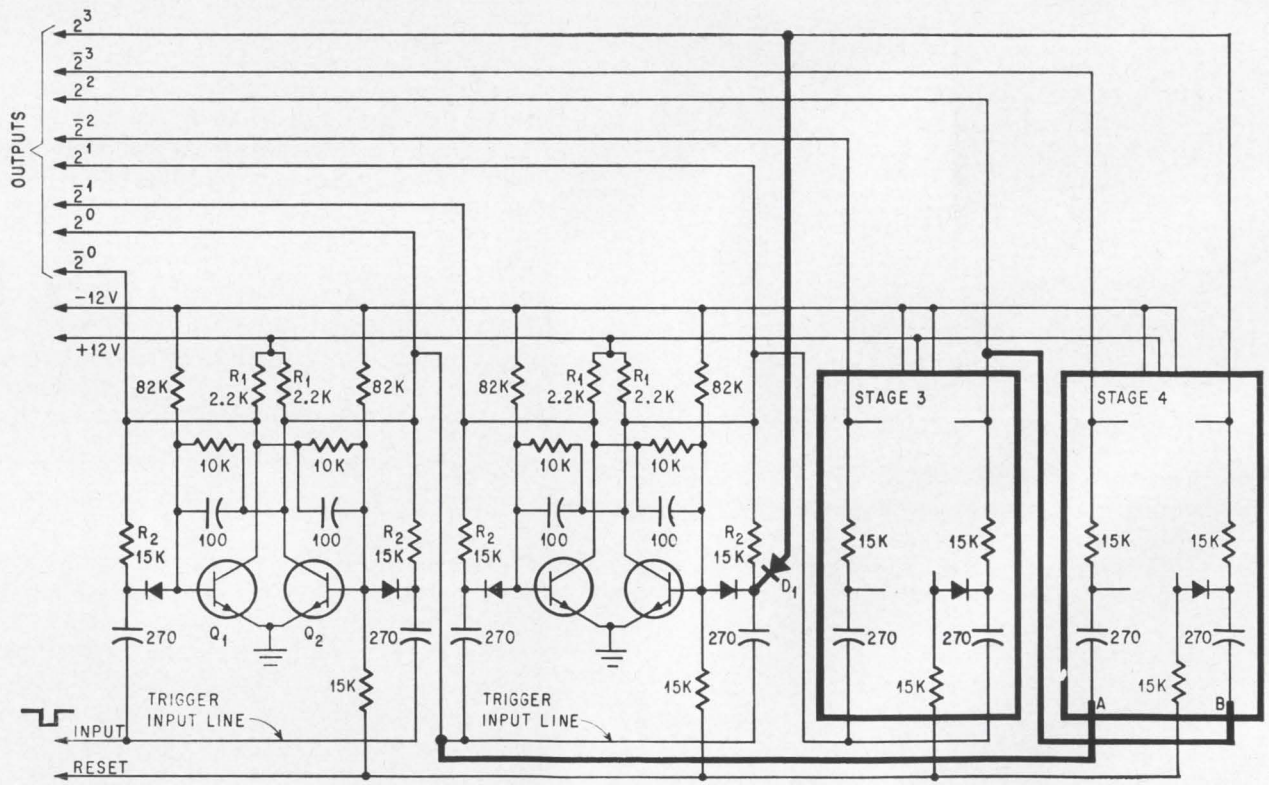
Decimal counter operates at the maximum repetition rate of the flip-flop stages. Heavy lines in the schematic indicate the changes that have been made in the basic circuit.
