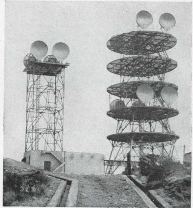
Microwave repeater stations, like this one at Futago Yama, dot the hilltops of the Japanese countryside. Inside the building is a heterodyne repeater.
