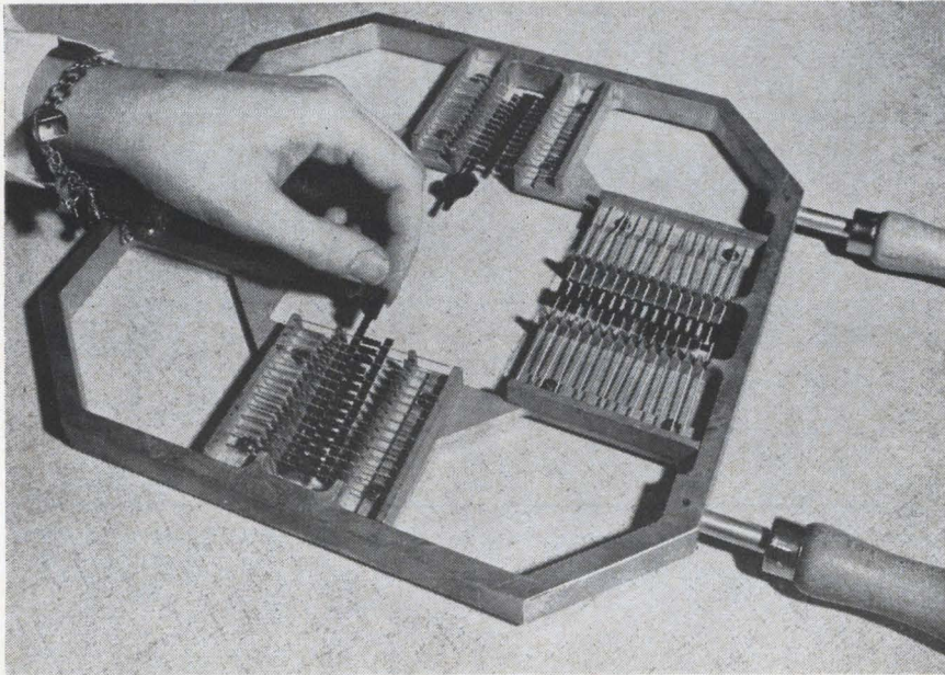
Zener diodes , encapsulated in thermosetting silicone plastic, are removed from fixture after coming off assembly line. Assembly of the silicone plastic diode lends itself readily to automation; yields are higher than with designs requiring more complicated production techniques.
