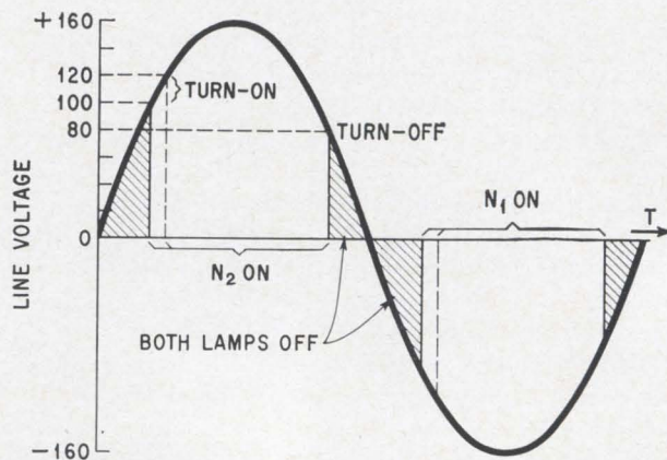
Ignition voltage of neon lamps varies (jitters) and must be considered when the phase of the output a-c is important.
