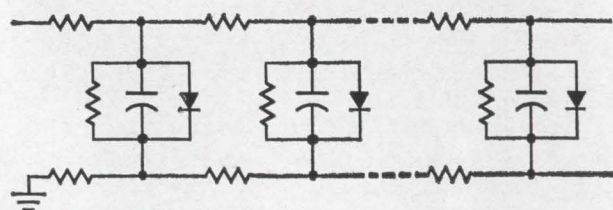
Capacitance and rectifying properties of the p-n junction are indicated in this equivalent circuit for a diffused resistor.
