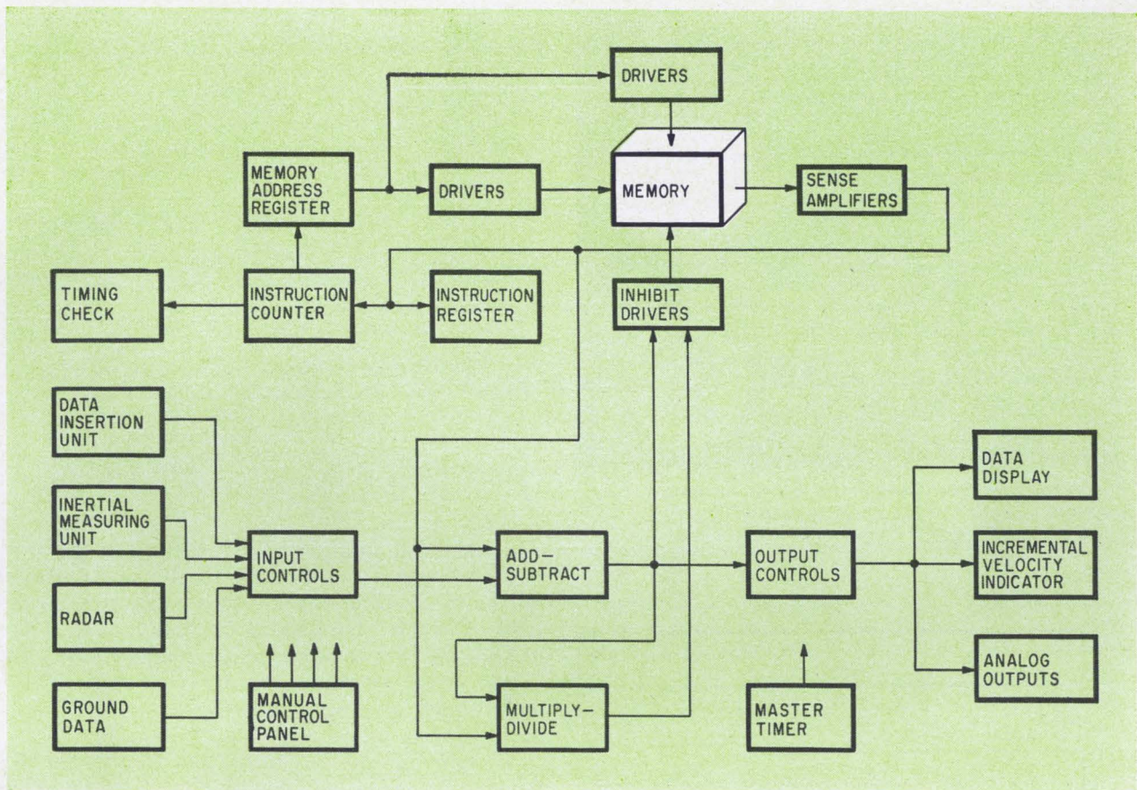
Data flow in Gemini's computer. All data and instructions originate in memory. Control of inhibit drivers by add-subtract unit and multiply-divide unit prevents writing of "ones"; all cores are first set to zero when writing. Nondestructive readout memory does not require regeneration.
