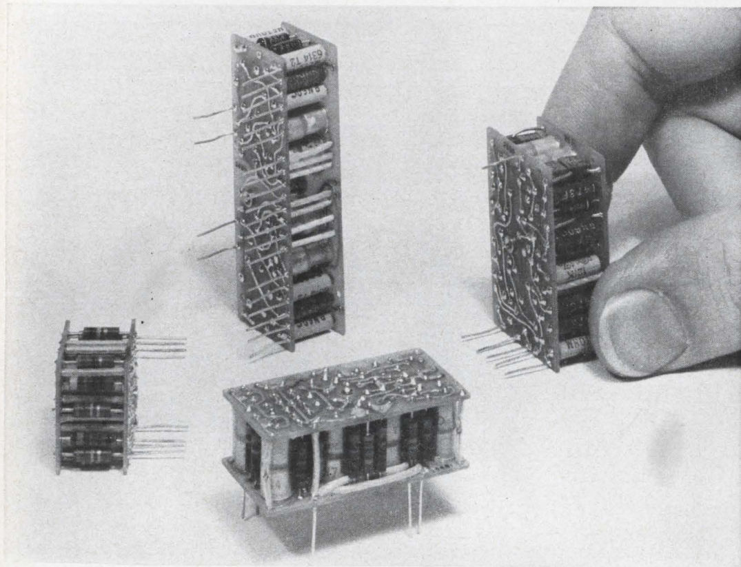
Cordwood construction of the circuit modules before encapsulation.
