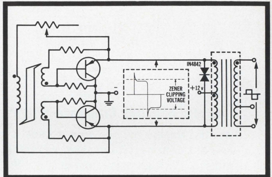
Figure 5. One 1N4842 double-anode regulator protects both transistors by clipping transients in this dual-transformer inverter
