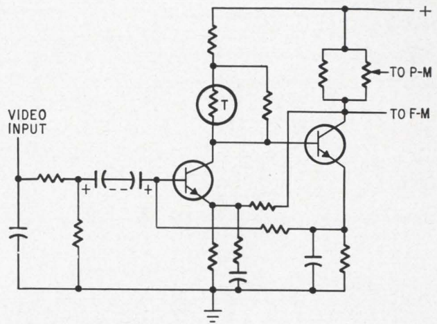
Video amplifier is direct-coupled, eliminating bulky capacitors.
