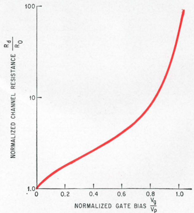
Normalized drain current versus voltage characteristic of field effect resistors (top) is nonlinear. Using only the region below pinch-off, (color line) the curve for channel resistance as a function of gate bias is derived at lower right. Overall V-I curve of this type of resistor shows essentially constant current between pinch-off and breakdown.
