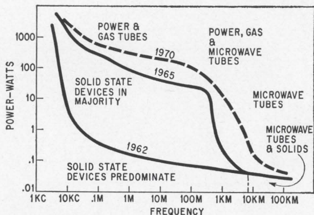
Comparison of tubes and solid state devices. It is evident that there are some areas where it will be a long time before solid state can replace tubes.
