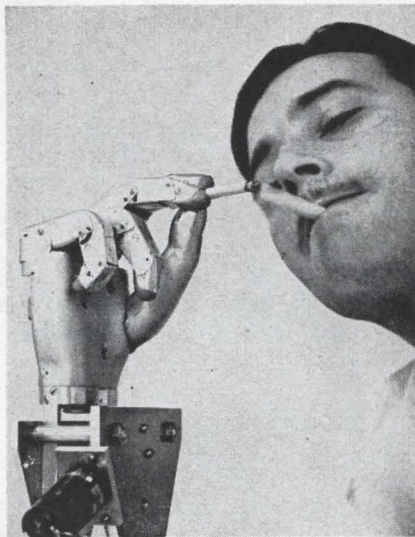
Artificial hand is steadier than the cigarette the user is lighting. Motor is in cylindrical tube at bottom. In use the hand has a plastic cover.
