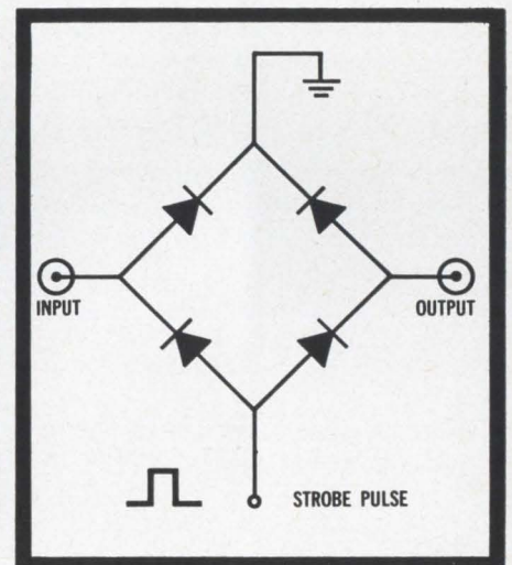
Figure 7. Oscilloscope sampling gate uses TIXD27 metal-barrier silicon diodes
