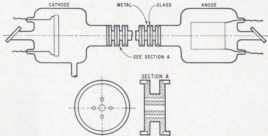
Laser discharge tube with rings of metal. New design is expected to permit high-power lasers.
