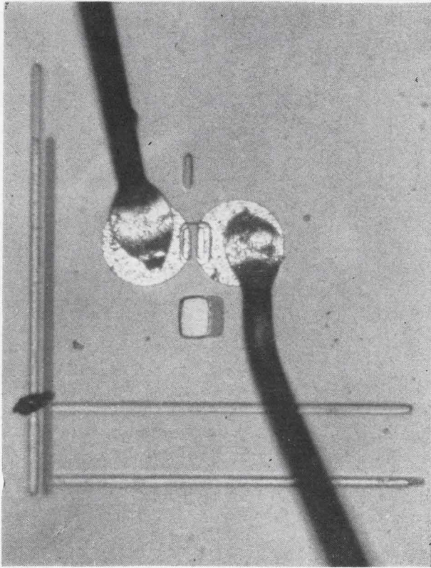
Unretouched photograph of the 2N393 mounted on the header. The two one-mil diameter wire leads attached to the bonding islands dwarf the actual transistor.
