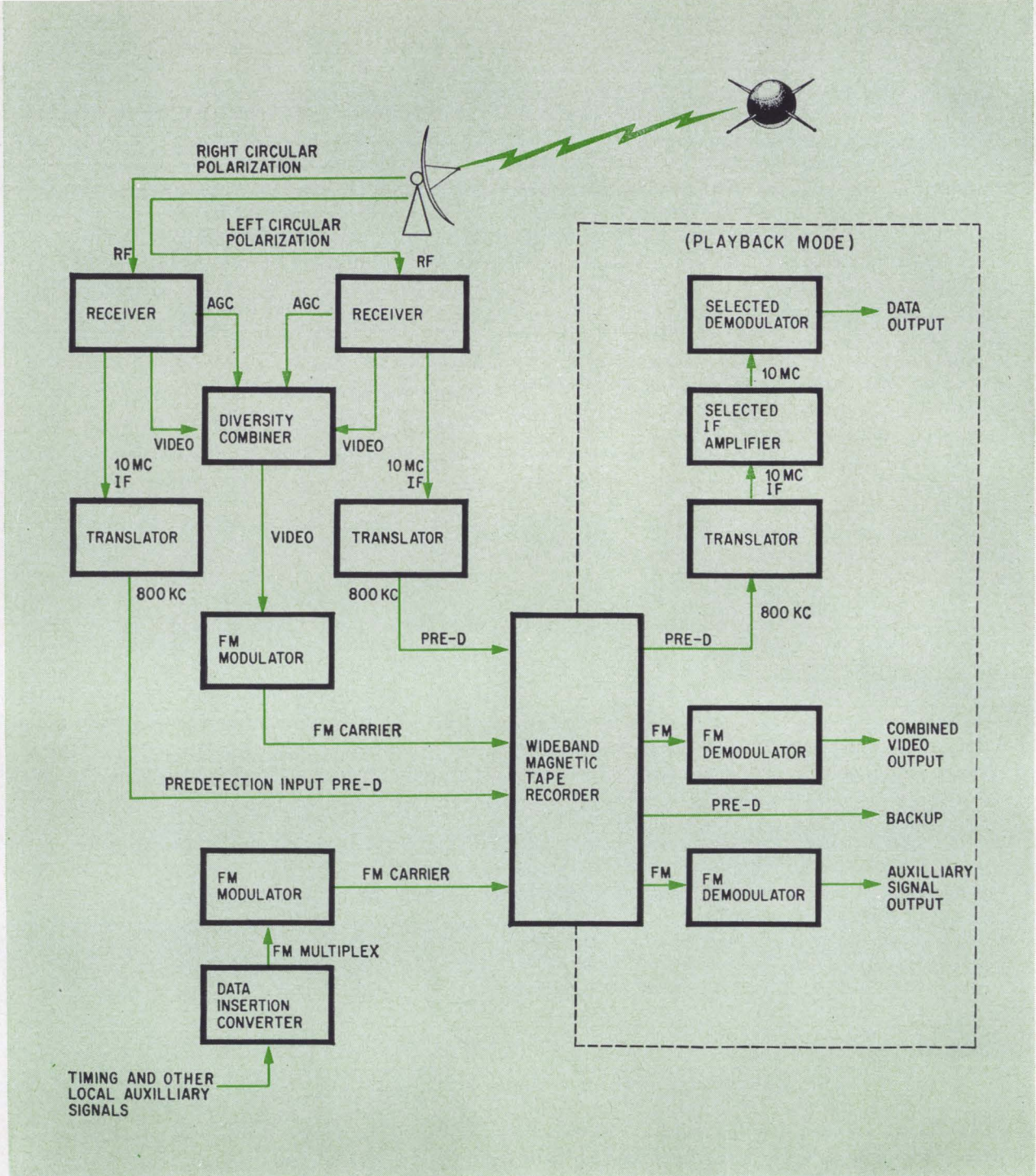
Pre-detection techniques have produced a real breakthrough in operational procedure of the missile range telemetry system. With pre-d, all known types of modulation can be received and recorded with common equipment.
