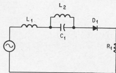
Tuned rectifier circuit. The transformer leakage inductance is represented by L_1 . Capacitor C_1 is series resonant with L_1 at the fundamental frequency. L_2 provides d-c bypass for C_1 .
