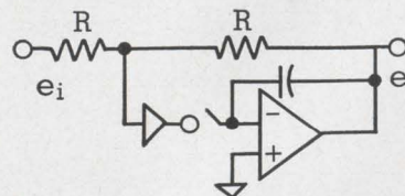
TRACK-AND-HOLD CIRCUIT
