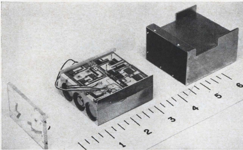
The 15-Mc thin-film receiver. The end plate at left has a screw at its top right-hand corner, which turns the receiver on. Center unit, made of plastic, reveals the circuit on top and three of the nine mercury cells at left. Remainder of the plastic housing is at right.
