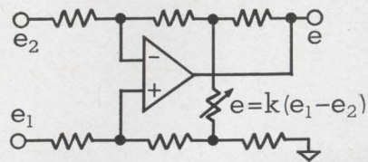
ADJUSTABLE-GAIN SUBTRACTOR
