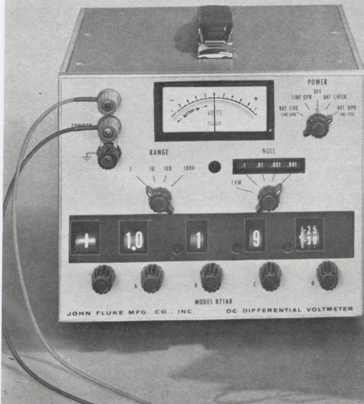
Model 871AB DC Differential Voltmeter
