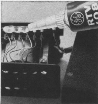
1. RTV-108 provides instant, "see-through" insulation as well as vibration resistance and environmental protection. RTV needs no pre-mixing; is applied directly from the tube.
