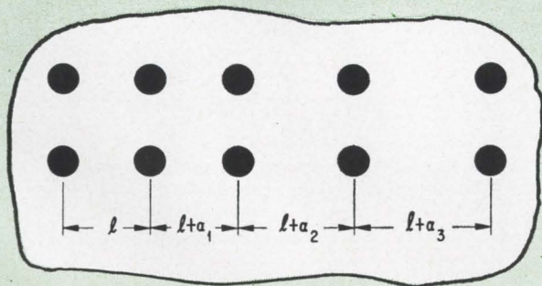
Conventional mask pattern for etching circles on a semiconductor wafer. As with the mask containing the squares, errors occurring during mask fabrication produce uneven spacing between circles.
