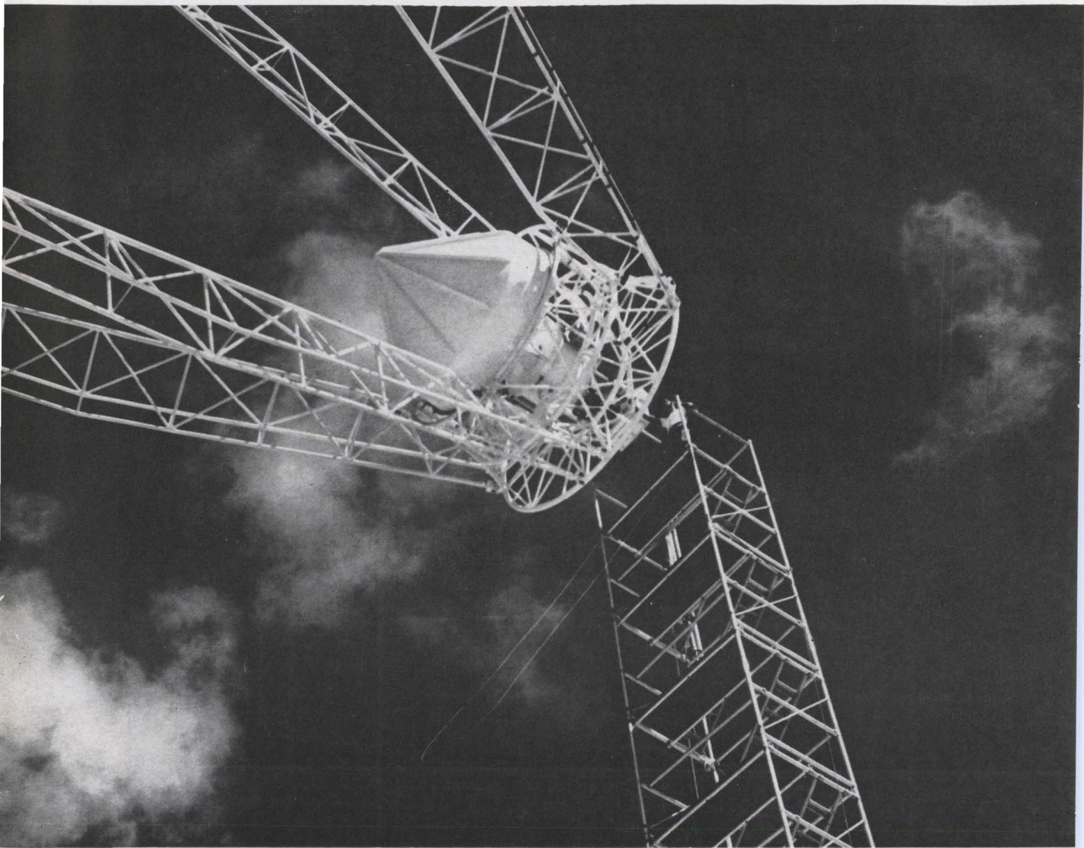
Dual conical spiral feed on the TAA-2 telemetry antenna covers the 130 Mc to 2,300 Mc range.
