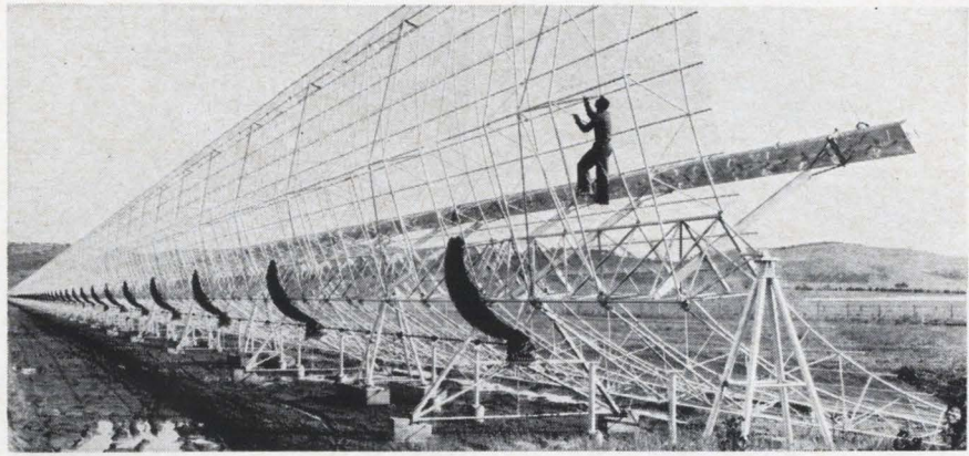
Antenna wire mesh of the mile-long east-west arm being inspected. Dark horizontal line just above ground is a motor-driven shaft that rotates the arm as much as 55° about its long axis.
