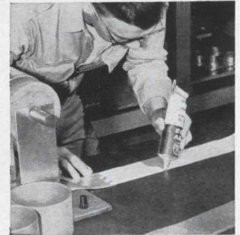
4. RTV bonds sheeting into desired configuration in low volume production of cylindrical air ducts for dielectric heaters. Results: production costs cut more than 300%.
