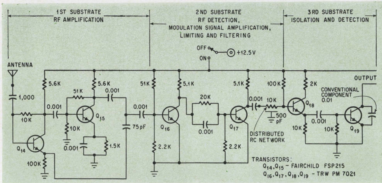
Microelectronic receiver circuit uses three substrates containing thin-film passive components. Each substrate also contains two transistor chips cemented in place. A fourth substrate provides for terminal connections; it also holds a 0.01-microfarad capacitor, the only conventional component used in the receiver.
