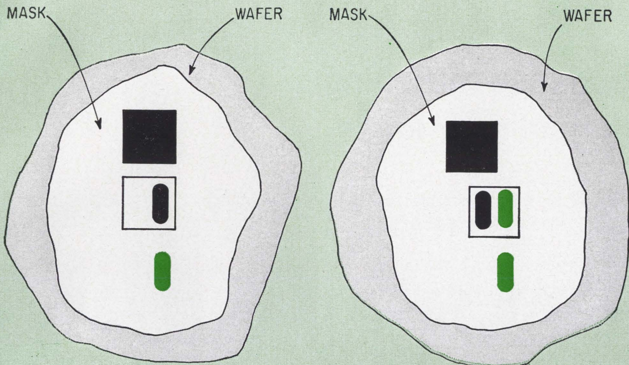
Accurate alignment of the two patterns is shown in the center. Lower pattern is leftover from the first masking process.
