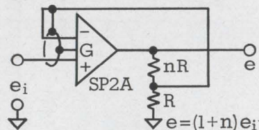
FOLLOWER-AMPLIFIER
