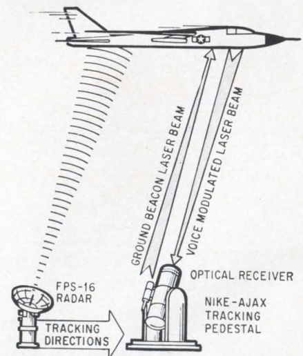
In test of laser space communication, radar locks onto plane and directs slaved optical receiver. Operator in plane aims laser transmitter manually.
