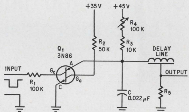
Generator can be operated in the gated mode by applying negative pulses at the cathode or can be free-running when this gate is open-circuited. The value of resistor R_5 must match the impedance of the delay line selected.
