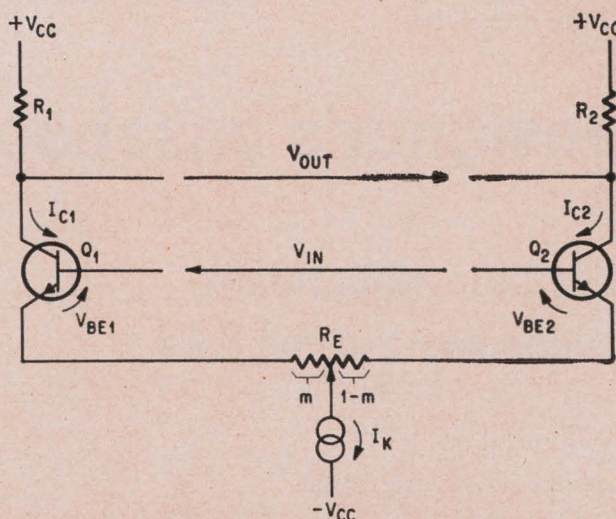
Diagram of basic differential-input, differential-output amplifier. Resistor R_E is adjusted so that V_{OUT} equals 0 when V_{IN} equals 0.
