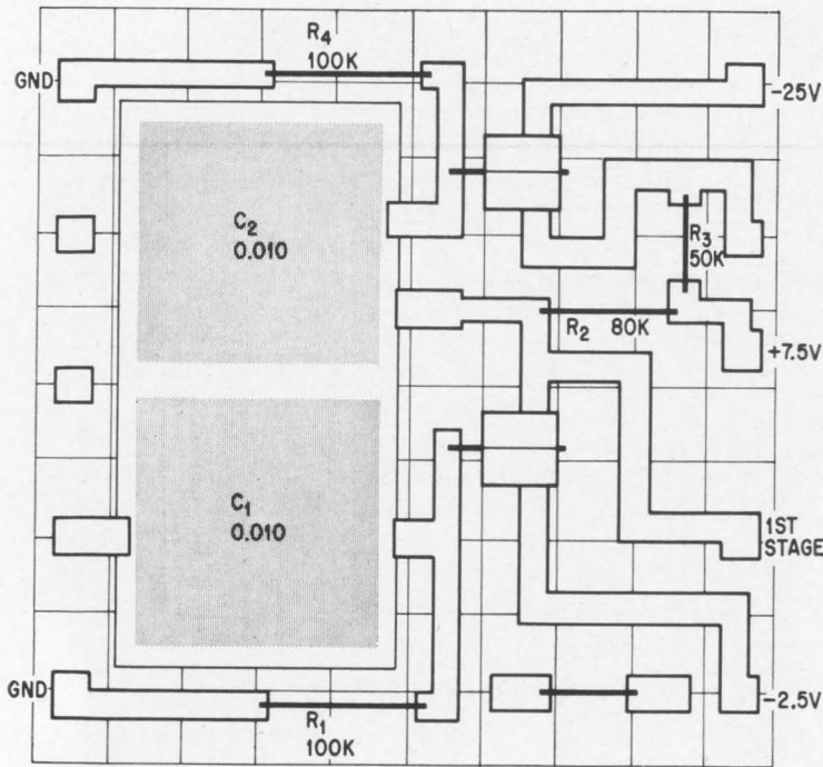
Thin-film amplifier incorporates two silicon-monoxide aluminum capacitors, two thin-film triodes and several chromium and rhenium resistors. Evaporated interconnections offer increased reliability; low mass has greater resistance to radiation damage.
