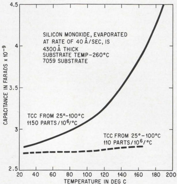
Capacitance as a function of temperature for silicon monoxide. The broken line shows that silicon-monoxide capacitors can be operated up to 165°C, with negligible change in capacitance after a heat treatment at 400°C for 30 minutes.
