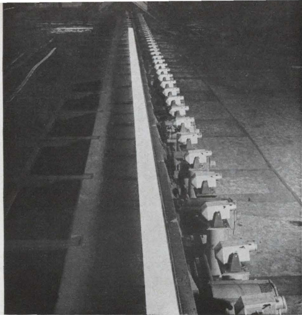
Hot billets are sized as they whiz past 72 infrared-sensitive photocells. Data goes to billet-cutting computer.
