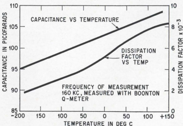
Capacitance and dissipation factor increase with temperature for an aluminum-oxide capacitor.
