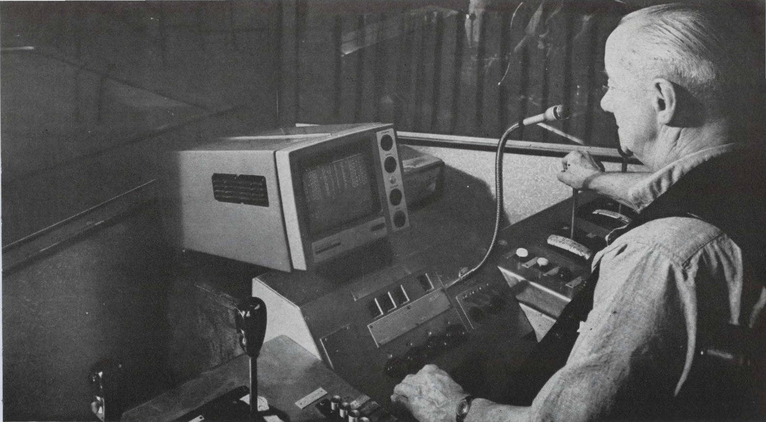
Operator controls cutting of blooms after reading computer-generated instructions on the face of the cathode-ray tube display.
