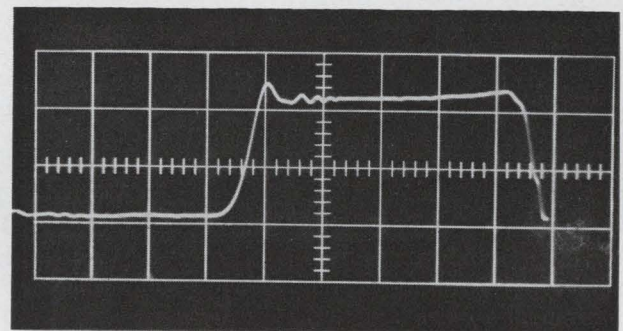
Pulse output across R_5 = 3.9 kilohms, pulse duration of 5 \mu sec , 500 pps, 20 v amplitude with HH-400 delay line. Horizontal scale is one microsecond per division.
