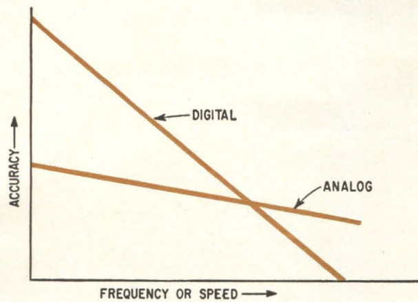
Digital systems tend to lose accuracy faster than analog systems as operating speed increases (left). Analog systems are generally cheaper (right) than digital for simple problems but cost more to expand.
