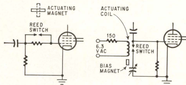
Using the reed switch to determine the influence of a series grid resistor
