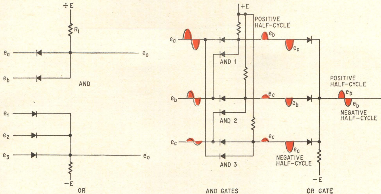
Amplitude selective gates, AND and OR, as used in voter circuit at right
