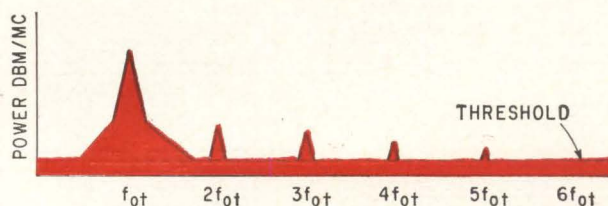
Combined emission spectrum at receiver input terminals.
