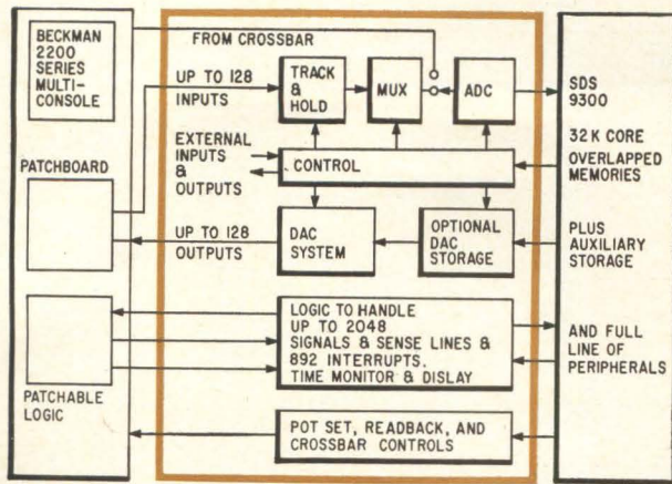
In the Beckman/Scientific Data Systems hybrid computer two low-cost general-purpose computers are linked by powerful interface equipment.
