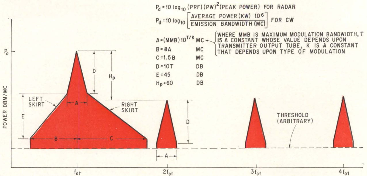
Stylized transmitter emission spectrum used in interference prediction.
