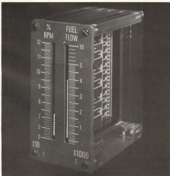
Electroluminescent bar graph by Sylvania produces 25 lines to the inch with 25- to 30-foot lamberts brightness. The unit shown is intended for aircraft or space-craft instrumentation.
