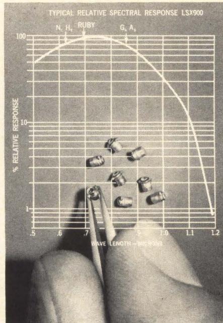
FIGURE 3. Sensitivity curve and packages for LSX 900 light sensor
