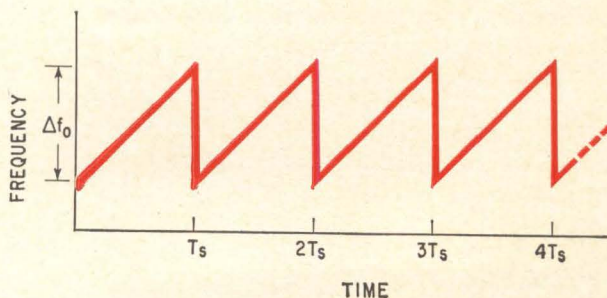
Periodically swept-frequency signal is the basis of the FSM system.
