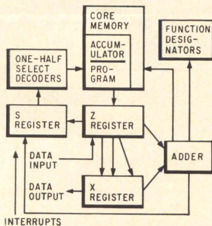
Westinghouse's Prodac 50 time shares components with this logic arrangement. Registers and memories do double duty for computation, logic decision making and control.
