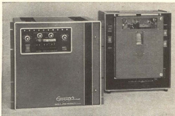
Portable data processor by Epsco Inc., Cambridge, Mass., has been used to field-test automotive components. Up to 100 sensors measure shock, vibration, acceleration and other variables while the car is in motion. Signals are digitized to 1 part in 1,000 at 20,000 samples per second.
