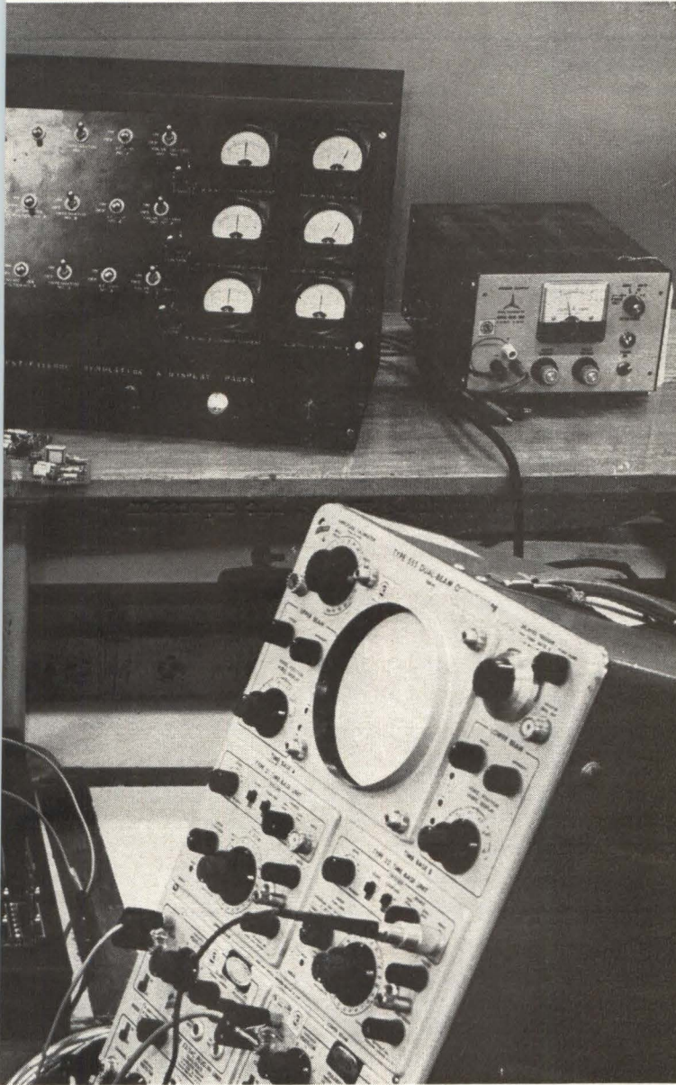
Frank Thomas tests breadboard of triple-redundant stability system.
