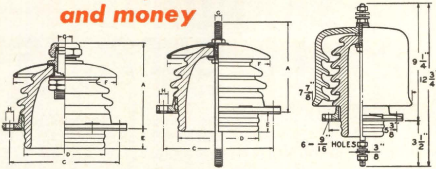
TYPE A Permits use of continuous pipe conductor through the insulator.
