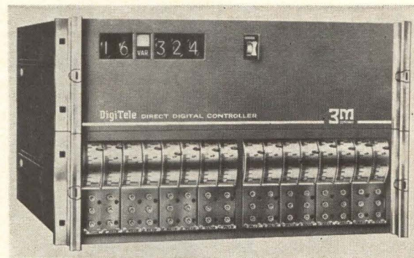
Direct digital multiloop controller will control pressure, temperature, flow and similar variables, relieving computers of competitive control calculations according to 3M Company, the manufacturer.
