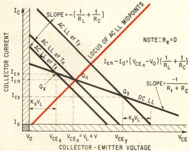
Load line diagram for common-emitter micropower amplifier.
