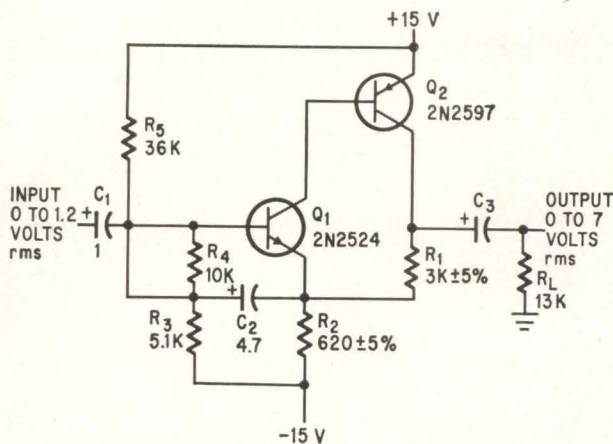
Complementary amplifier provides 220,000-ohm input impedance and wide operating temperature stability.
