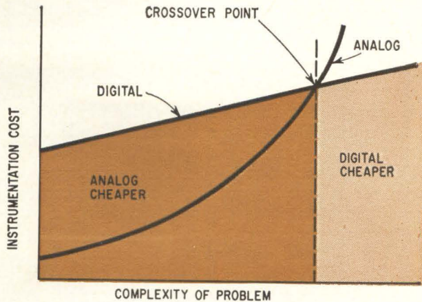
Digital systems tend to lose accuracy faster than analog systems as operating speed increases (left). Analog systems are generally cheaper (right) than digital for simple problems but cost more to expand.
