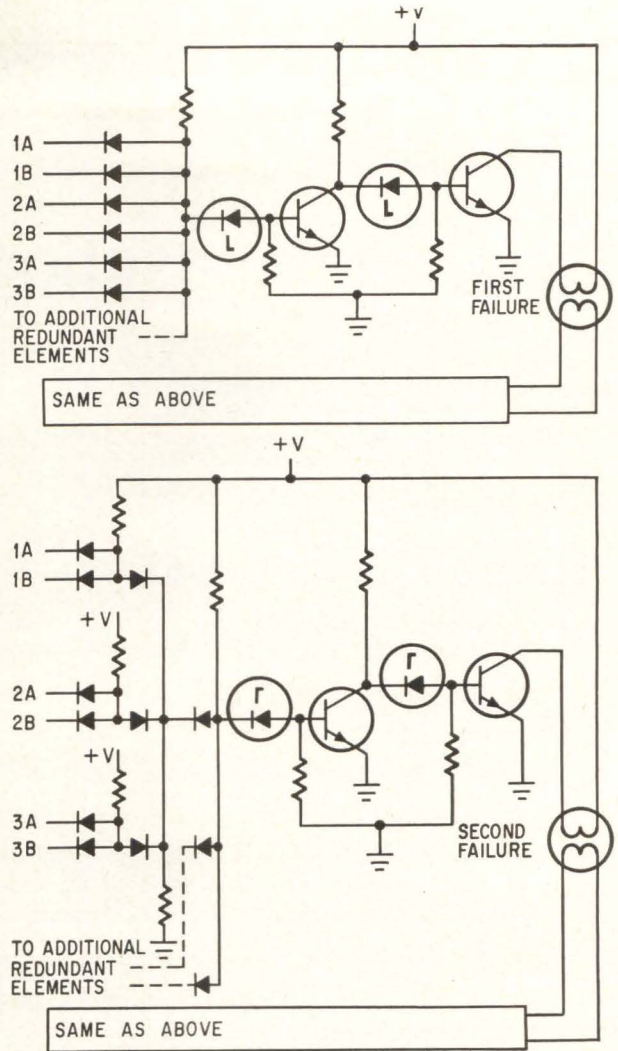
Logic and driver circuits, which use double-filament lamps
