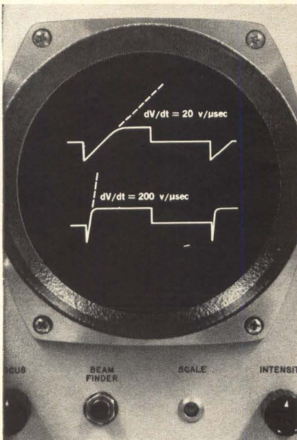
FIGURE 2. dV/dt comparison between TI 2N3037-42 and conventional SCR's
