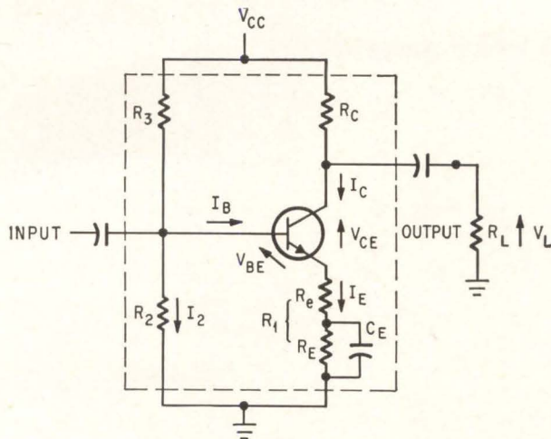
Common-emitter micropower amplifier schematic indicating circuit d-c currents and voltages, and peak a-c load voltage V_L .
