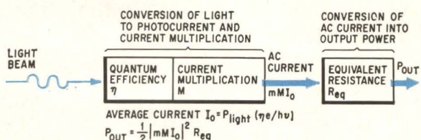
Photodetector for a-m optical signals.
