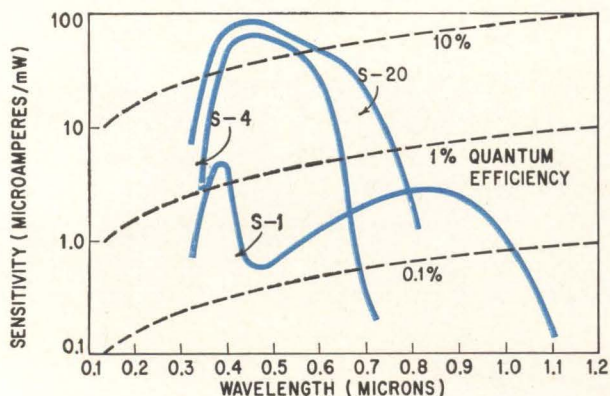
Typical spectral response curves for S-1, S-4 and S-20 photoelectric cathodes
