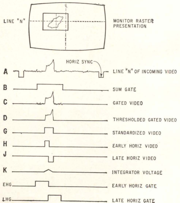
Target reference waveforms. Letter callouts refer to video tracker block diagram.
