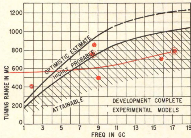
Projected tuning ranges based upon a completed rotary tuning development and three experimental models shows probable tuning range of better than 1 Gc at 19 Gc.
