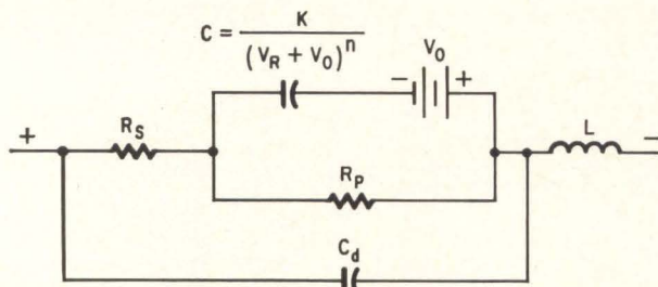
Voltage-variable capacitor equivalent circuit.
