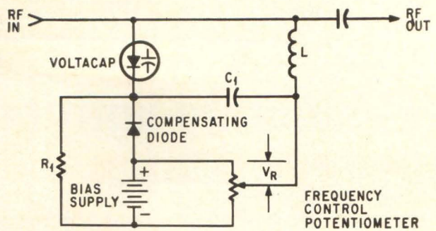
Compensating for diffusion potential v_o with a forward bias.
