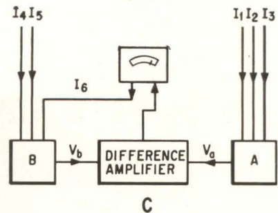
3-D multiplier with input currents representing three parameters and output voltage giving their product (A). Dynamic characteristic curves of bridge (B). Practical circuits relationship (C) of output voltages A and B and amplifier current I_6 can be used to carry out a large number of mathematical operations.
