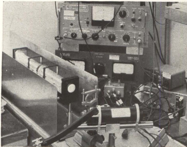
Test setup of an 11-to-20-gigacycle traveling-wave phototube and helium-neon gas laser.
