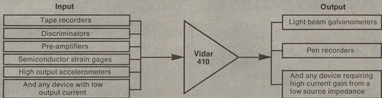
Typical applications for the Vidar 410 Galvanometer Amplifier
