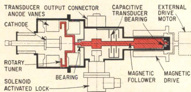
Solenoid lock shown at center of cross-section drawing holds tube at fixed frequency. Capacitive transducer indicates the approximate frequency to the receiver local oscillator.
