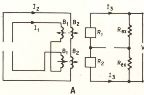
3-D multiplier with input currents representing three parameters and output voltage giving their product (A). Dynamic characteristic curves of bridge (B). Practical circuits relationship (C) of output voltages A and B and amplifier current I_6 can be used to carry out a large number of mathematical operations.
