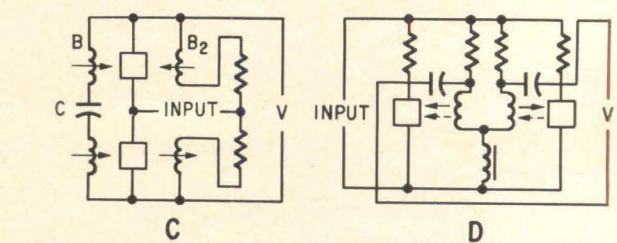
Amplifier in (A) is modified with feedback winding in (B) for a d-c amplifier. If the feedback is equal to or larger than unity and a capacitor is connected between the feedback windings, the oscillator shown in (C) is produced. Two capacitors in tank circuit give oscillator (D)
