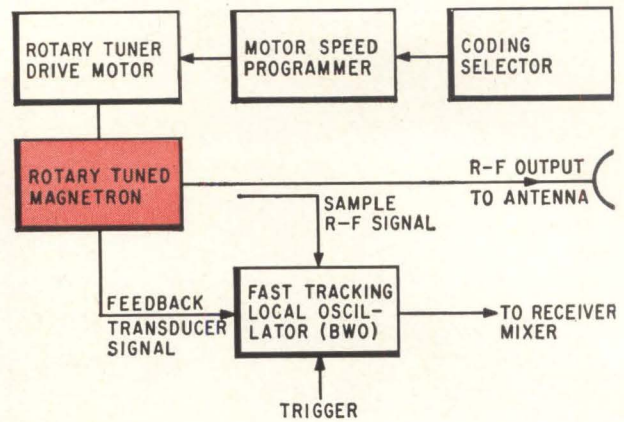
System of rotary tuning that might be applied as a modification kit for an existing radar.
