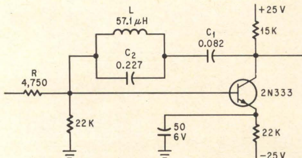
One-transistor operational amplifier is resonant at 1,200 cps and antiresonant at 1,400 cps.
