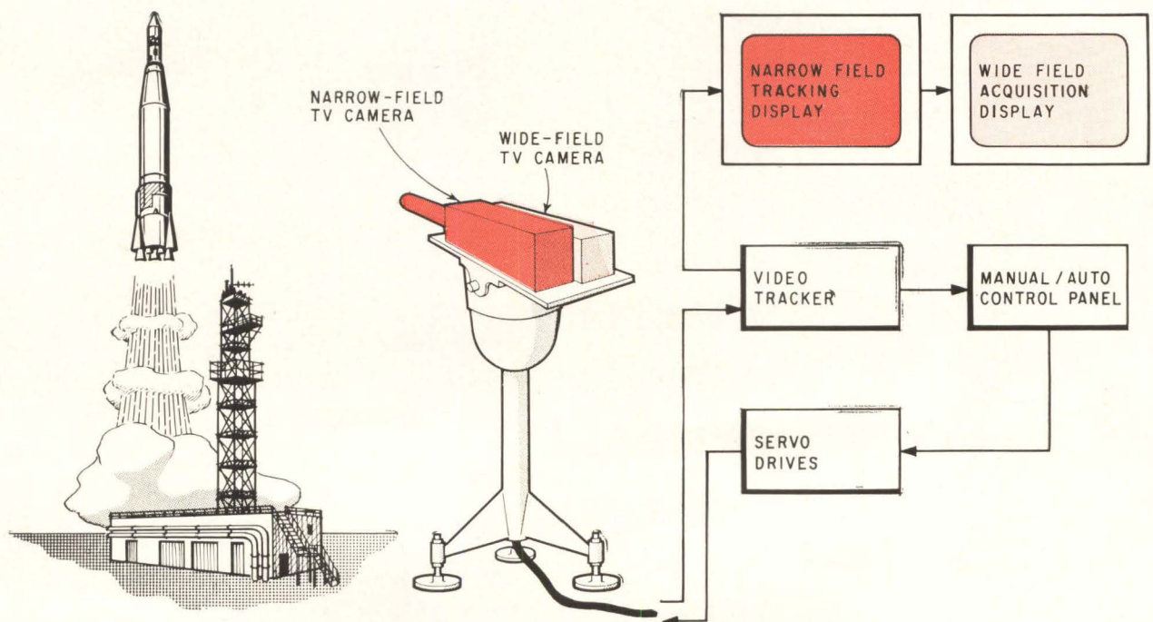
Wide-field camera acquires target while the tracking camera uses longer focal length optics for a narrower (1.8°) field.
