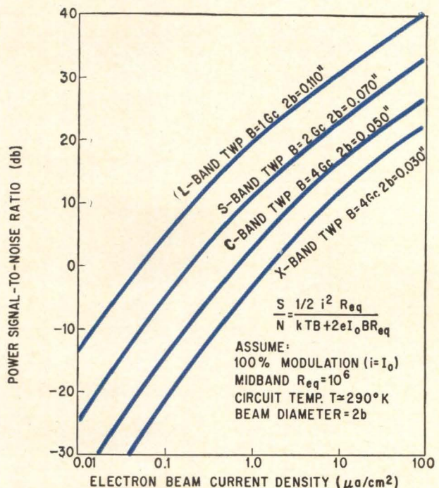
Plot of signal-to-noise ratio (equation 3, page 55) shows dependence of traveling-wave phototube signal-to-noise ratio on electron-beam current density.
