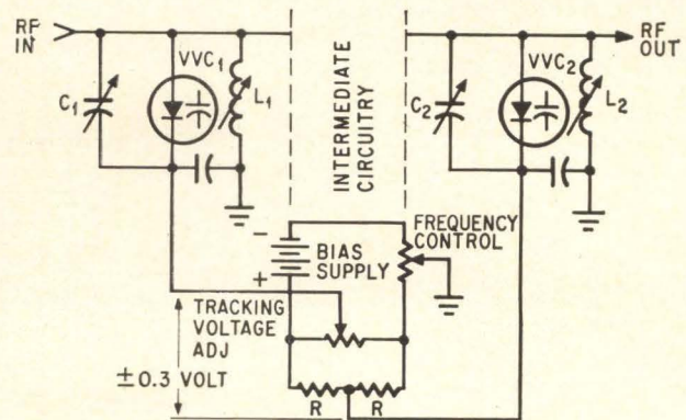
Three-point frequency tracking method uses a series offset voltage.
