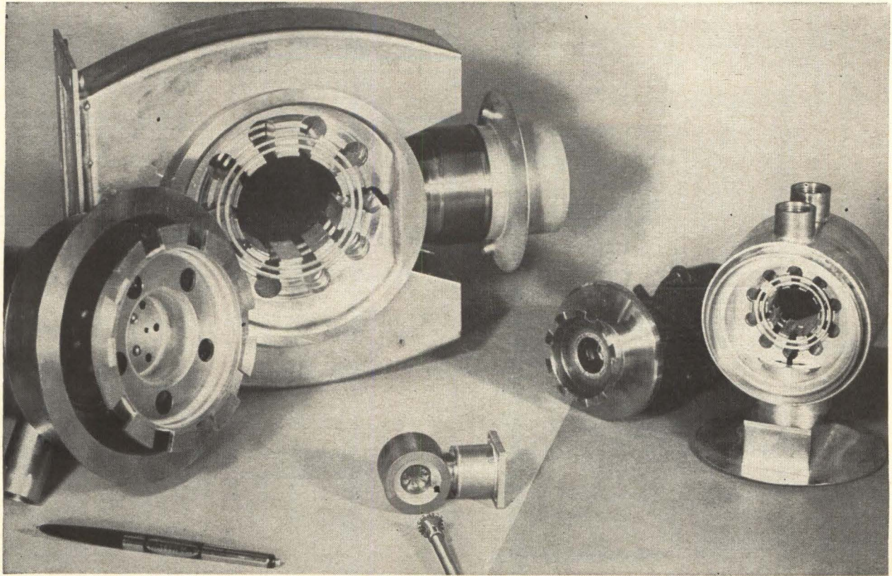
Tuning is accomplished by rotating the toothed wheels relative to the anode structures. Subassemblies shown are for the L,S and Ku bands.
