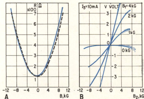
Indium antimonide used in two active elements gives identical curves when the magnetic field under four-kilogauss (A). A 3-D multiplier using these elements gives the family of curves in (B). The curves are linear when variable magnetic fields are less than four-kilogauss.
