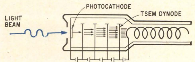
Distributed-emission photodiode, top; traveling-wave phototube, center; a traveling-wave phototube using transmission-type electron multiplication, bottom.
