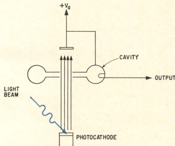
Cavity-type photoelectric diode, or photoklystron.
