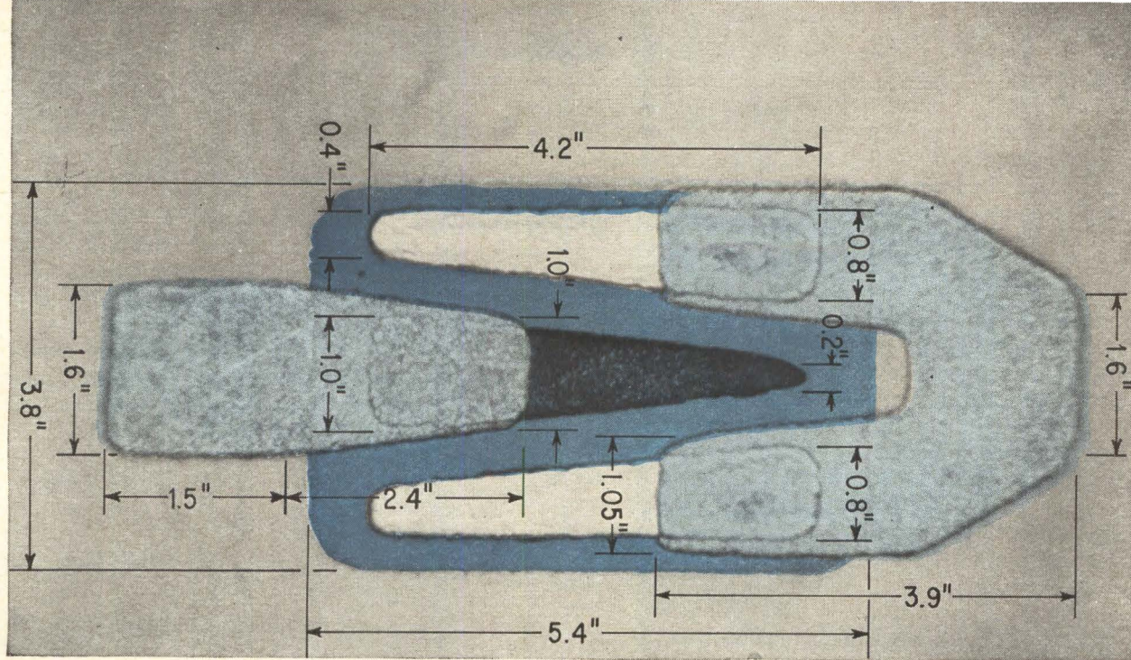
Planar germanium transistor has alloyed p-type emitter stripe and two alloyed base stripes.
