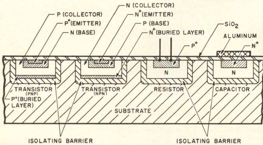
Epic process simplifies fabricating npn and pnp transistors within same semiconductor substrate, top, and improves speed and power dissipation as shown at right. "Floating collector" technique is illustrated right.
