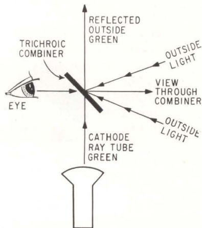
TRICHOIC combiner principle rejects outside green light, reflects cathode-ray-tube green signal into eye's direct view—Fig. 1
