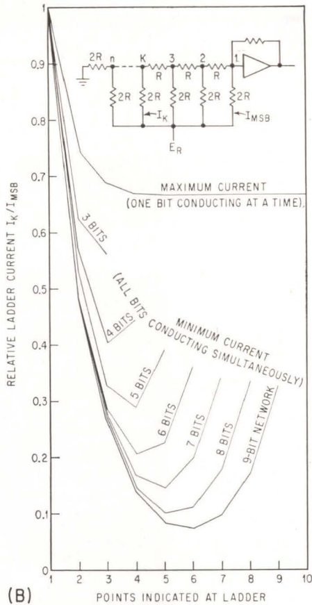
POTENTIAL distribution in ladder network (A); maximum current swing through the ON bit (B); maximum reverse current through the OFF bit (C)—Fig. 2
