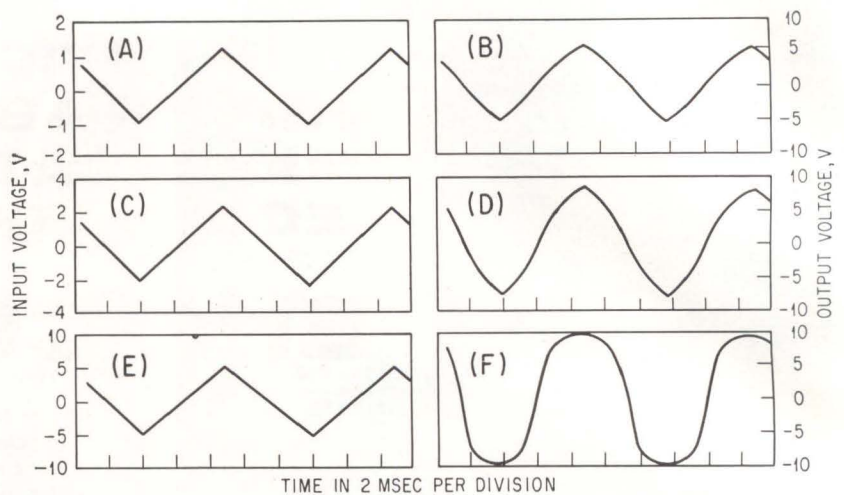
OSCILLOSCOPE displays show input-output amplitudes when the nlr is used for decreased gain—Fig. 5
