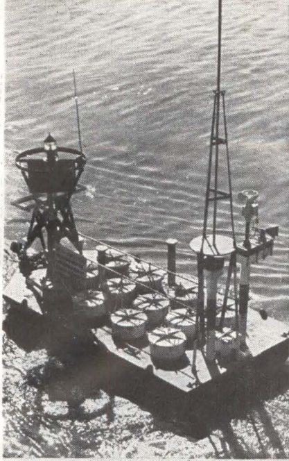
NOMAD BUOY. Martin Co.'s atomic-powered meteorological reporting system has just been installed in the Gulf of Mexico
