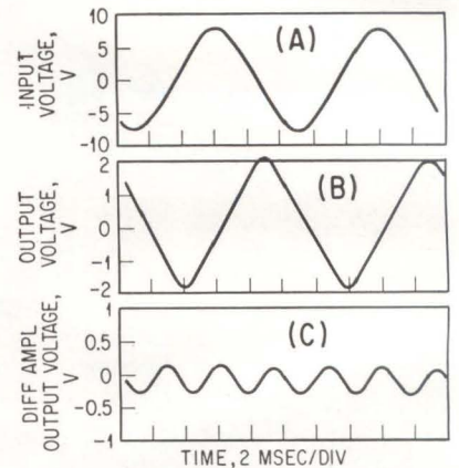
WAVEFORMS resulting from connection of the nlr to obtain third harmonic—Fig. 7
