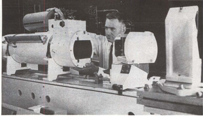
AUTHOR'S HAND rests on vidicon camera atop the autocollimator. In the middle is the penta mirror unit. At far right is the reference-prism unit
