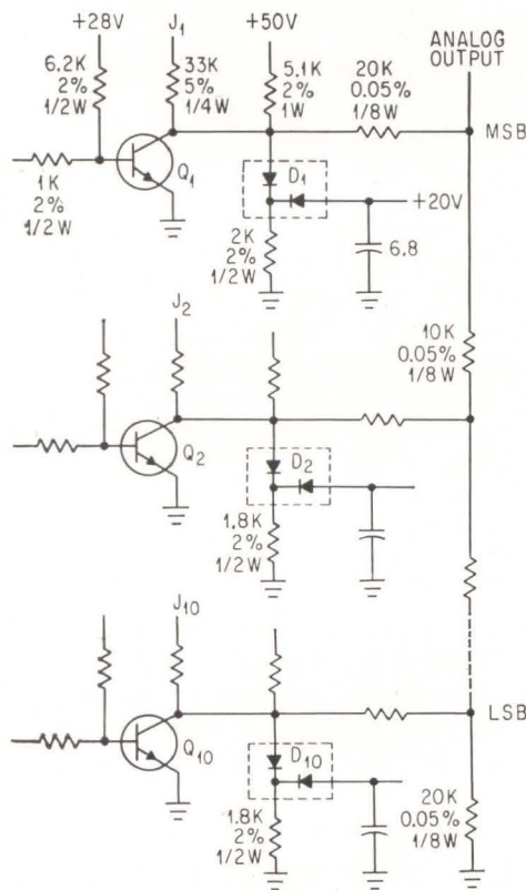
TEN-BIT digital-to-analog converter, accepting negative-pulse digital inputs at 0 to -8 volts—Fig. 5
