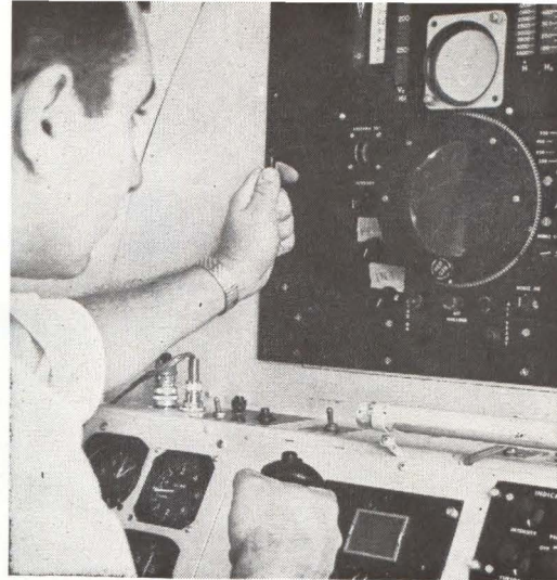
DISPLAYS for automatic TFR, built by Autonetics, consists of (center) plan position indication (PPI) and 3-D terrain to give azimuth, range and elevation information. Upper scope tells position of aircraft (circle) in relation to where automatic terrain following command (dot) says it should be
