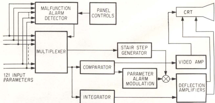
SYSTEM management display block diagram combines 121 input signals into bar-graph form generated on a single crt, and sequentially projected in groups into pilot's line of view—Fig. 3
