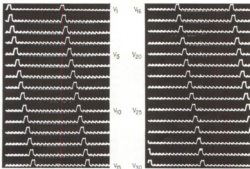
PULSE WAVEFORMS at each scan-generator output. Vertical scale is 3v/div, horizontal is 30 \mu sec/div; clock is 100 kc, 3 v peak-to-peak—Fig. 2
