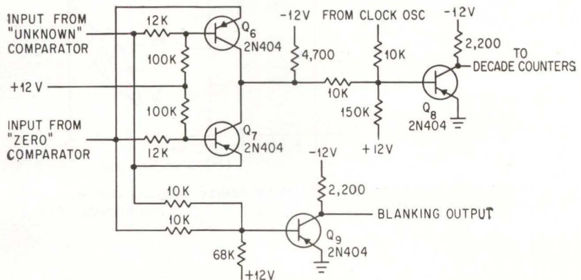
LOGIC is an exclusive OR gating circuit that produces a ground level signal only when the output of the two comparators are in different states—Fig. 5
