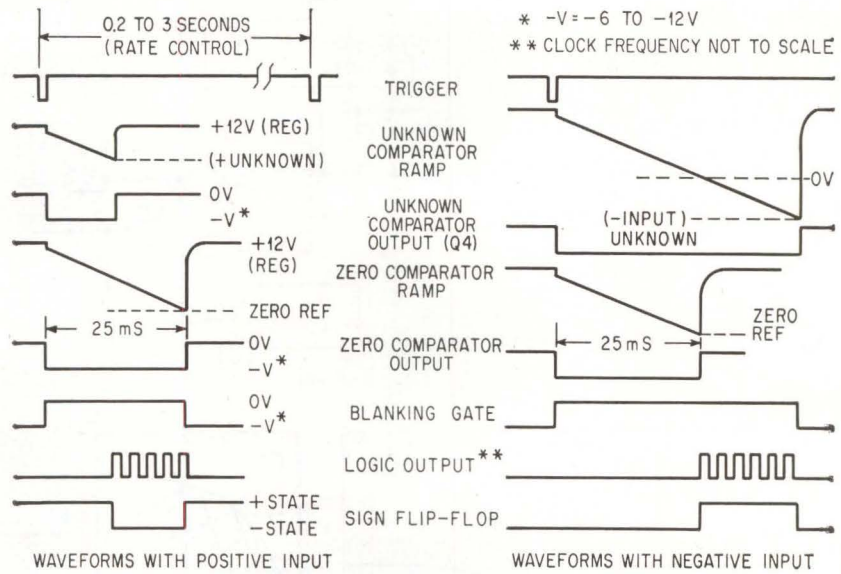
WAVEFORMS are produced by the comparator and logic circuits—Fig. 4
