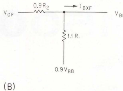
(A) DATA OBTAINED from example is plotted in (A). Dots corresponding to standard EIA resistors can be added to this graph to aid in selecting resistors. Worst-case conditions for Q_1 cutoff (B), and worst-case for the circuit during saturation (C)—Fig. 3
