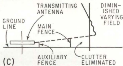
EFFECT of fences on r-f front shape: transmission without fences, (A); effect of main r-f fence, (B); effect of both fences together, (C)—Fig. 2
