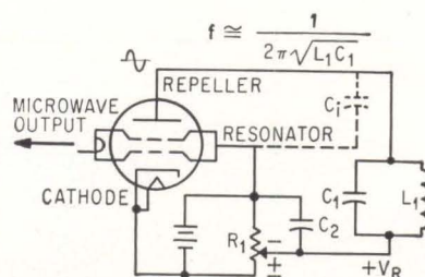
SIMPLIFIED version of superregenerative klystron circuit was found to provide its own quench action—Fig. 1
