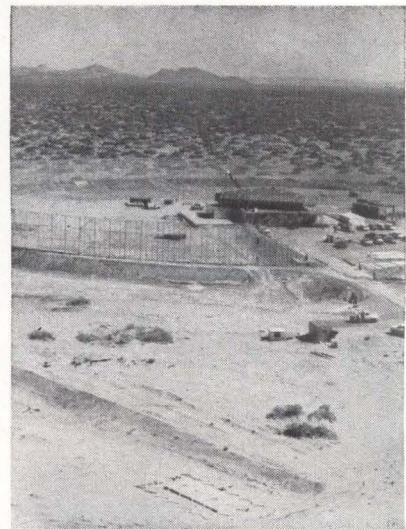
OVERALL VIEW of Nike-Zeus acquisition radar transmitter site at White Sands Missile Range during construction of main fence; auxiliary fence was added later—Fig. 1
