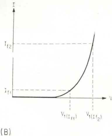
ENHANCED tunnel-diode NOR circuit (A) produces output only if none of the inputs are present; then charge-storage diode D_s is forward biased in state denoted by V_{1(I_{f1})} in (B); when clock pulse comes, it sweeps the stored charge of minority carriers across the junction in the reverse direction, producing a current pulse that is large enough to trigger the tunnel diode to its high-voltage state—Fig. 2
