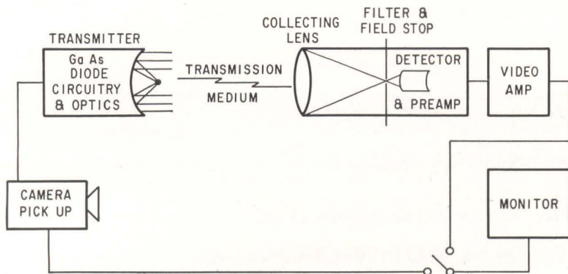
TV DEMONSTRATION setup. An 800-line picture was transmitted over a 12-ft path
