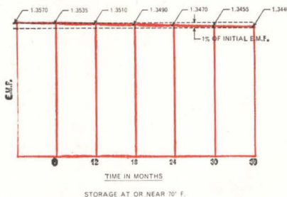
Long-term stability test shows steady output voltage from Mallory Mercury Batteries.
