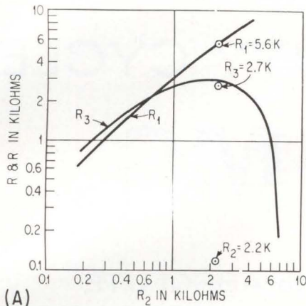
(A) DATA OBTAINED from example is plotted in (A). Dots corresponding to standard EIA resistors can be added to this graph to aid in selecting resistors. Worst-case conditions for Q_1 cutoff (B), and worst-case for the circuit during saturation (C)—Fig. 3
