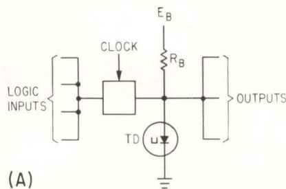
TUNNEL DIODE in (A) is heart of typical tunnel-diode NOR logic circuit. The tunnel charge-storage diode amplifier; current pulses through charge-storage diode are
