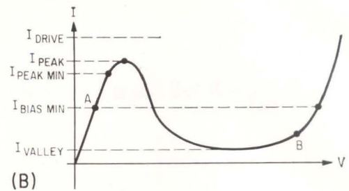
TUNNEL DIODE in (A) is heart of typical tunnel-diode NOR logic circuit. The tunnel charge-storage diode amplifier; current pulses through charge-storage diode are
