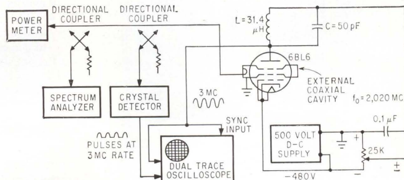
TEST setup finds best conditions for self-quench operation—Fig. 3
