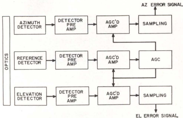
RECEIVER output amplitude indicates linear displacement of image. Transmitter is simply a pulsed laser and the necessary trigger circuit
