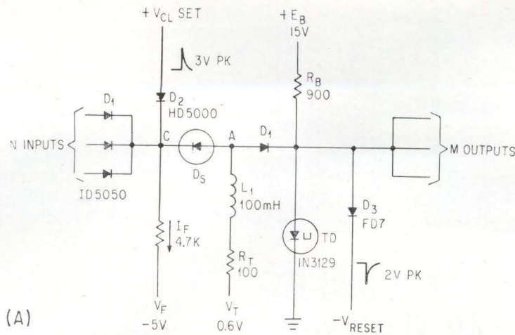
ENHANCED tunnel-diode NOR circuit (A) produces output only if none of the inputs are present; then charge-storage diode D_s is forward biased in state denoted by V_{1(I_{f1})} in (B); when clock pulse comes, it sweeps the stored charge of minority carriers across the junction in the reverse direction, producing a current pulse that is large enough to trigger the tunnel diode to its high-voltage state—Fig. 2
