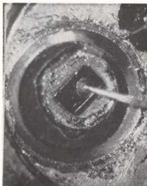
LASER is mounted with n-type material facing up. N-type crystal's greater transparency increases transmitter's light output
