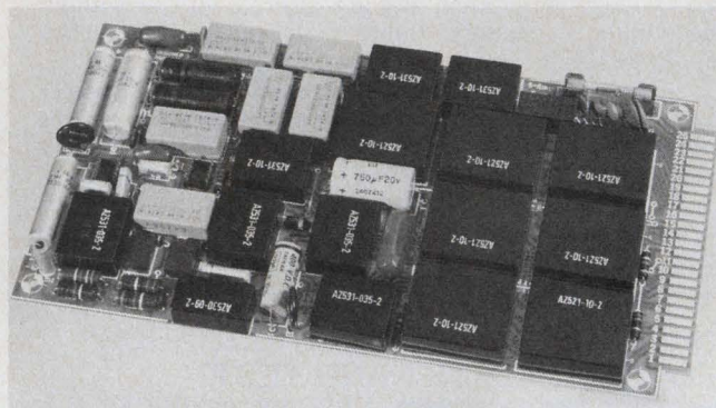
PC boards need skillful artwork to achieve high packaging density and a properly functioning circuit.
