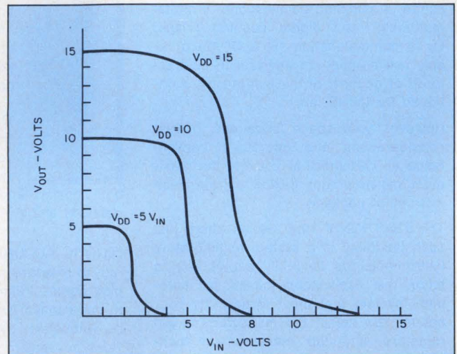
1. The threshold of a CMOS inverter remains nearly centered between supply-voltage limits, regardless of the actual supply voltage.
