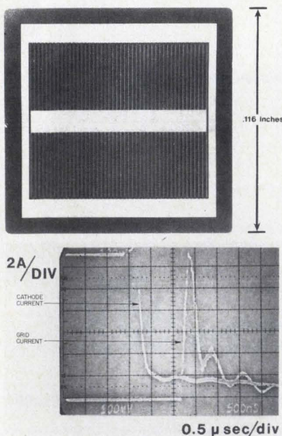
The cathode and grid structures of the General Electric FCT are highly interdigitated (top). Cathode current is interrupted by the grid control in 0.3 \mu\text{s} , as shown at bottom.
