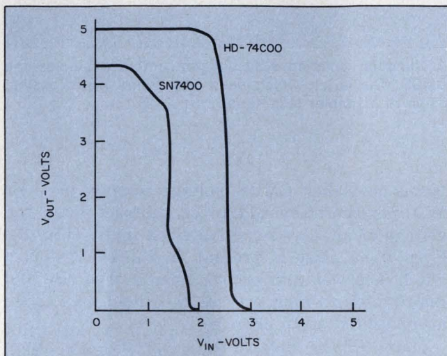
2. The improved transfer characteristics of CMOS over TTL can be seen from a comparison of the TTL SN7400 and CMOS HD74C00, shown for V_{DD} = V_{CC} = 5 V.
