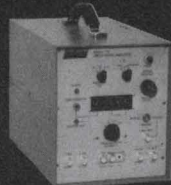
MODEL 710 OMEGA SIGNAL SIMULATOR Only instrument of its kind. Provides simulated OMEGA signals for checking performance of an OMEGA Navigation Receiver. Simple to operate. Portable. Internal frequency standard.
