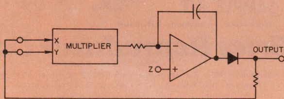
SQUARE ROOTER: V_{OUT} \cong \sqrt{Z}
