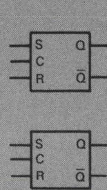
MC1666 (High Z) MC1667 (Low Z) Dual Clocked R-S Flip-Flop
