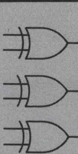
MC1672 (High Z) MC1673 (Low Z) Triple 2-Input Exclusive OR Gate
