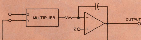
DIVIDER: V_{OUT} \cong Z/X
