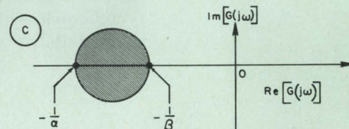
1. The circle criterion applies to systems like this (a) where f(e) is a memoryless nonlinear transfer function (b) and G(s) is the Laplace transform of the linear portion of the system. The prohibited region (c) is the circle centered between the points \text{Re}[G(j\omega)] = -1/\alpha and \text{Re}[G(j\omega)] = -1/\beta .
