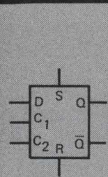
MC1670 (High Z) MC1671 (Low Z) Master Slave Type D Flip-Flop
