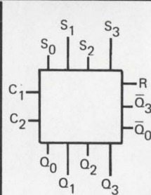
* MC1678 (High Z) MC1679 (Low Z) Bi-Quinary Counter
