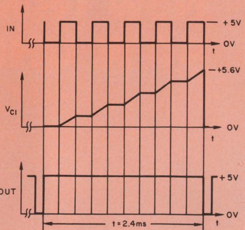
determined by the source Q_2 . A 15:1 frequency division can be obtained by this circuit.
