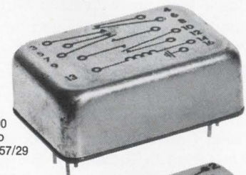
Series 500 Miniature: 1 Form A Case Size .280" x .330" x .750"
