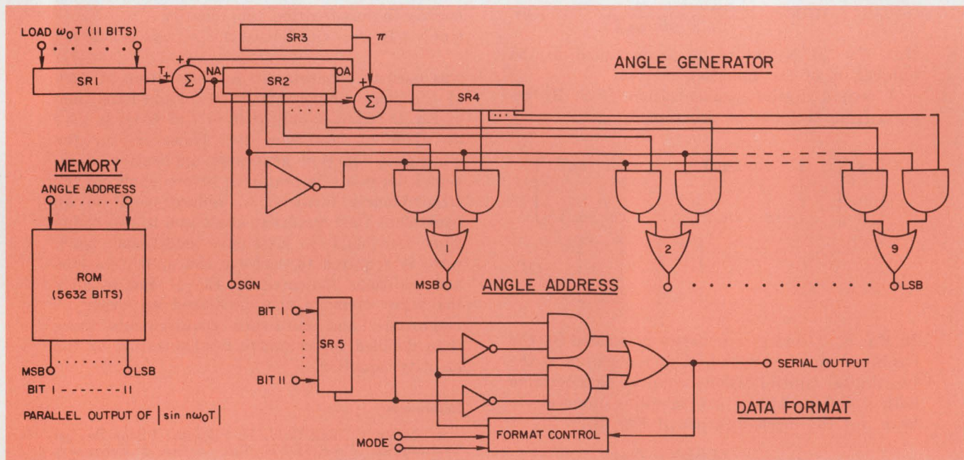
1. Round-off errors do not increase with time in this simplified sine-wave generator. The angle generator section reduces the angle generated to a first quadrant
