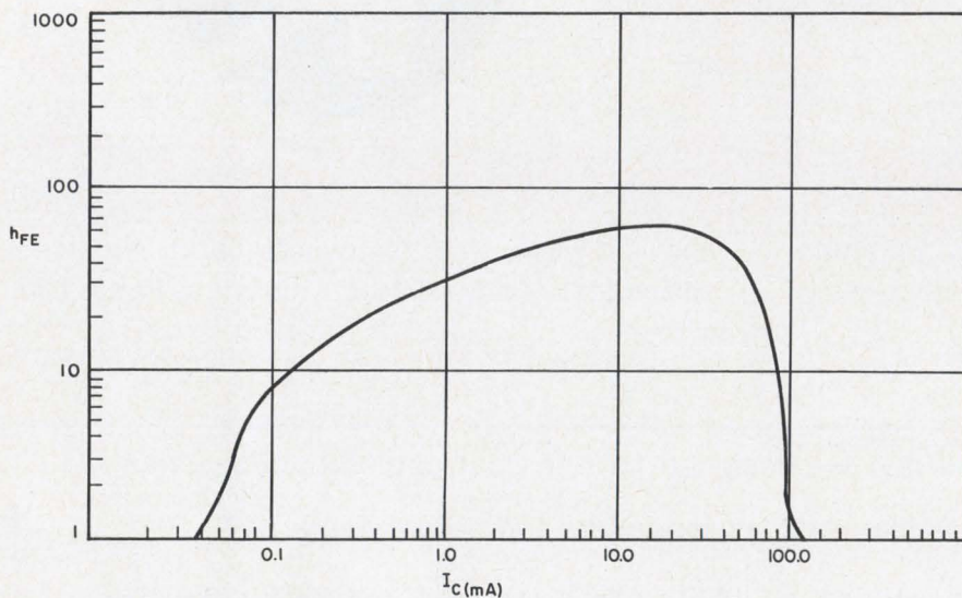
h_{FE} of 500-V device reaches 60 at a 10-mA collector current.
