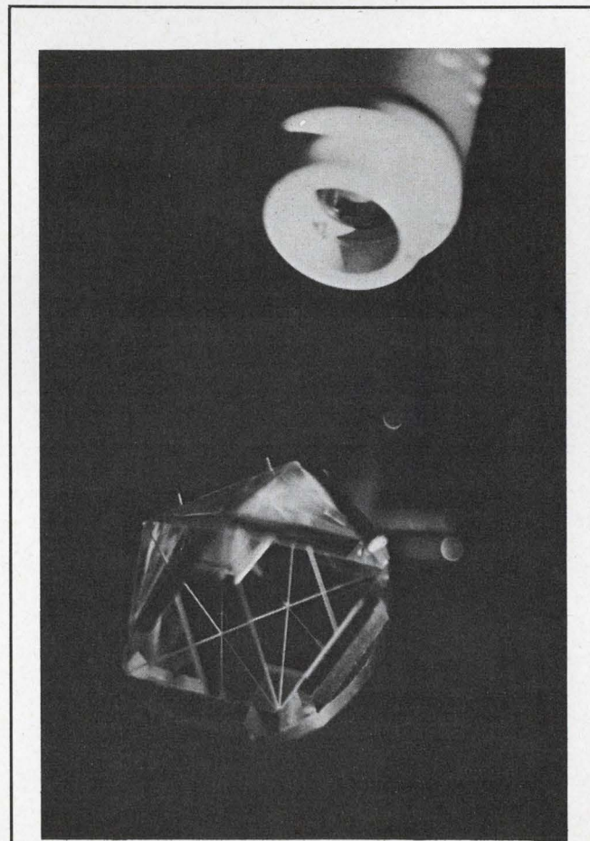
Five-corner cube reflector , designed for laser trackers, returns the light beams at the path of incidence. Its sphere-like behavior enables engineers to track missiles, airplanes or spacecraft without fear of losing the target. (Perkin-Elmer, Inc.)
