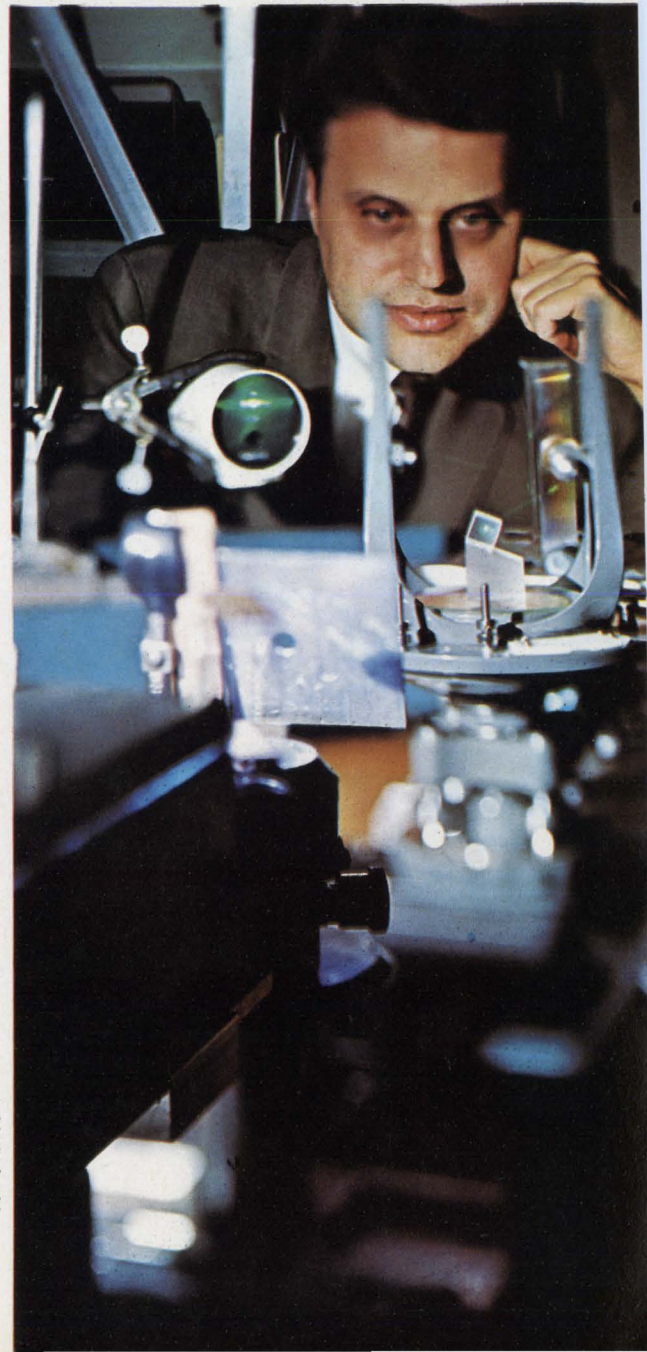
An early model of an ionized argon laser is adjusted by scientists of Electro-Optical Systems, Inc. This unit produced about 4.5 watts during continuous-wave operation. With a ceramic laser tube, advance devices produce about 3 watts continuous wave. These are being built under a classified military contract.
