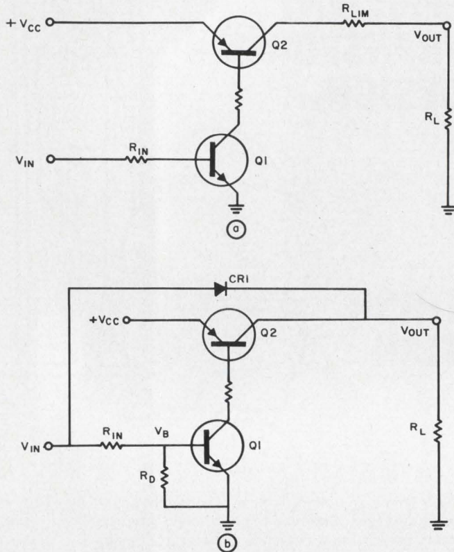
Current-limiting series resistor, R_{LIM} , is eliminated from the output line (a) by using diode feedback element (b). As output goes to ground, V_{IN} limits at 0.7 V and V_B becomes 0.3 V, turning Q1, and subsequently Q2, OFF.
