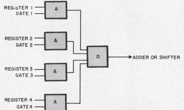
4. In-gates to an adder or shifter
