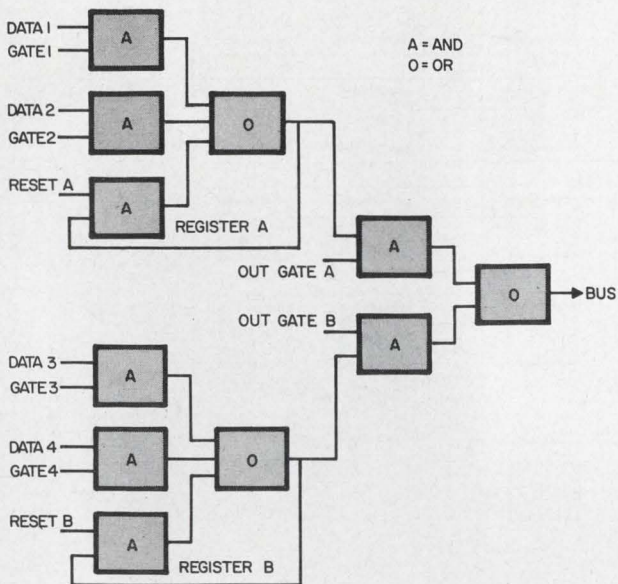
1. Data path register pair, out-gated and ORed
