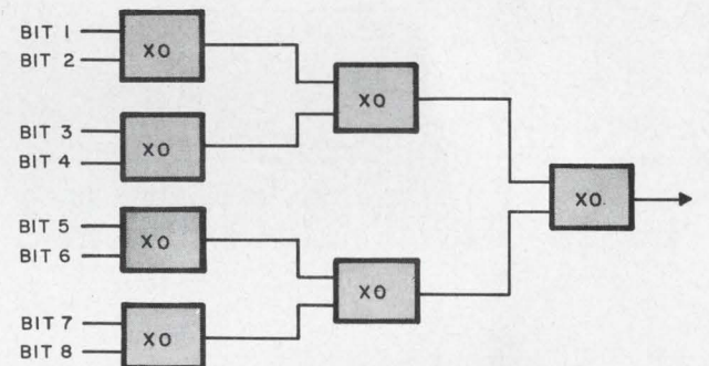
5. Eight-bit parity tree for checking
