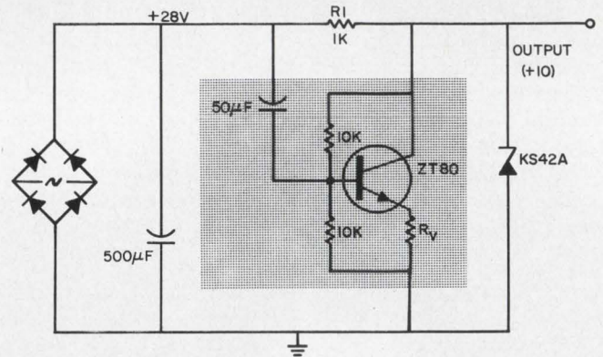
Shunt circuit serves to smooth output fluctuations in this power supply.
