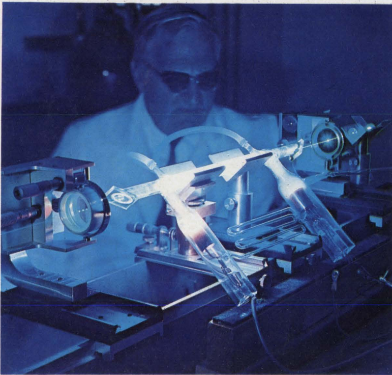
An early model of an ionized argon laser is adjusted by scientists of Electro-Optical Systems, Inc. This unit produced about 4.5 watts during continuous-wave operation. With a ceramic laser tube, advance devices produce about 3 watts continuous wave. These are being built under a classified military contract.
