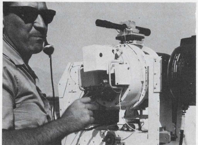
6. Feasibility of optical radars has been demonstrated with the Sperry system. The range and range rate data are presented in digital form.
