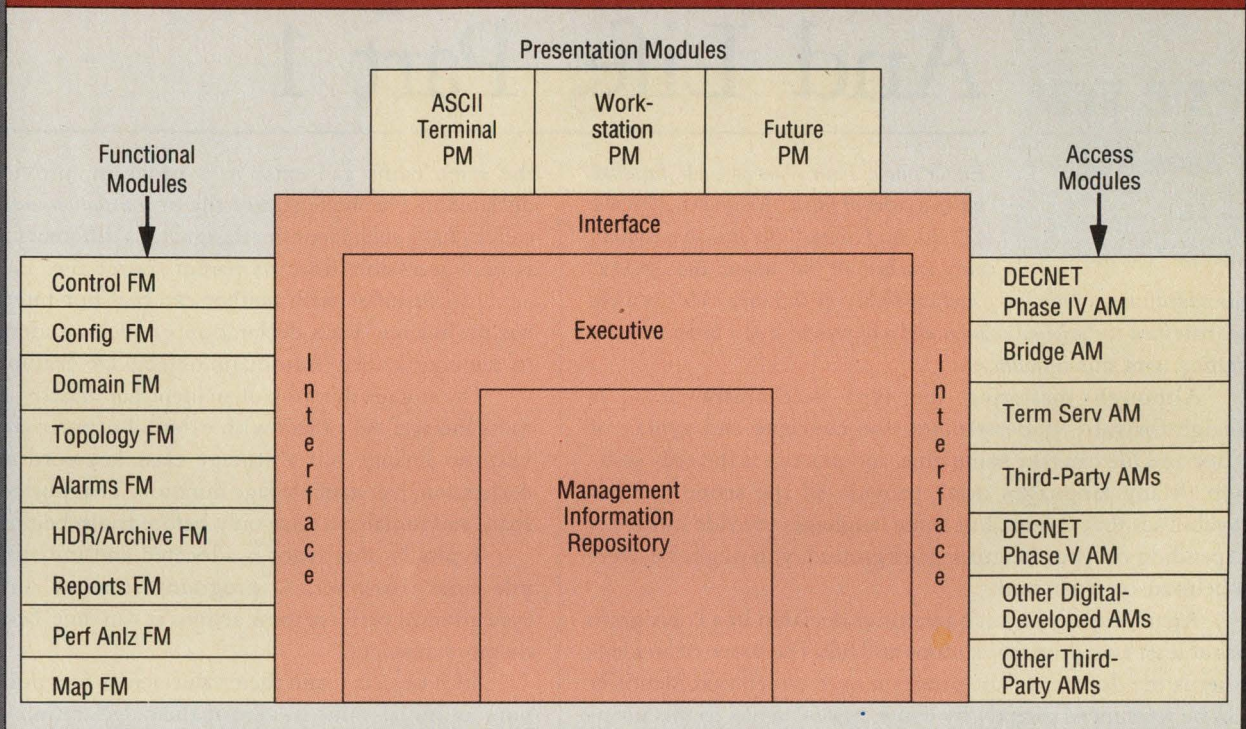
DEC's Network Enterprise Management Architecture.
