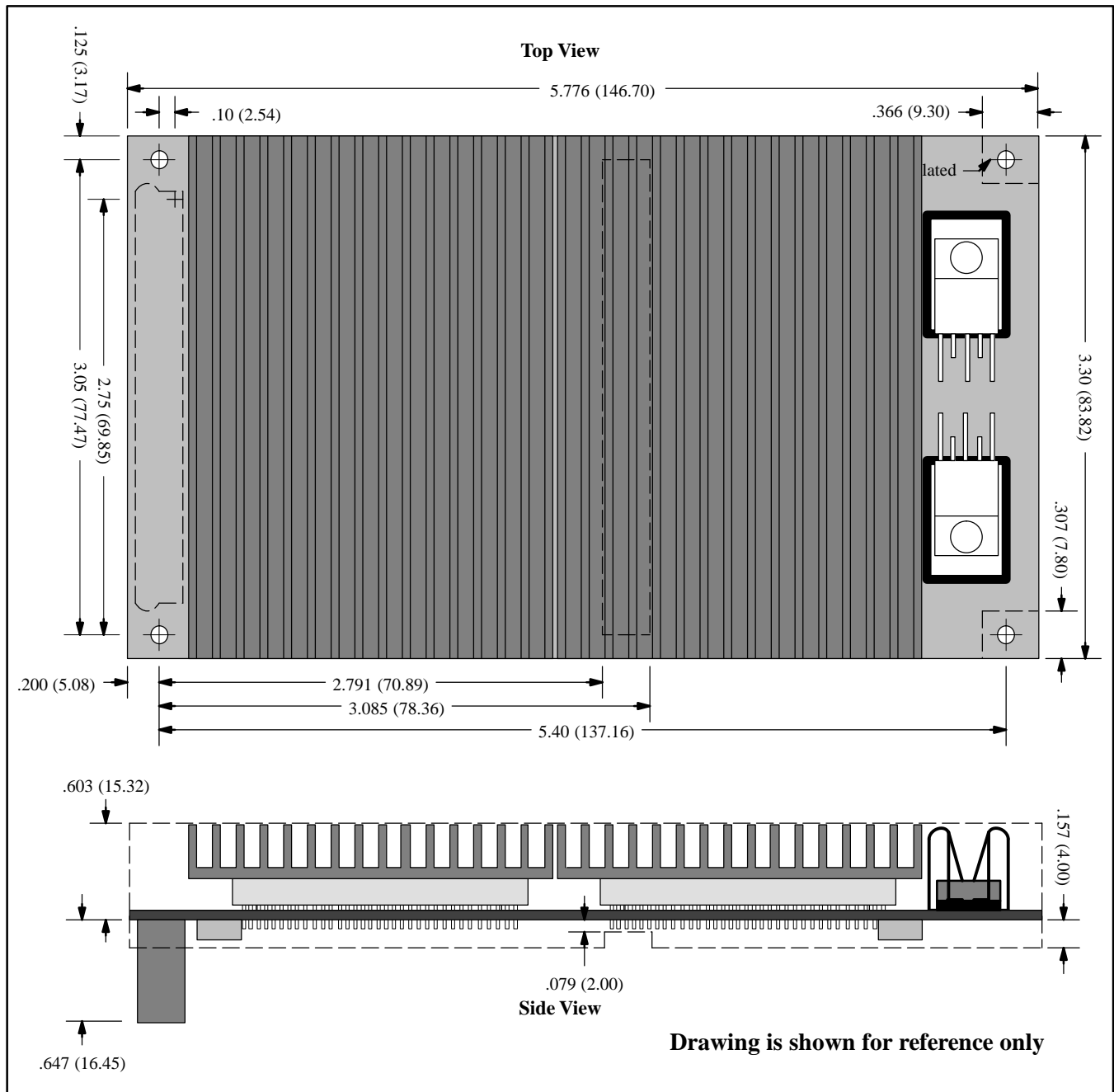
Figure 6. RT6226K Mechanical Dimensions
