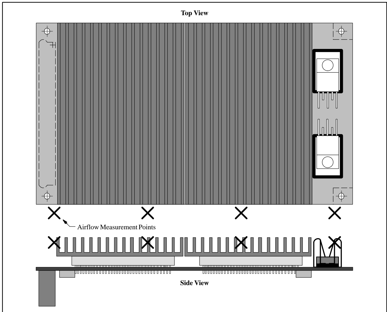
Figure 8. RT6226K Airflow Measurement
