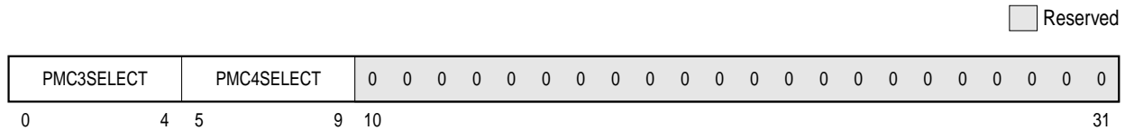
Figure 2-7. Monitor Mode Control Register 1 (MMCR1)
