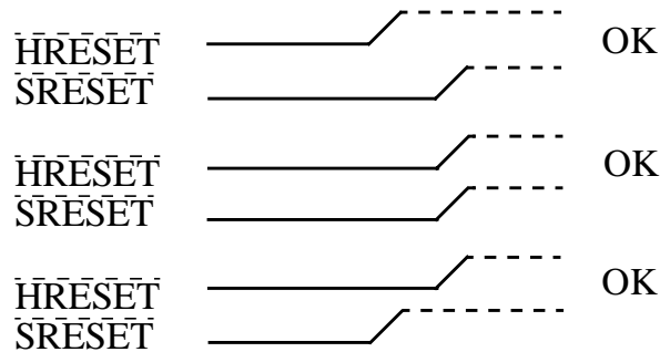
Figure 4-4. SRESET Asserted During HRESET
