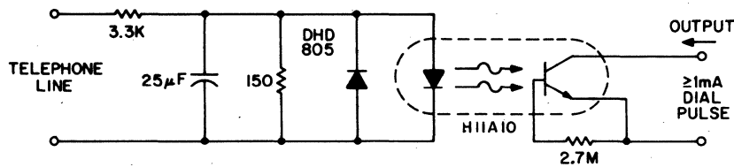
FIGURE 6.37: DIAL PULSE INDICATOR
