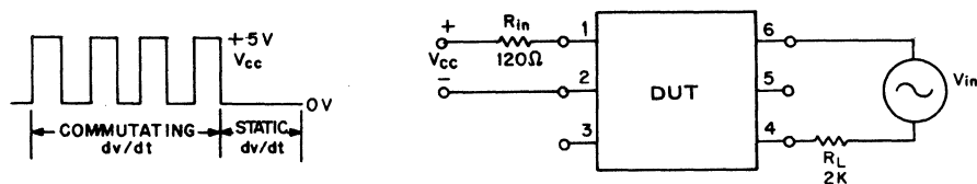
FIGURE 1. dv/dt — TEST CIRCUIT
