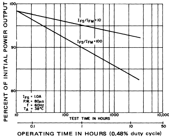
FIGURE 3.9: GaAs IRED PULSED OPERATION
