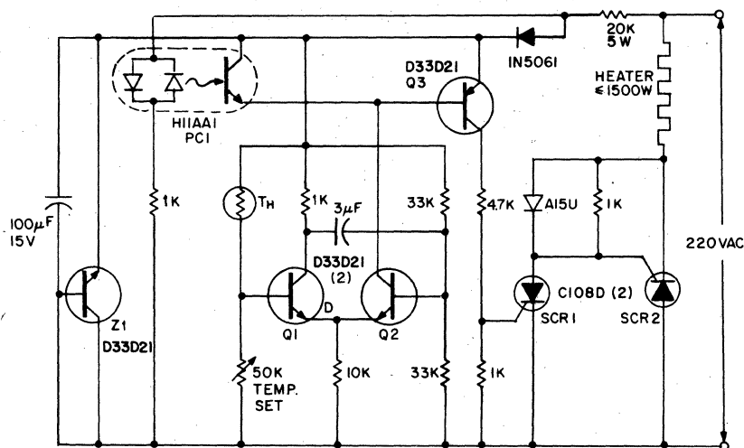
FIGURE 6.83: LOW POWER (>50W) ZVS PROPORTIONAL TEMPERATURE CONTROLLER
