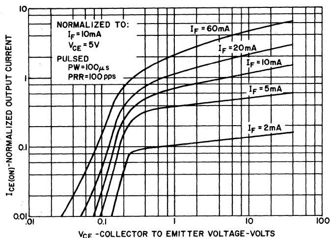
4. OUTPUT CHARACTERISTICS
