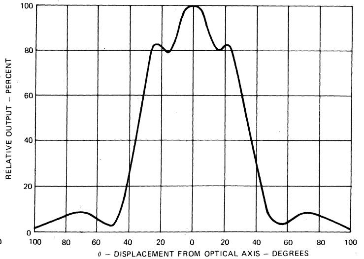
6. TYPICAL RADIATION PATTERN
