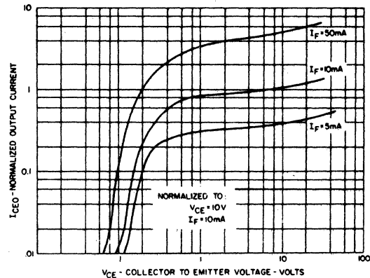
OUTPUT CHARACTERISTICS
