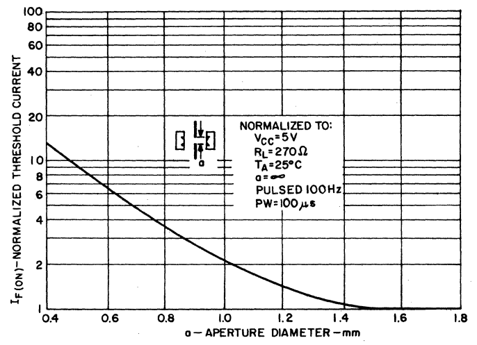
6. THRESHOLD CURRENT VS. APERTURE DIAMETER
