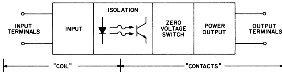
FIGURE 6.42: SOLID STATE RELAY BLOCK DIAGRAM
