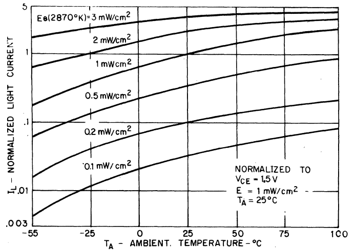
2. LIGHT CURRENT VS. AMBIENT TEMPERATURE
