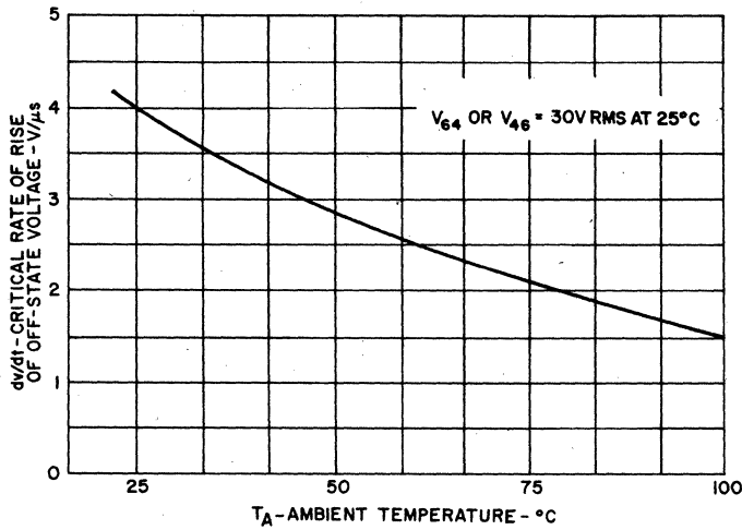
FIGURE 5. dv/dt VS. TEMPERATURE
