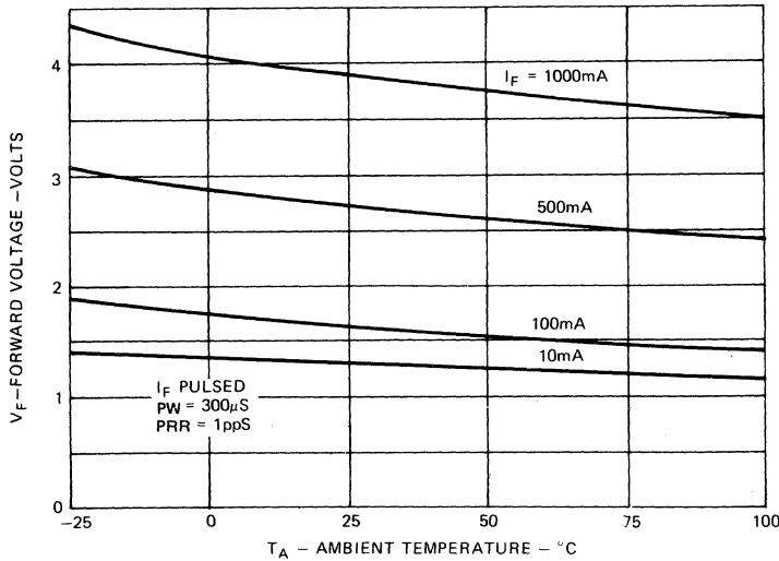
3. FORWARD VOLTAGE VS. TEMPERATURE
