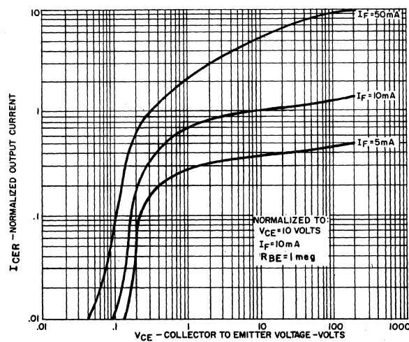
4. OUTPUT CHARACTERISTICS
