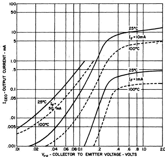
6. OUTPUT CHARACTERISTICS
