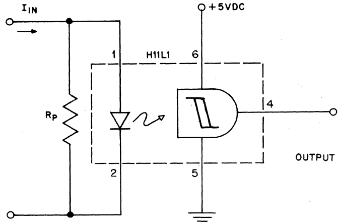
PROGRAMMABLE CURRENT THRESHOLD SENSING CIRCUIT
