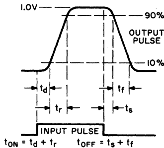
6. WAVE FORMS
