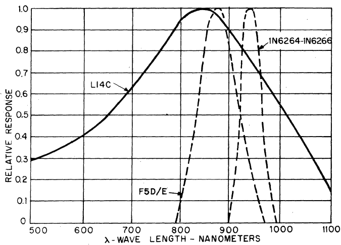
SPECTRAL RESPONSE
