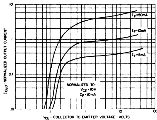
OUTPUT CHARACTERISTICS
