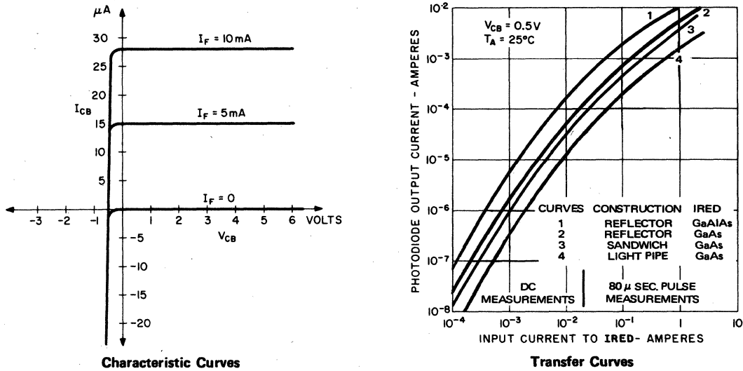
FIGURE 2.25: TYPICAL OPTOCOUPLER TRANSFER CHARACTERISTICS — PHOTODIODE RESPONSE OF PHOTOTRANSISTOR AND PHOTODARLINGTON COUPLERS
