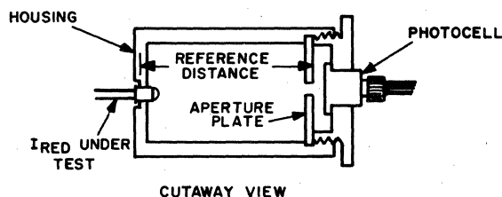
FIGURE 4.2 RADIANT INTENSITY TEST FIXTURE
