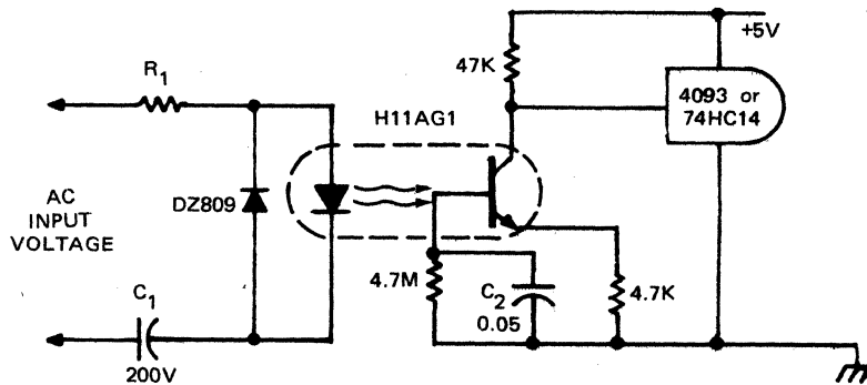
TELEPHONE RING DETECTOR/A.C. LINE CMOS INPUT ISOLATOR
