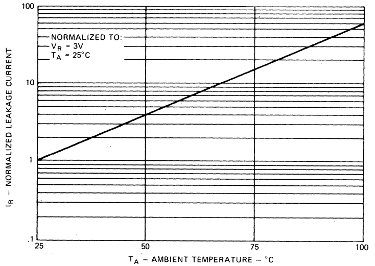
4. LEAKAGE CURRENT VS. TEMPERATURE
