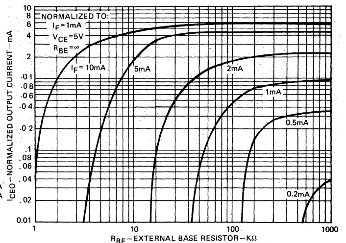
OUTPUT CURRENT VS. BASE EMITTER RESISTANCE
