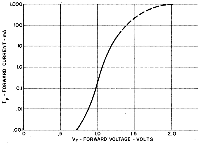
3. INPUT CHARACTERISTICS
