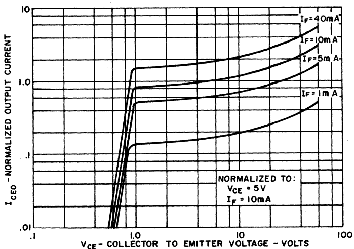
4. OUTPUT CHARACTERISTICS
