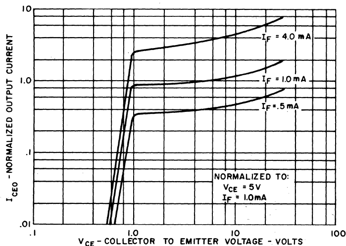
OUTPUT CHARACTERISTICS
