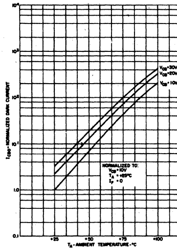
4. I_{CBO} VS TEMPERATURE
