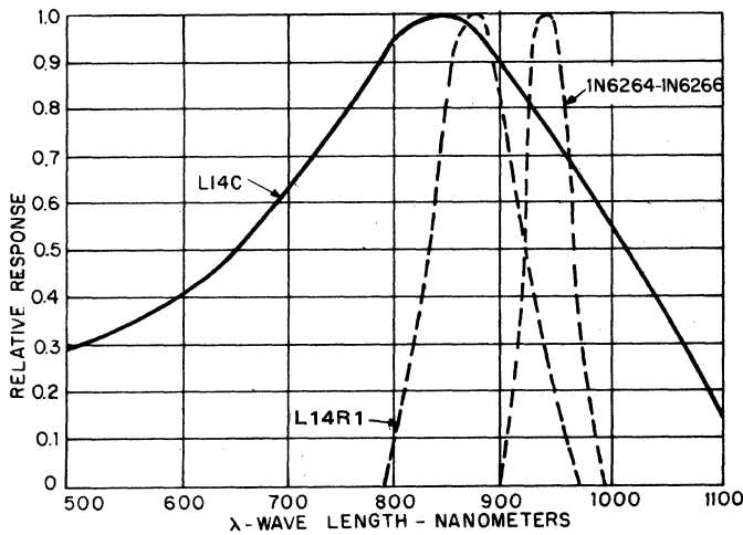
5. SPECTRAL RESPONSE
