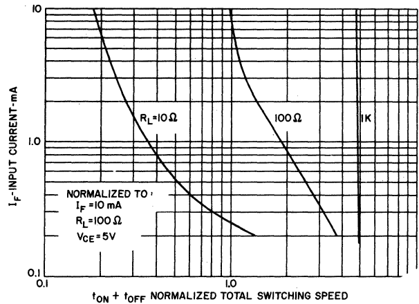
SWITCHING SPEED
