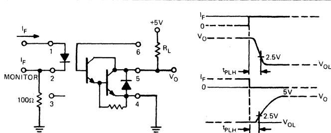
SWITCHING TEST CIRCUIT
