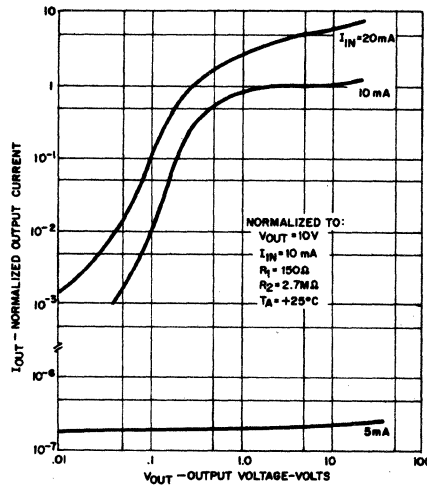
4. INPUT CURRENT
