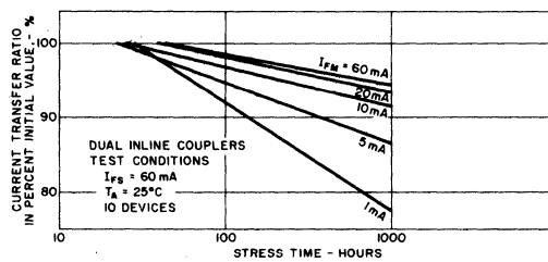
FIGURE 3.7a: EFFECT OF MEASUREMENT CURRENT ON SLOPE
