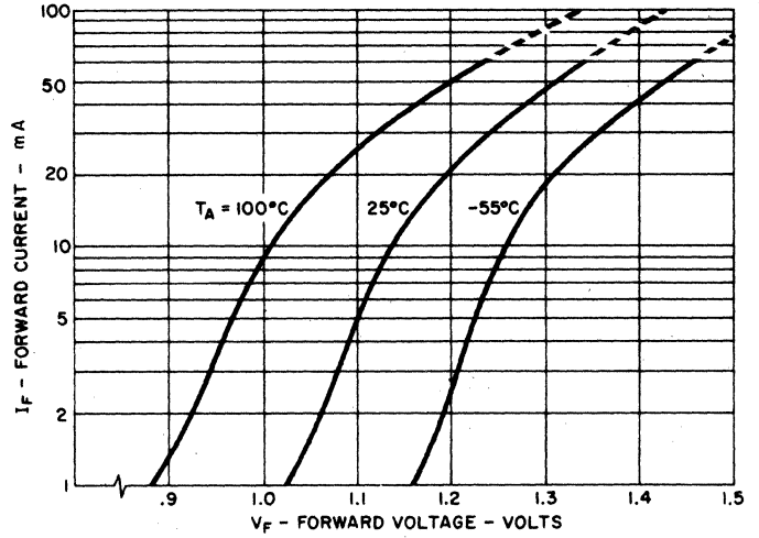
FIGURE 2. FORWARD VOLTAGE VS. FORWARD CURRENT
