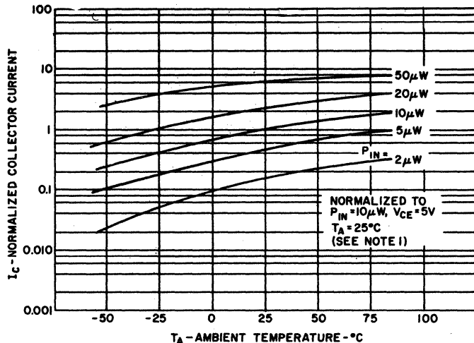
2. COLLECTOR VS. TEMPERATURE
