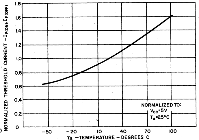
THRESHOLD CURRENTS VS. TEMPERATURE
