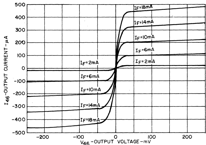
2. OUTPUT CHARACTERISTICS
