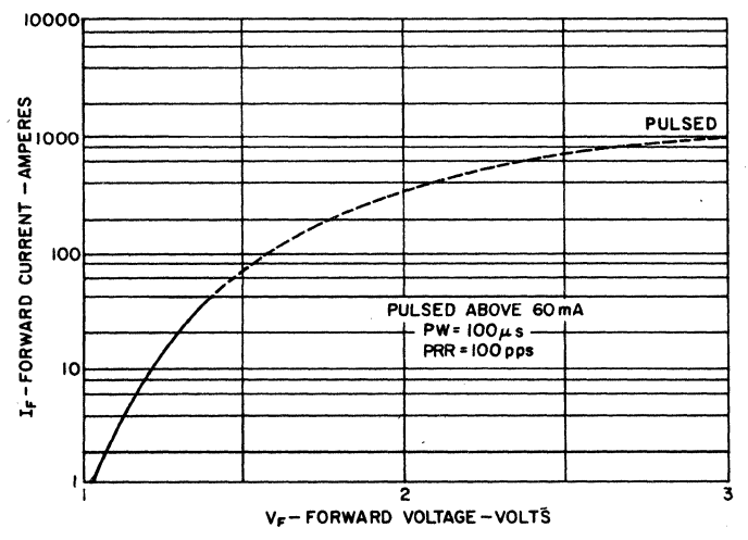
3. INPUT CHARACTERISTICS
