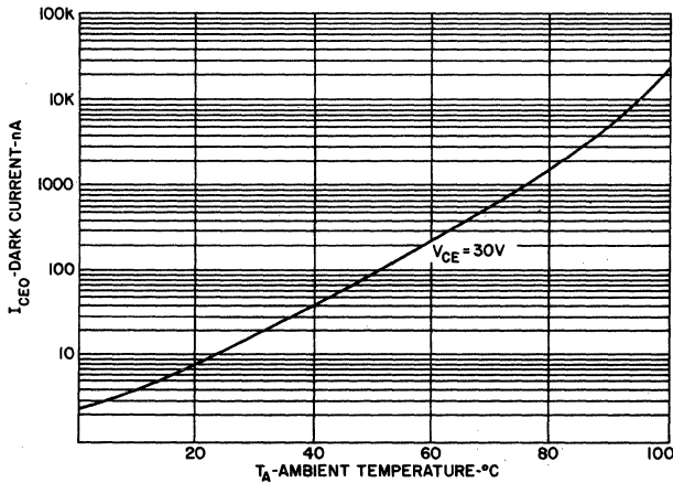
DARK CURRENT
