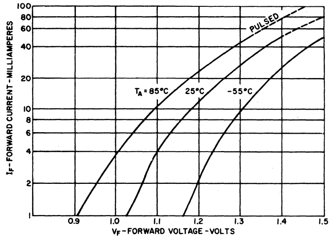
4. FORWARD VOLTAGE VS. FORWARD CURRENT
