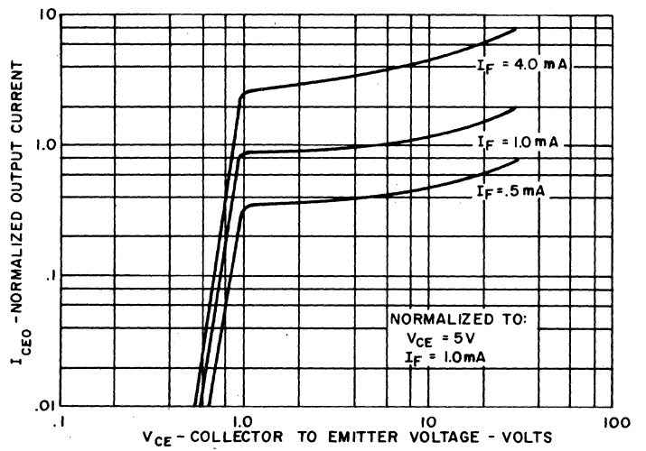
OUTPUT CHARACTERISTICS
