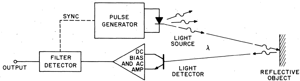
FIGURE 2.13: TYPICAL PULSED REFLECTIVE OBJECT SENSOR
