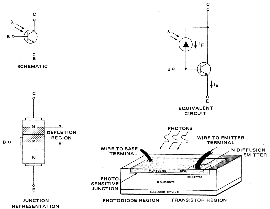
FIGURE 1.3: LIGHT GENERATED CURRENT IN PHOTOTRANSISTOR
