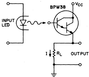
5. TEST CIRCUIT
