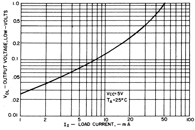
3. ON VOLTAGE VS. LOAD CURRENT
