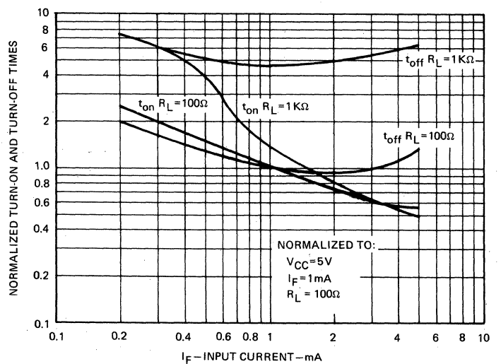
SWITCHING TIMES VS. INPUT CURRENT
