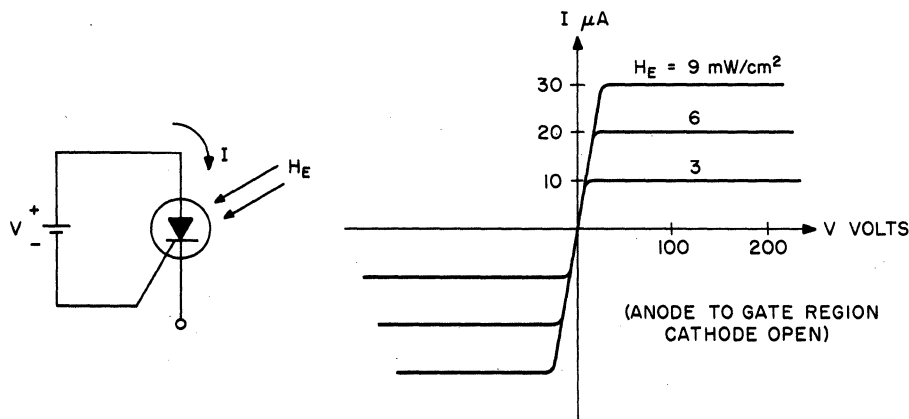
FIGURE 1.8: TYPICAL PNP PHOTOTRANSISTOR ACTION OF LASCR
