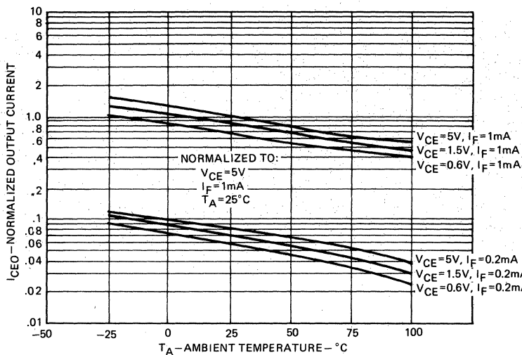
OUTPUT CURRENT VS. TEMPERATURE
