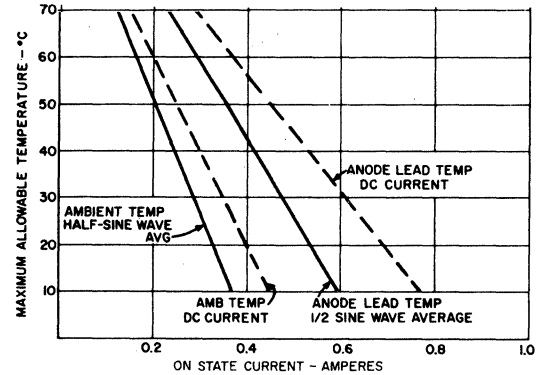
FIGURE 4. ON-STATE CURRENT VS. MAXIMUM ALLOWABLE TEMPERATURE
