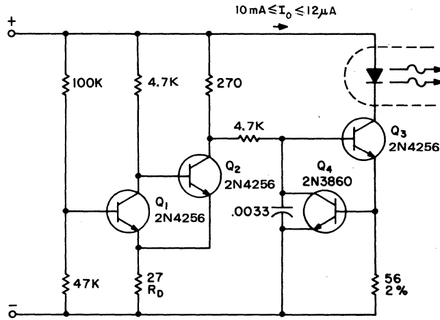
FIGURE 6.45: HYSTERESIS INPUT CIRCUIT
