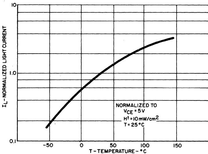
NORMALIZED LIGHT CURRENT VS TEMPERATURE
