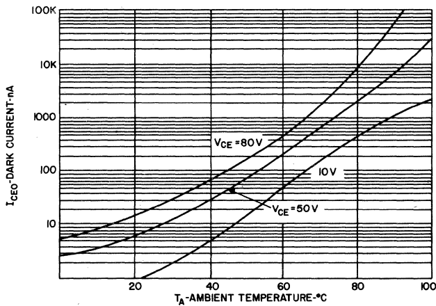
DARK CURRENT
