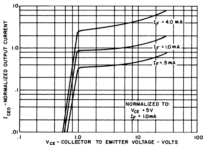
OUTPUT CHARACTERISTICS
