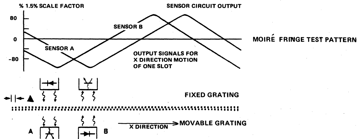
FIGURE 2.15: MOIRÉ FRINGE TEST PATTERN
