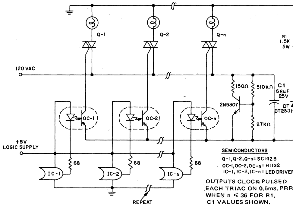
FIGURE 6.59: MICROPROCESSOR TRIAC ARRAY DRIVER
