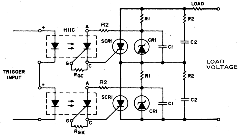
FIGURE 6.66: HIGH VOLTAGE SWITCH
