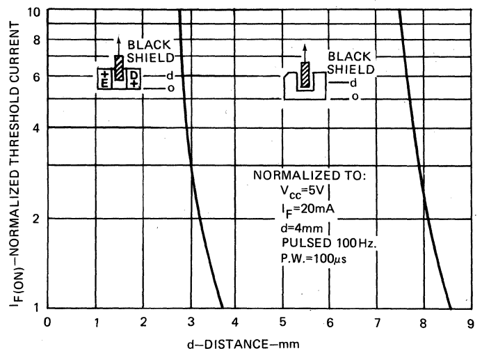
THRESHOLD CURRENT VS. SHIELD DISTANCE
