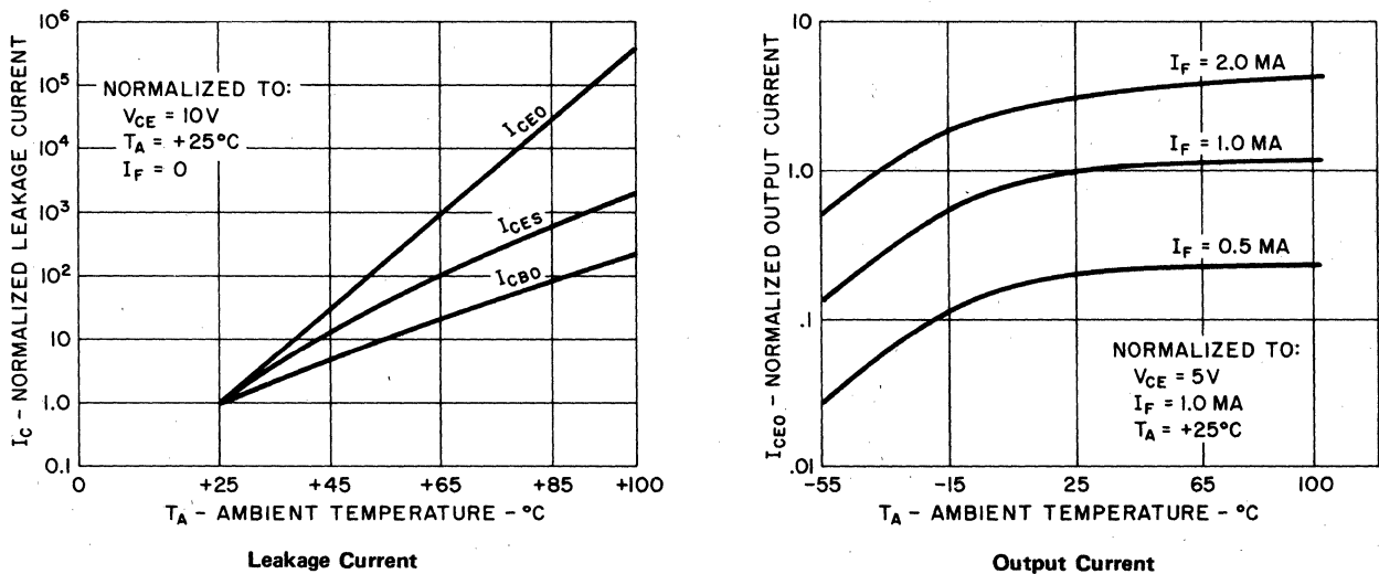
FIGURE 2.32: TYPICAL TEMPERATURE EFFECTS ON PHOTODARLINGTON OUTPUT
