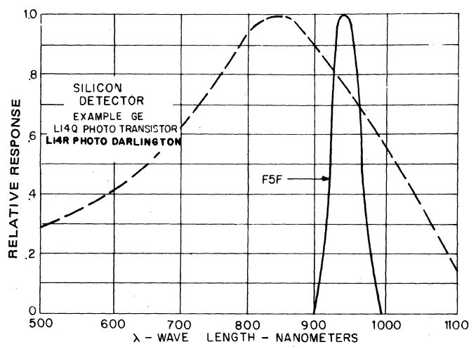
5. SPECTRAL RESPONSE
