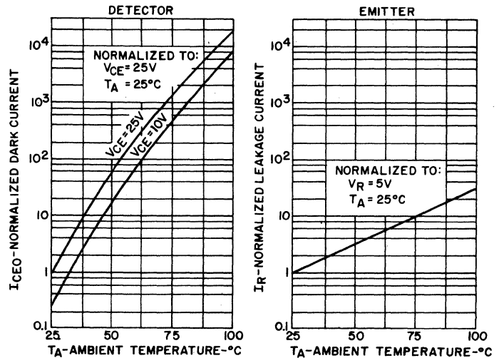
4. LEAKAGE CURRENTS VS. TEMPERATURE
