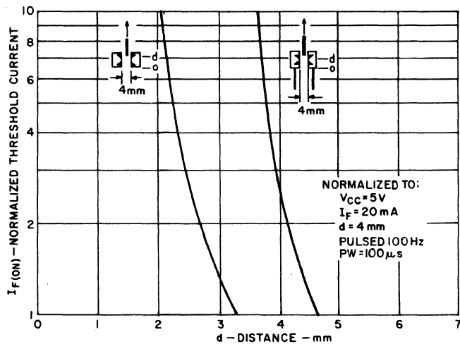
9. THRESHOLD CURRENT VS. SHIELD DISTANCE
