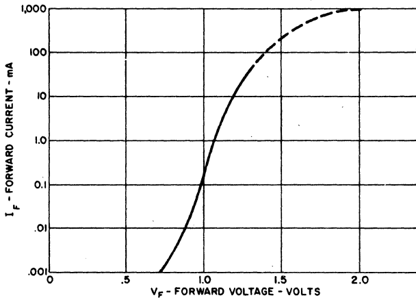
INPUT CHARACTERISTICS
