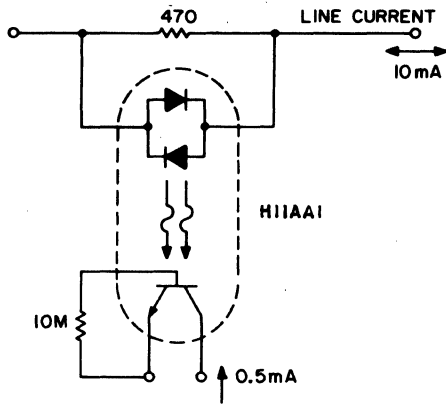
FIGURE 6.34: POLARITY INSENSITIVE LINE CURRENT DETECTOR
