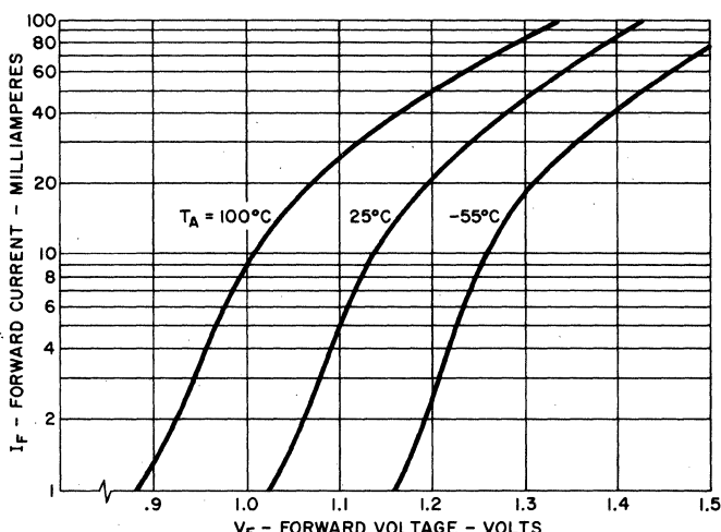
4. FORWARD VOLTAGE VS. FORWARD CURRENT
