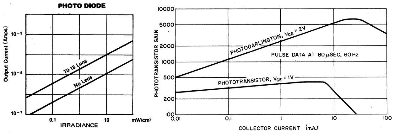
FIGURE 2.6: TYPICAL PHOTODETECTOR CURRENT AND GAIN
