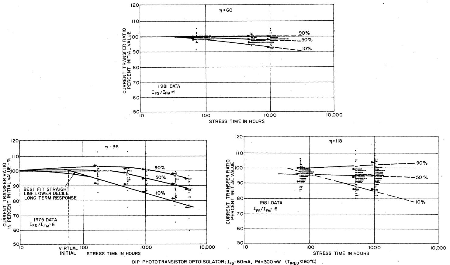
FIGURE 3.5: LIFE TEST RESULTS — ILLUSTRATING OBSERVED CHANGE IN IRED OUTPUT WITH OPERATING TIME
