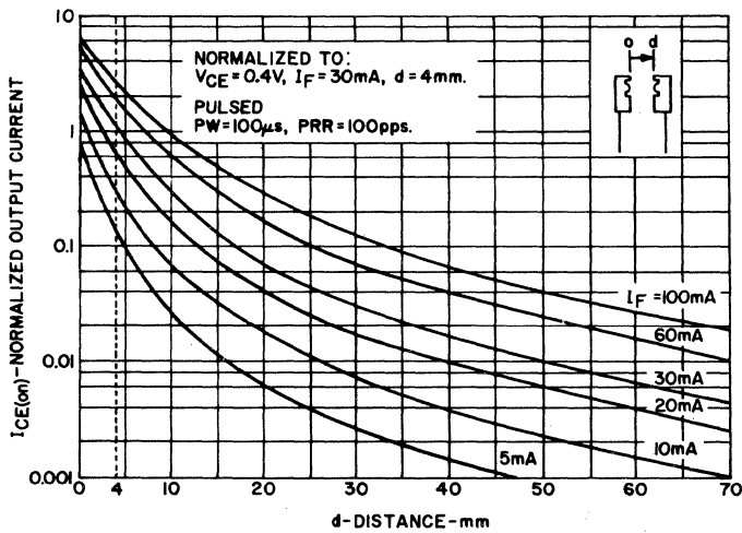
3. OUTPUT CURRENT VS. DISTANCE
