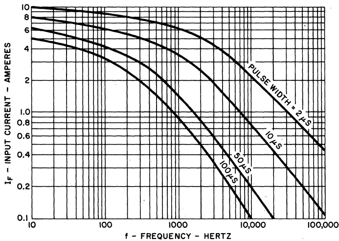
MAXIMUM PULSE CAPABILITY
