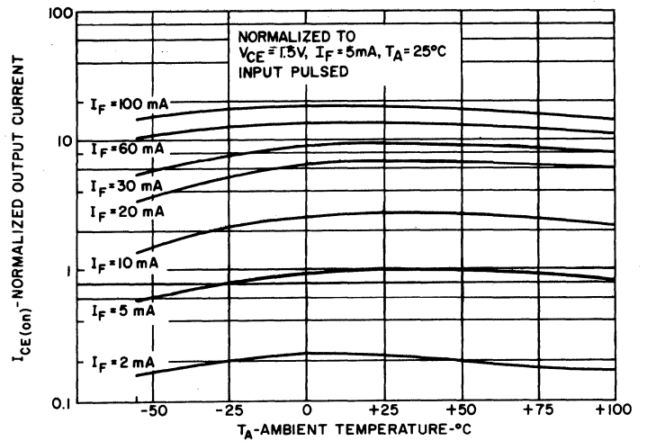
2. OUTPUT CURRENT VS. TEMPERATURE
