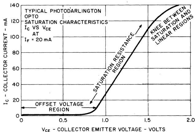
FIGURE 2.34: TYPICAL PHOTODARLINGTON OPTOCOUPLER SATURATION CHARACTERISTICS
