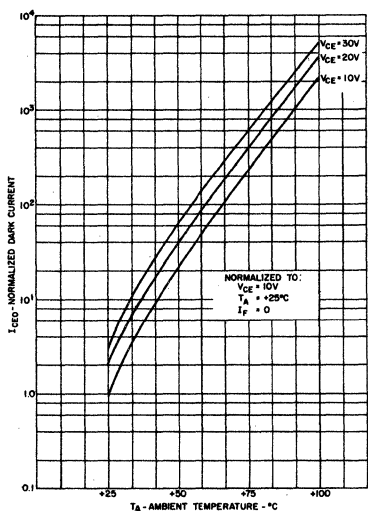
3. DARK I_{CE0} CURRENT VS. TEMPERATURE
