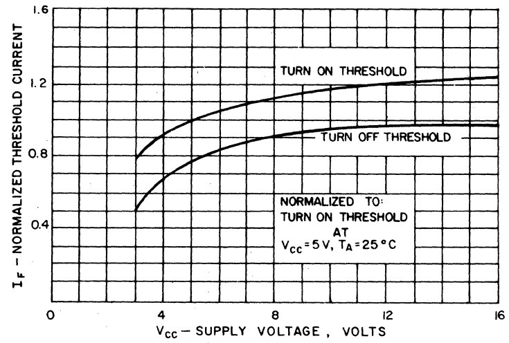
5. THRESHOLD CURRENT VS. SUPPLY VOLTAGE
