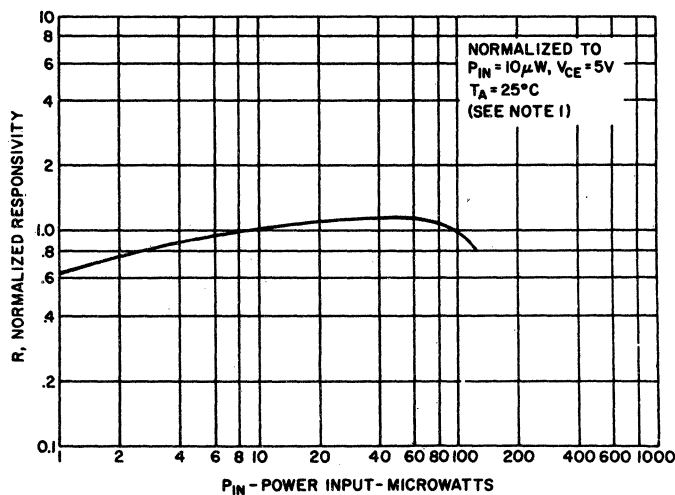
4. RESPONSIVITY VS. POWER INPUT
