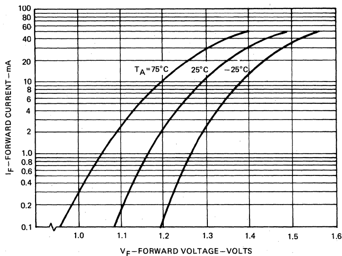
INPUT VOLTAGE VS. INPUT CURRENT
