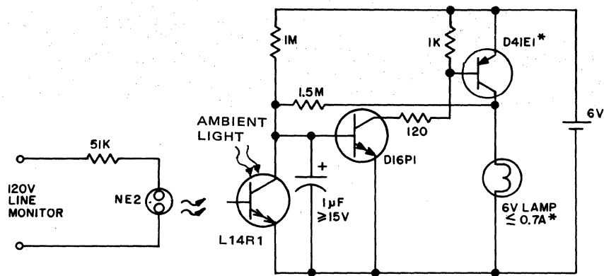
FIGURE 6.7: LINE OPERATED POWER OUTAGE LIGHT
