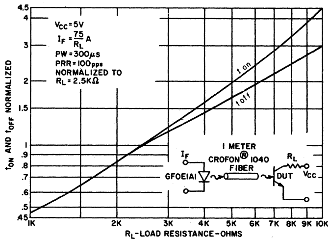
5. SWITCHING SPEED VS. RL
