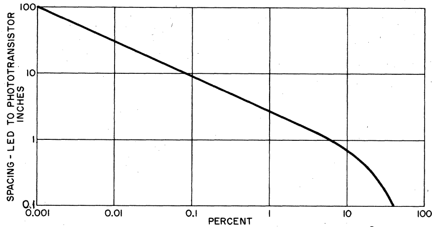
FIGURE 2.4: LENSED LED TO PHOTOTRANSISTOR COUPLING CHART
