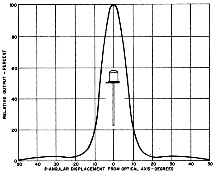
5. 1N6264 - TYPICAL RADIATION PATTERN
