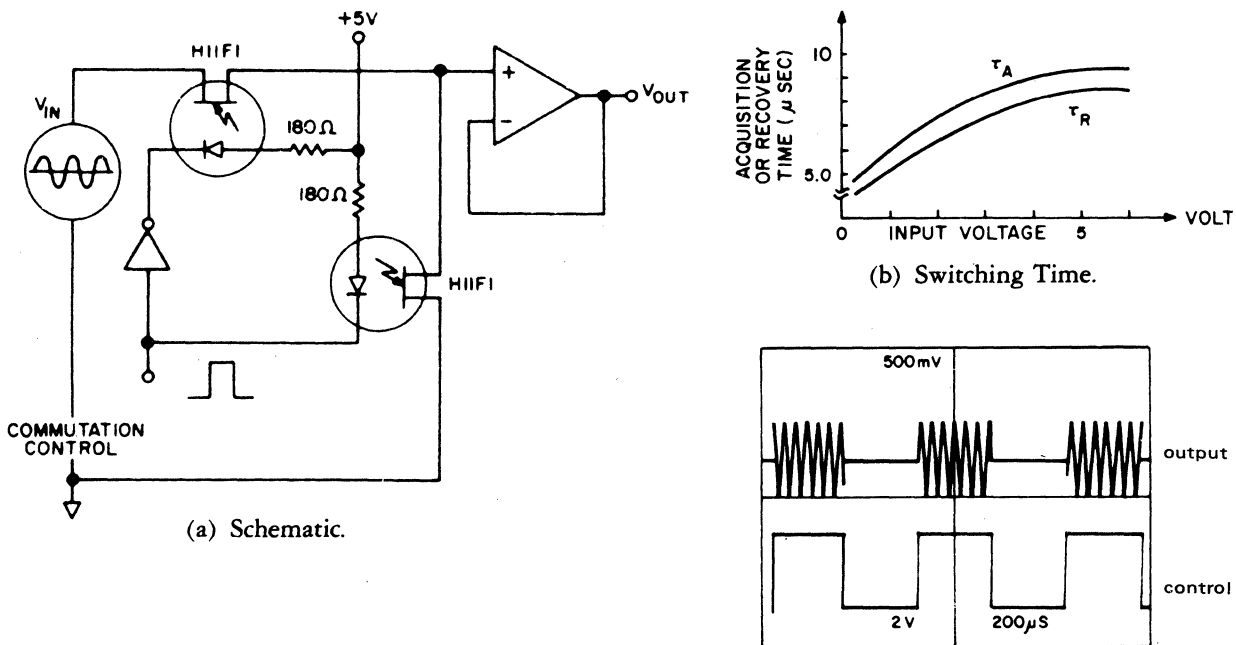
FIGURE 6.39: ANALOG COMMUTATOR CIRCUIT
