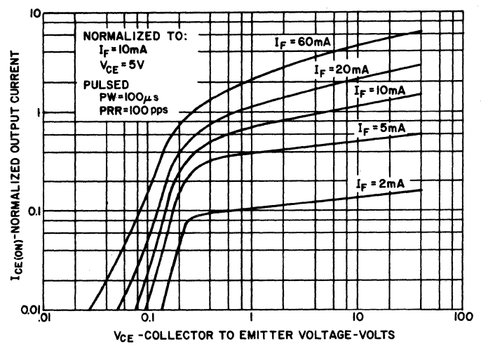
4. OUTPUT CHARACTERISTICS
