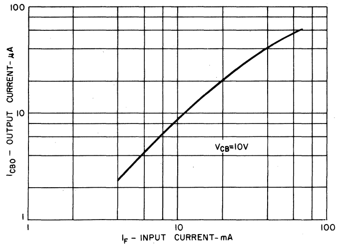
OUTPUT CURRENT ( I_{CBO} ) VS. INPUT CURRENT
