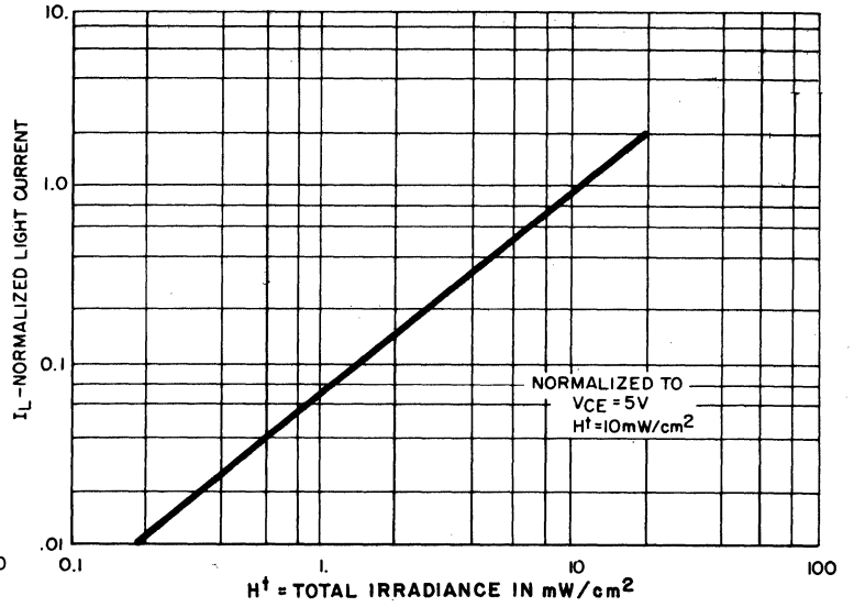
NORMALIZED LIGHT CURRENT VS RADIATION
