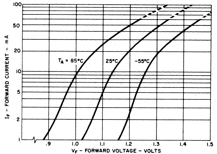
2. FORWARD VOLTAGE VS. FORWARD CURRENT
