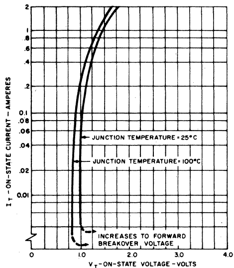
FIGURE 12. ON-STATE CHARACTERISTICS
