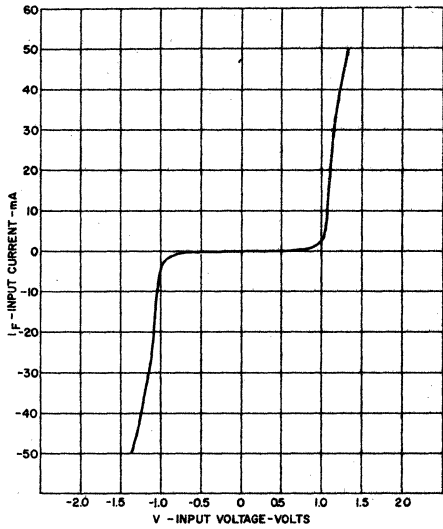
1. INPUT CHARACTERISTICS
