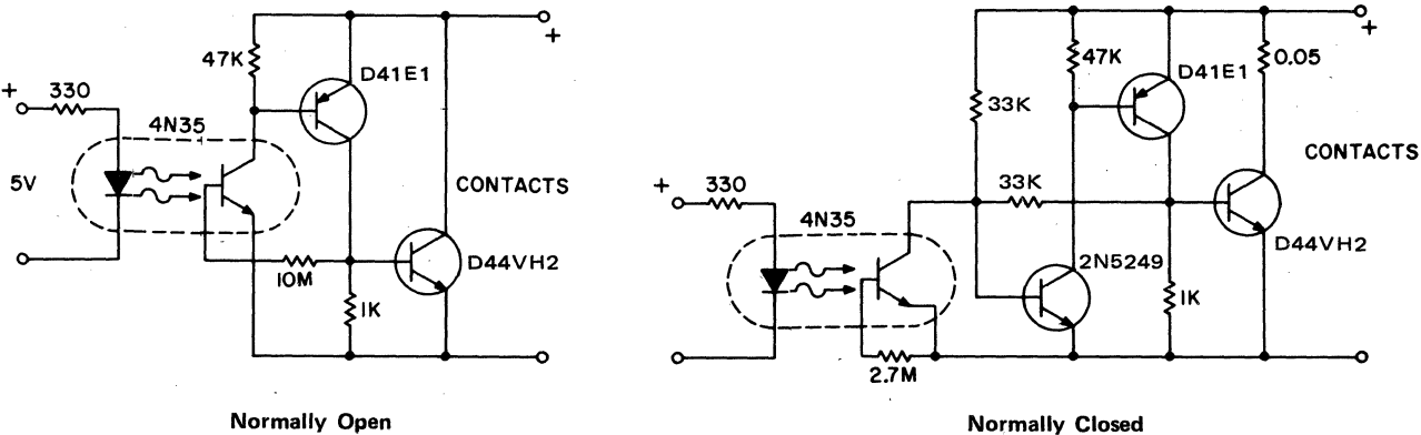
FIGURE 6.74: 10A, 25V DC SOLID STATE RELAYS
