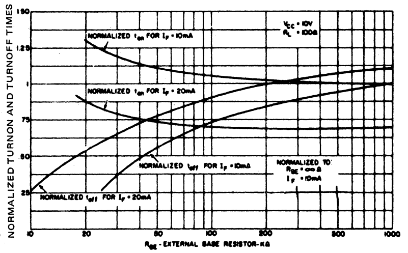
FIGURE 3. SWITCHING TIME VS. R BE
