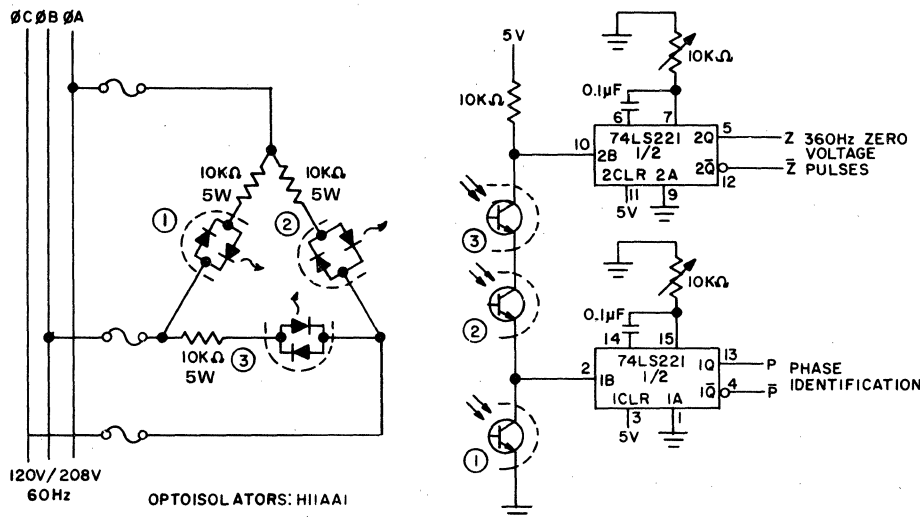
FIGURE 6.41: THREE PHASE LINE SYNCHRONIZER
