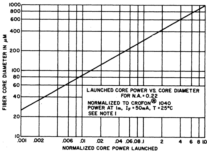
5. POWER OUTPUT VS. FIBER DIAMETER
