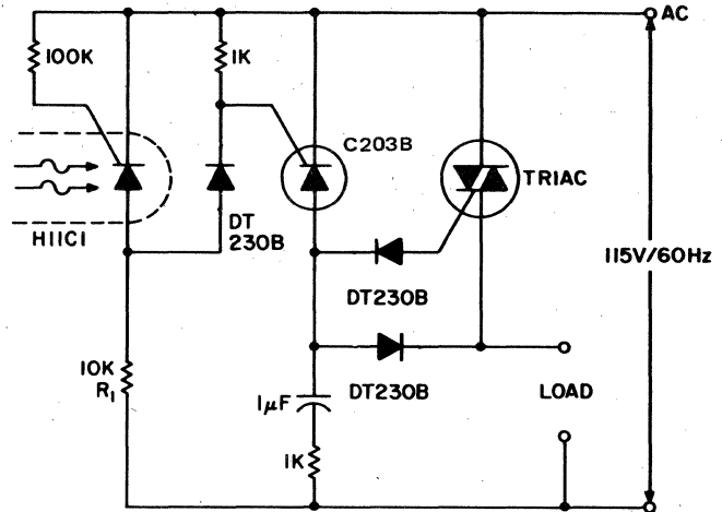
FIGURE 6.53: NORMALLY CLOSED INTEGRAL CYCLE, ZERO VOLTAGE SWITCHING, CONTACT CIRCUIT
