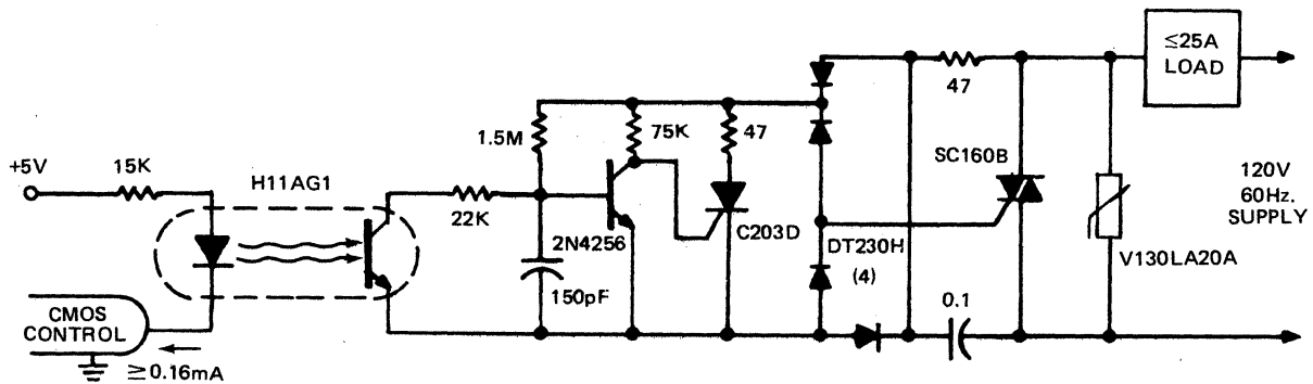
CMOS INPUT, 3KW, ZERO VOLTAGE SWITCHING SOLID STATE RELAY
