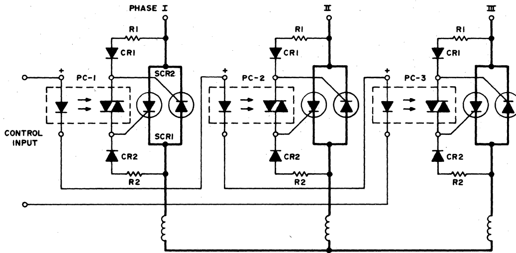
FIGURE 6.71: THREE PHASE SWITCH WITH INVERSE PARALLEL SCR'S FOR INDUCTIVE LOAD AND Y OR Δ CONNECTIONS
