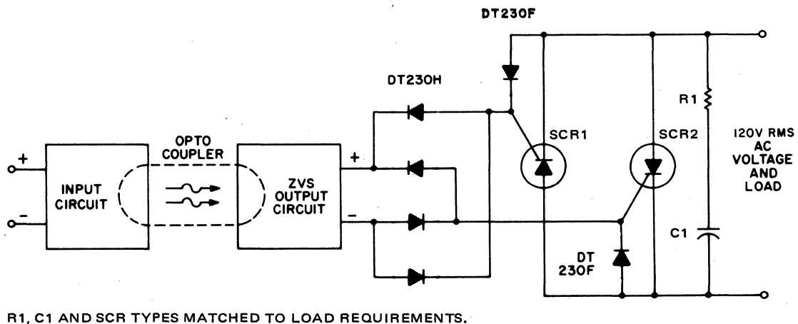
FIGURE 6.51: ZERO VOLTAGE SWITCHING, SOLID STATE RELAY WITH ANTIPARALLEL SCR OUTPUT
