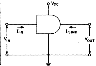
FIGURE 6.26: CHARACTERISTICS REQUIRED OF TTL GATES WHICH ARE TO BE INTERFACED BY H74 SERIES
