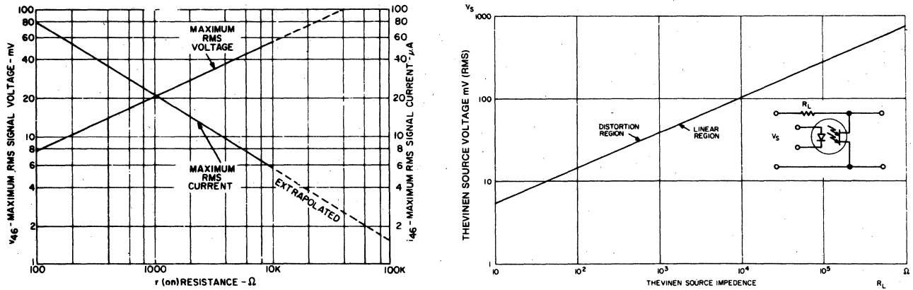
FIGURE 2.38: H11F BIAS LIMITS FOR LINEAR CONDUCTION
