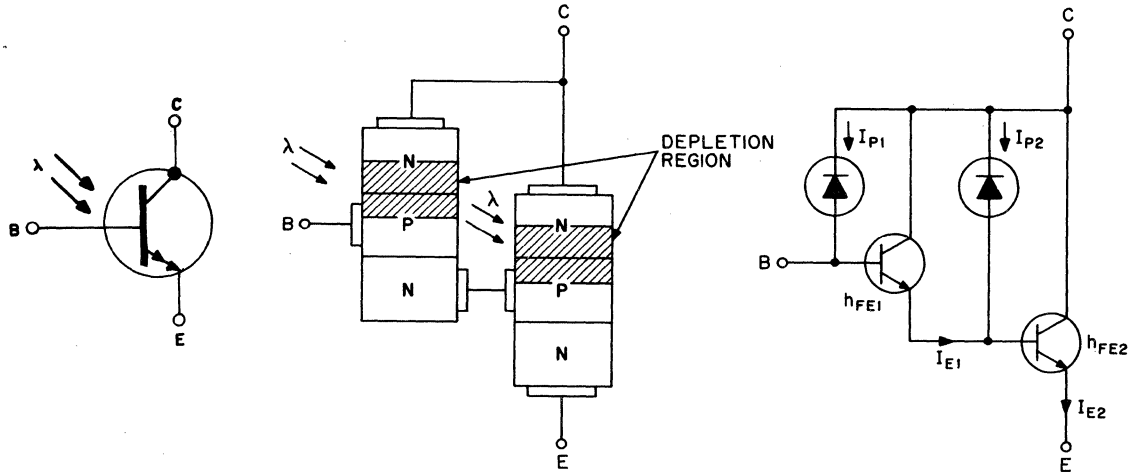
FIGURE 1.6: PHOTO DARLINGTON AMPLIFIER ILLUSTRATING THE EFFECTS OF PHOTON CURRENT GENERATION
