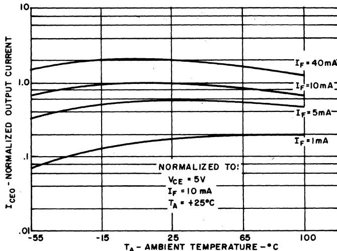
2. OUTPUT CURRENT VS. TEMPERATURE
