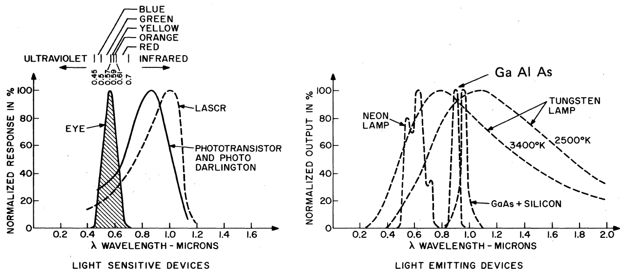
FIGURE 2.1: NORMALIZED SPECTRAL CHARACTERISTICS OF LIGHT SENSITIVE AND LIGHT EMITTING DIODES
