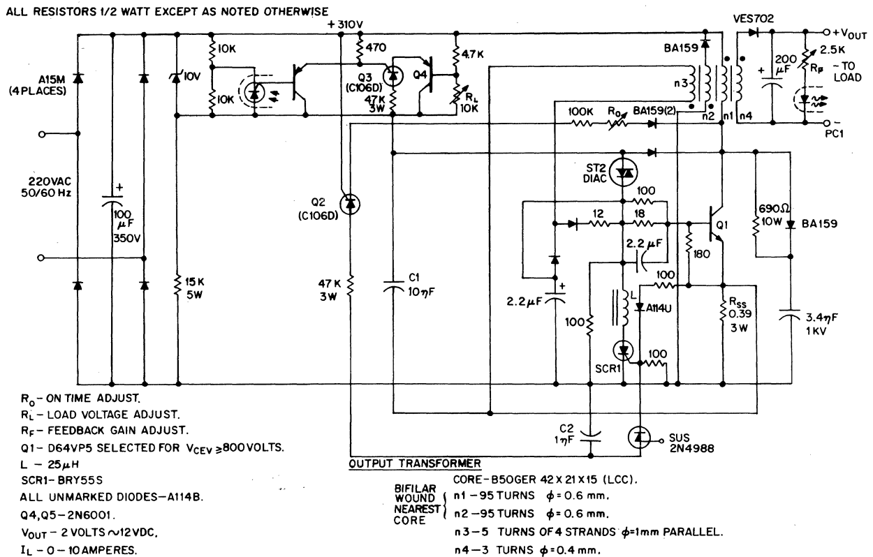
FIGURE 6.82: 12V SWITCHING POWER SUPPLY
