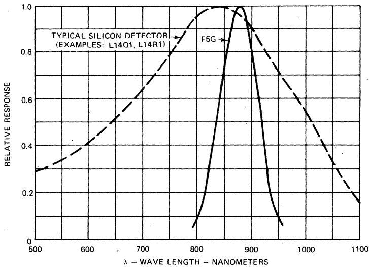
5. SPECTRAL RESPONSE
