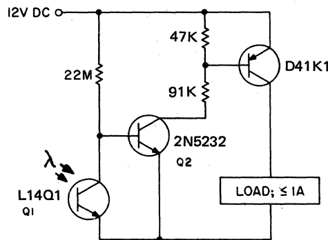
FIGURE 1.5: USE OF PHOTOTRANSISTOR AT VERY LOW LIGHT LEVELS
