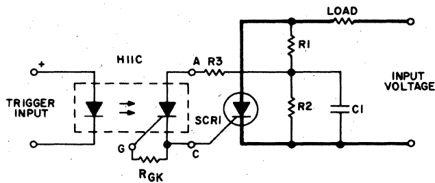
FIGURE 6.64: TRIGGERING SCR WITH PHOTON COUPLER AND SUPPLY VOLTAGE DIVIDER
