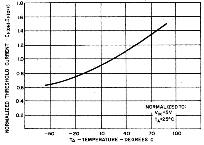
4. THRESHOLD CURRENTS VS. TEMPERATURE
