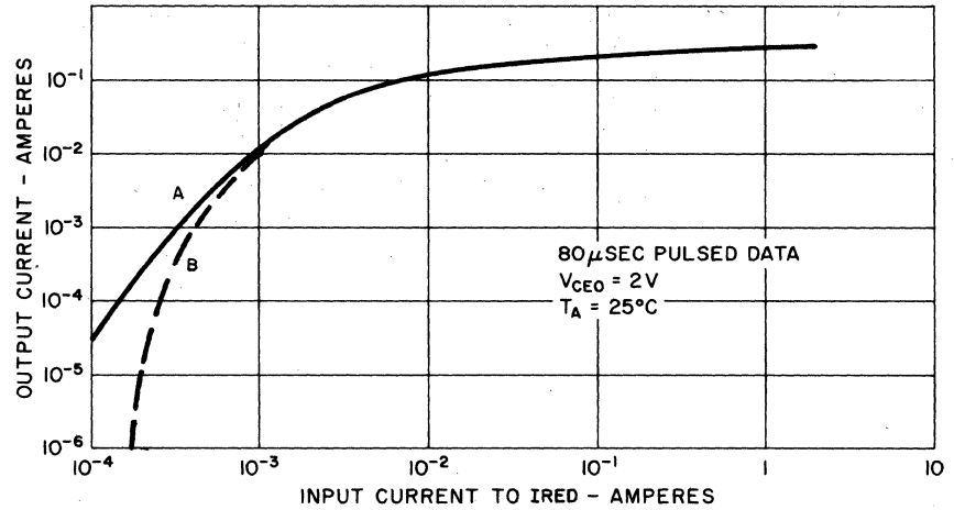
FIGURE 2.31: TYPICAL PHOTODARLINGTON OPTOCOUPLER TRANSFER CHARACTERISTICS
