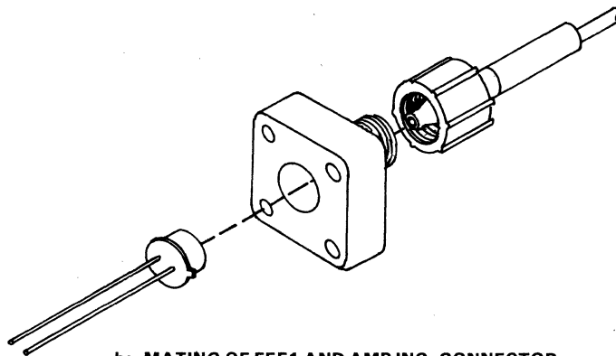
b: MATING OF F5E1 AND AMP INC. CONNECTOR
