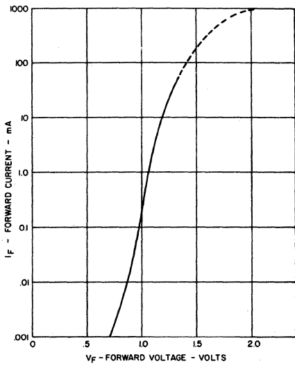
INPUT CHARACTERISTICS
