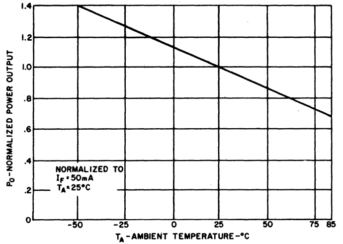
2. POWER OUTPUT VS. TEMPERATURE
