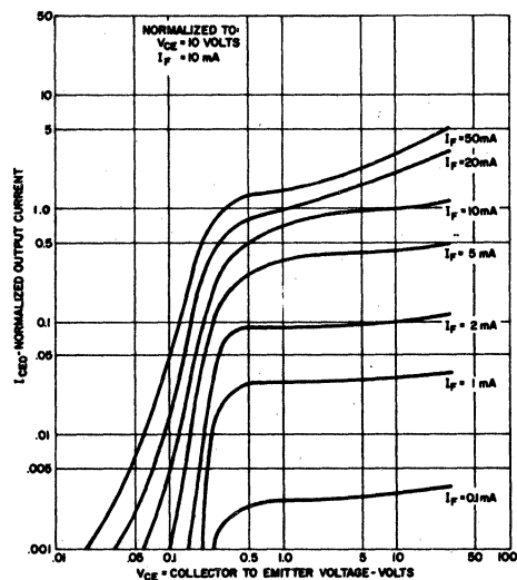
5. OUTPUT CHARACTERISTICS
