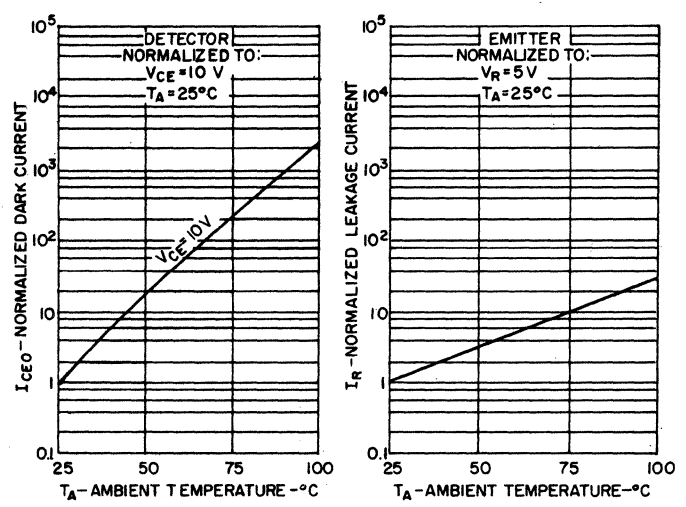
6. LEAKAGE CURRENTS VS. TEMPERATURE
