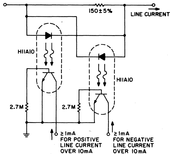
FIGURE 6.35: POLARITY INDICATING LINE CURRENT DETECTOR
