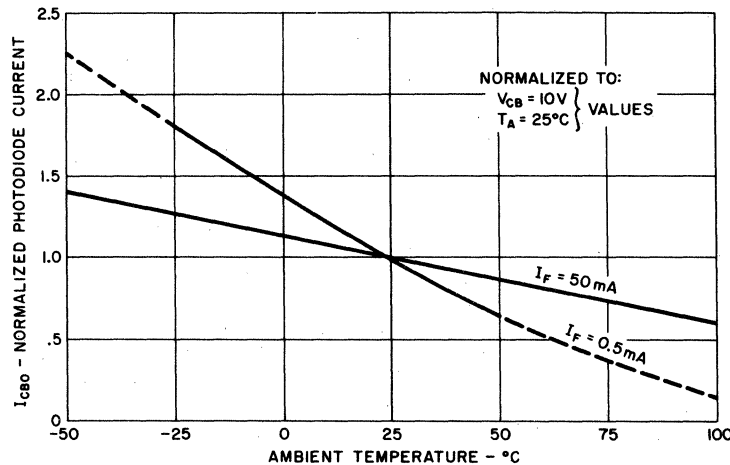
FIGURE 2.26: PHOTODIODE TRANSFER CHARACTERISTICS TEMPERATURE VARIATION
