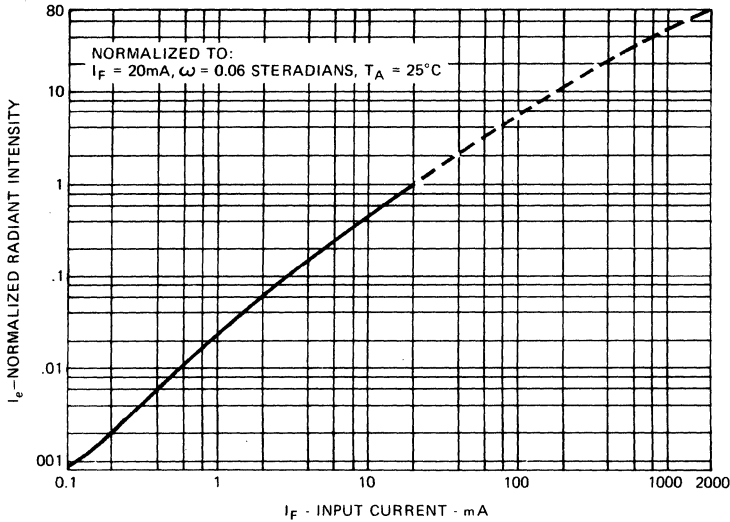
1. RADIANT INTENSITY VS. INPUT CURRENT
