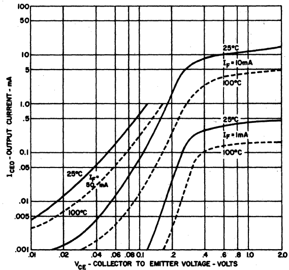
6. OUTPUT CHARACTERISTICS
