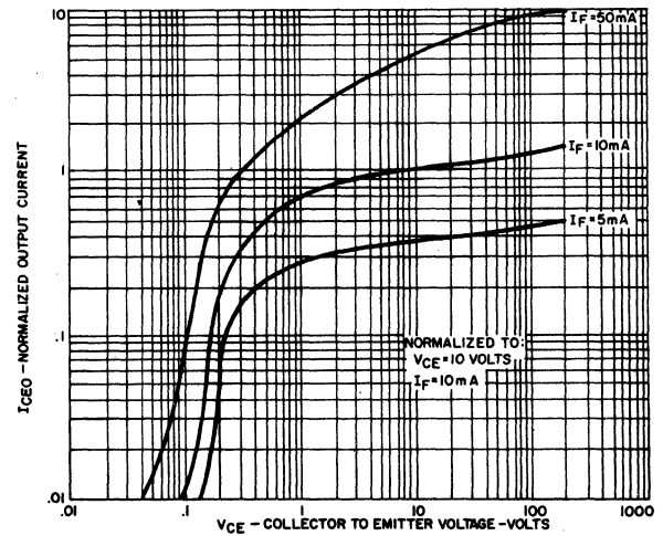
4. OUTPUT CHARACTERISTICS
