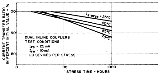
FIGURE 3.7b: EFFECT OF STRESS TEMPERATURE ON SLOPE
