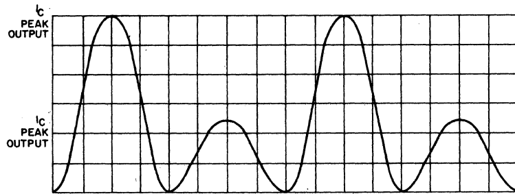
I_{CEO} OUTPUT WAVE FORM (SEE NOTE 2) AT V_{CE} = 5V
