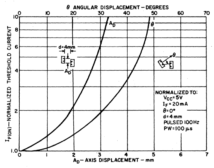
8. THRESHOLD CURRENT VS. DISPLACEMENT (ANGULAR AND AXIS)
