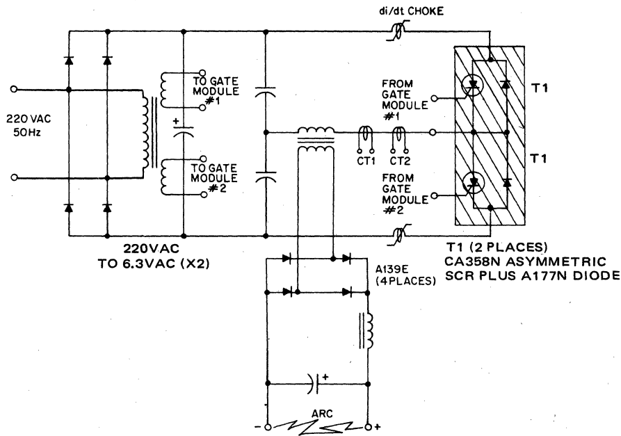
FIGURE 6.78: CLASS "A" - 3KW WELDING INVERTER
