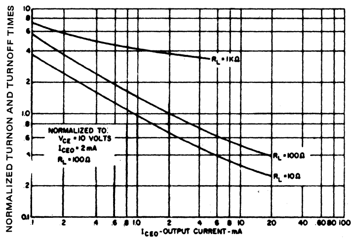
FIGURE 2. SWITCHING TIMES VS. OUTPUT CURRENT
