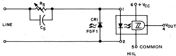
FIGURE 6.38: DIGITAL DATA LINE RECEIVER
