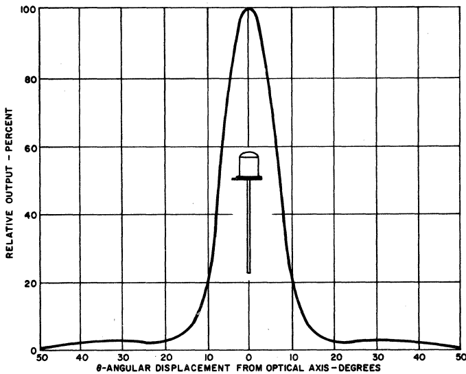
5. CQX14-CQX16 TYPICAL RADIATION PATTERN
