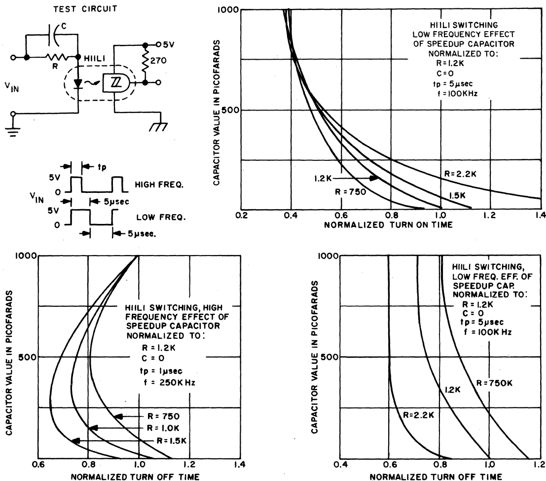
FIGURE 2.43: H11L SWITCHING
