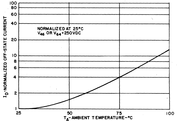
FIGURE 4. OFF-STATE CURRENT VS. TEMPERATURE
