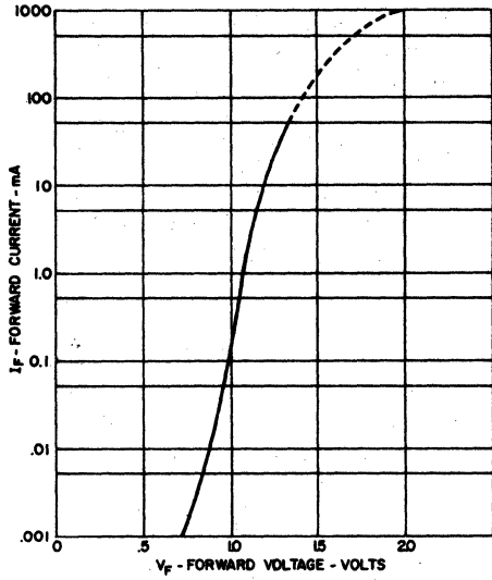
1. INPUT CHARACTERISTICS
