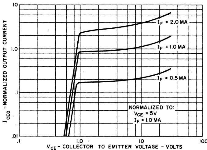
OUTPUT CHARACTERISTICS
