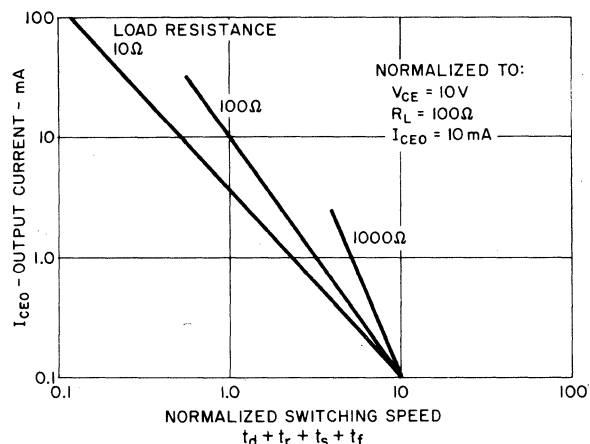
FIGURE 2.33: PHOTODARLINGTON SWITCHING SPEED AS A FUNCTION OF BIAS
