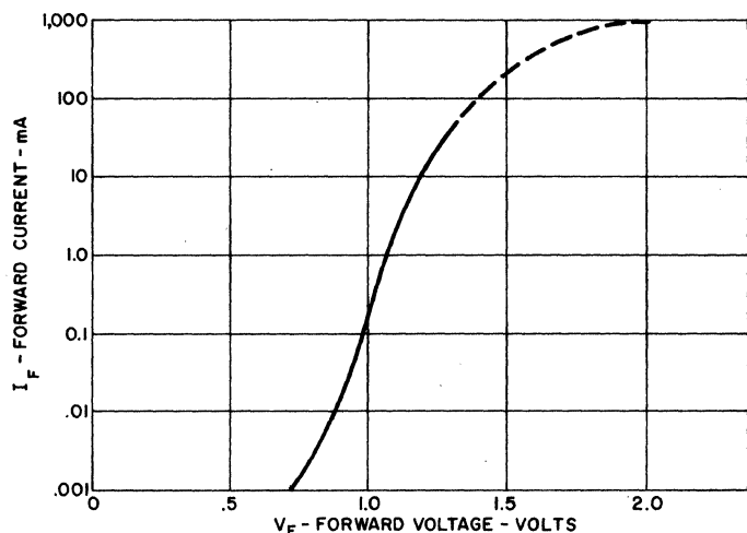
3. INPUT CHARACTERISTICS
