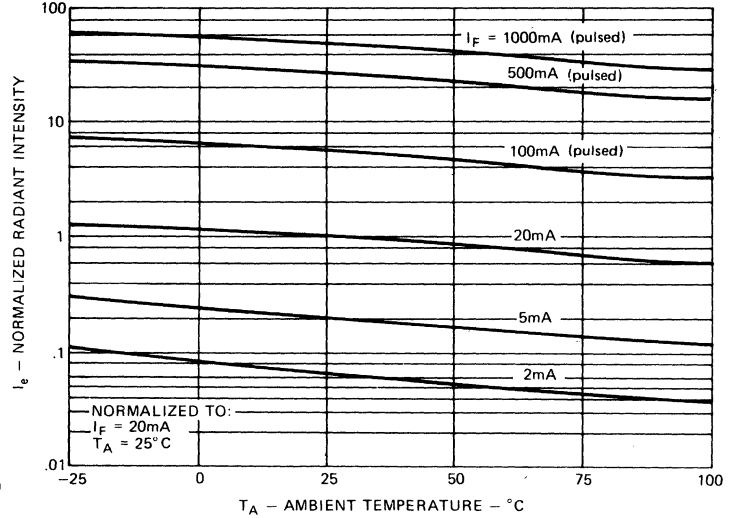
2. RADIANT INTENSITY VS. TEMPERATURE
