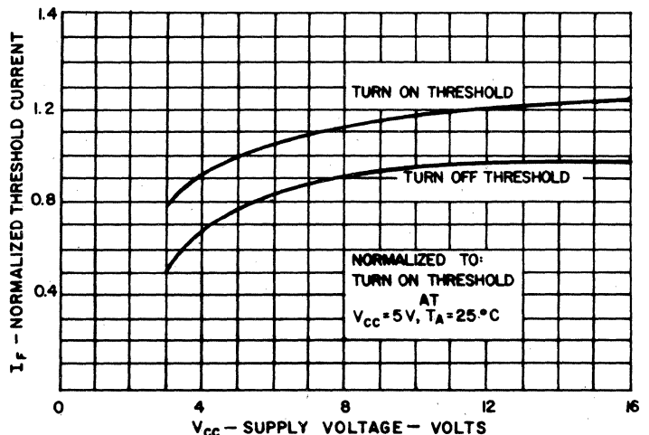
THRESHOLD CURRENT VS. SUPPLY VOLTAGE
