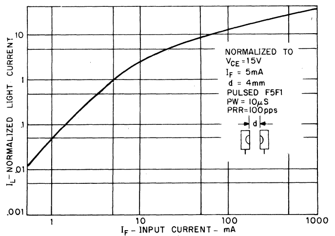
6. COUPLED LIGHT CURRENT VS. F5F1 INPUT CURRENT
