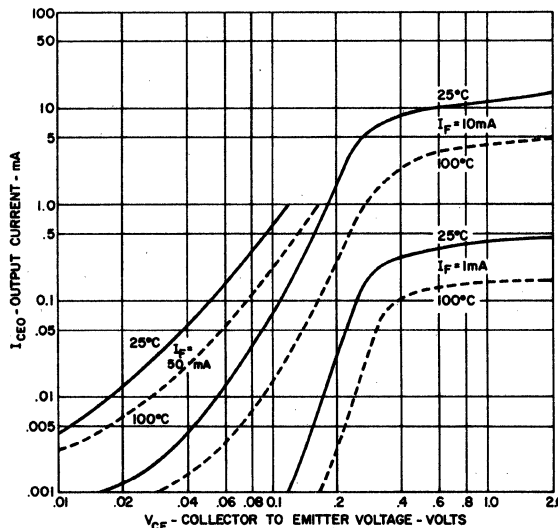
6. OUTPUT CHARACTERISTICS
