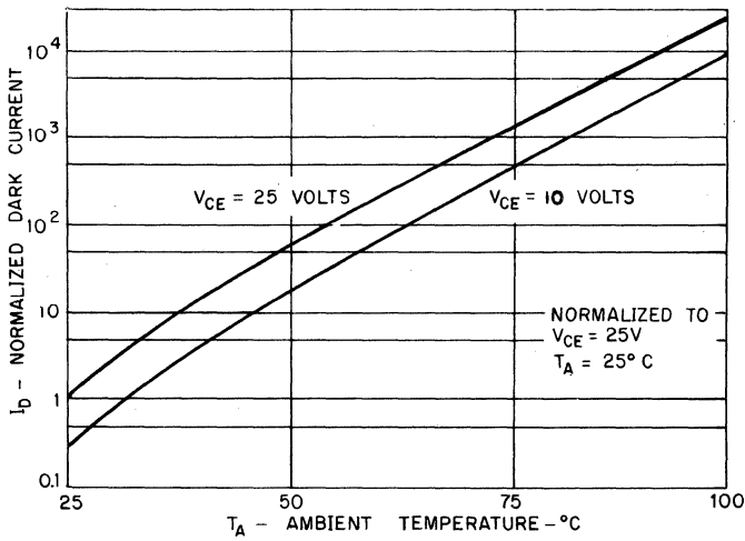
3. LEAKAGE CURRENT VS. TEMPERATURE
