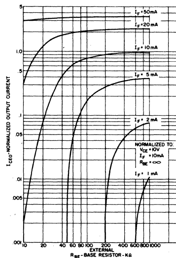
6. OUTPUT CURRENT VS BASE EMITTER RESISTANCE
