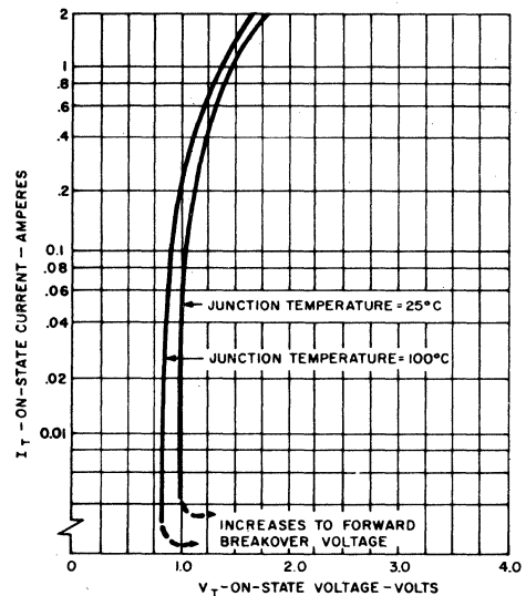
FIGURE 6. ON-STATE CHARACTERISTICS
