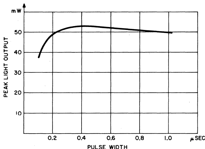
FIGURE 6.19: PEAK LIGHT OUTPUT EXPECTED FOR P_{AVE} = .25W , f = 80KHz OPERATION
