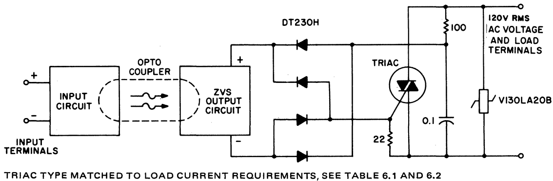
FIGURE 6.50: ZERO VOLTAGE SWITCHING SOLID STATE RELAY
