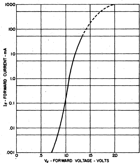
1. INPUT CHARACTERISTICS
