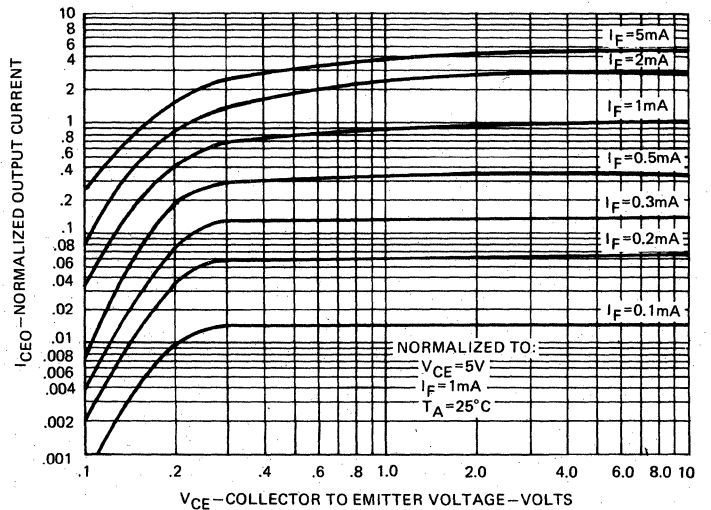
OUTPUT CURRENT VS. COLLECTOR-EMITTER VOLTAGE
