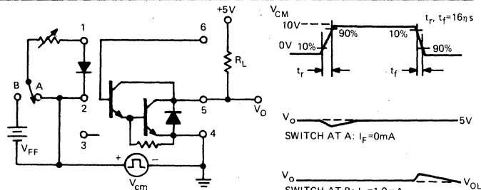
TEST CIRCUIT FOR TRANSIENT IMMUNITY AND TYPICAL WAVEFORMS
