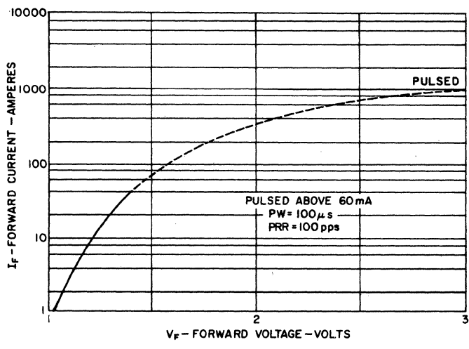
3. INPUT CHARACTERISTICS
