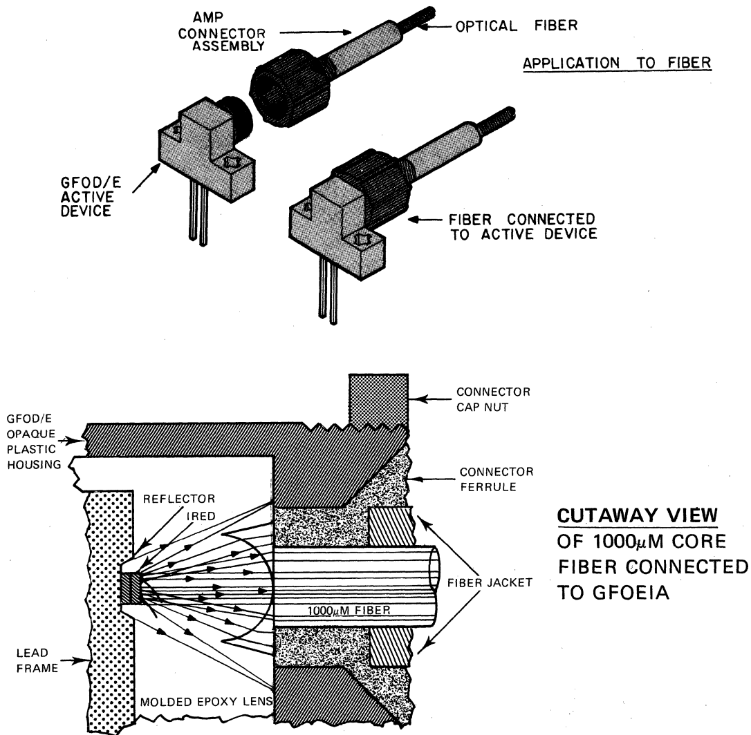
FIGURE 1.10: GFOD/E ACTIVE DEVICE WITH FIBER OPTICS TERMINATION
