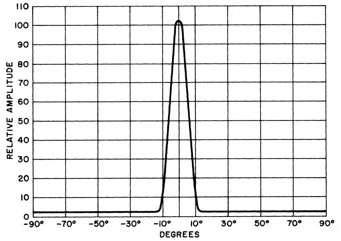
4. ANGULAR RESPONSE
