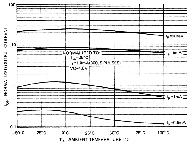
OUTPUT VS. TEMPERATURE
