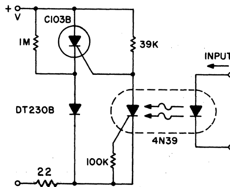
FIGURE 6.49: NORMALLY CLOSED, HALF WAVE ZVS CONTACT CIRCUIT
