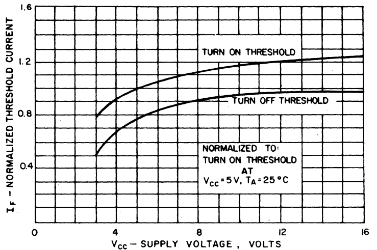
THRESHOLD CURRENT VS. SUPPLY VOLTAGE
