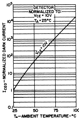
6. LEAKAGE CURRENTS VS. TEMPERATURE
