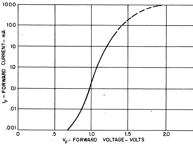
INPUT CHARACTERISTICS
