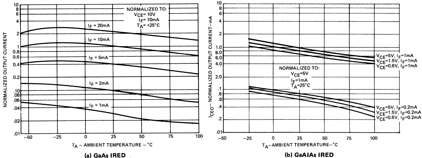
FIGURE 2.28: BIAS EFFECTS ON CTR TEMPERATURE COEFFICIENT
