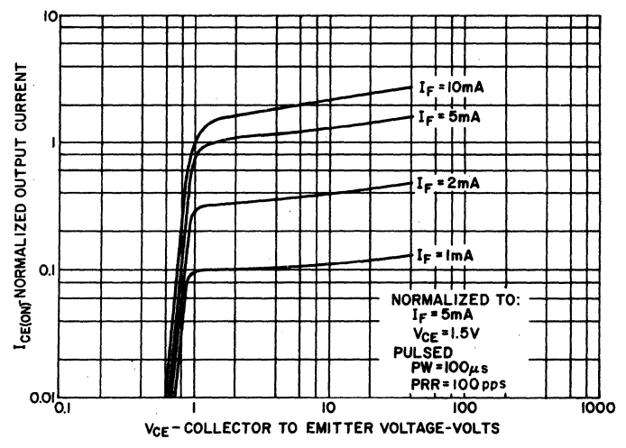
4. OUTPUT CHARACTERISTICS
