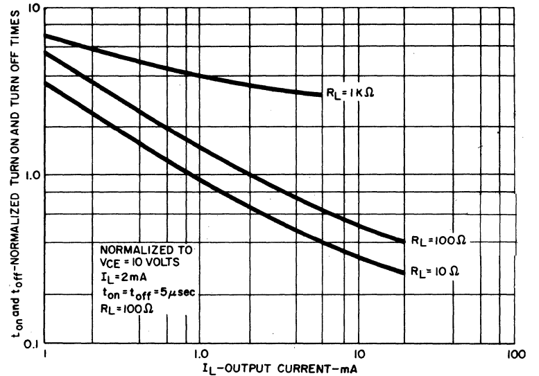
SWITCHING TIMES VS OUTPUT CURRENT
