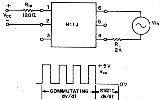
FIGURE 6. dv/dt - TEST CIRCUIT
