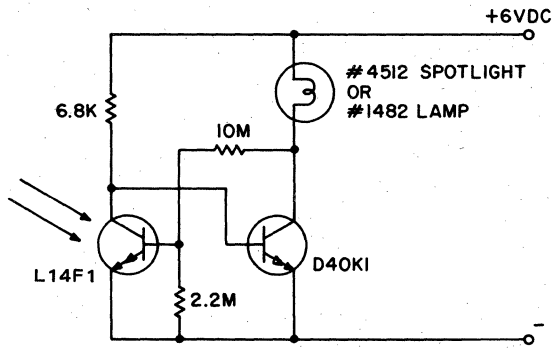
FIGURE 6.5: PORTABLE AUTOMATIC NIGHT LIGHT
