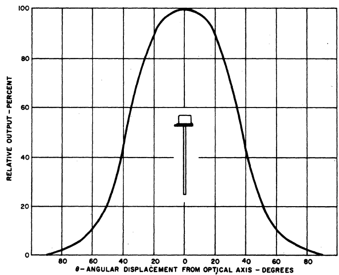
6. 1N6265 - TYPICAL RADIATION PATTERN
