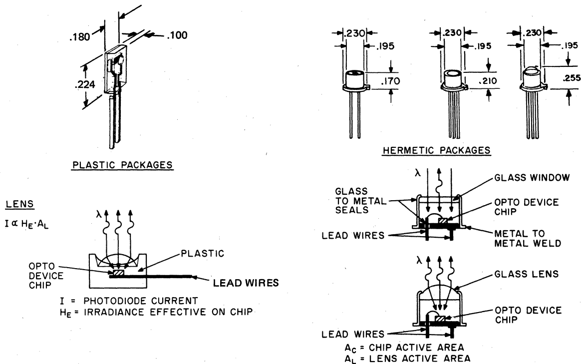
FIGURE 1.9: DISCRETE OPTOELECTRONIC COMPONENT PACKAGE CONCEPTS
