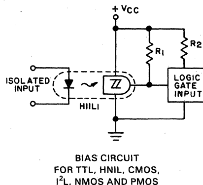
FIGURE 2.44: H11L INPUT FOR LOGIC CIRCUITS, SUGGESTED BIAS RESISTORS
