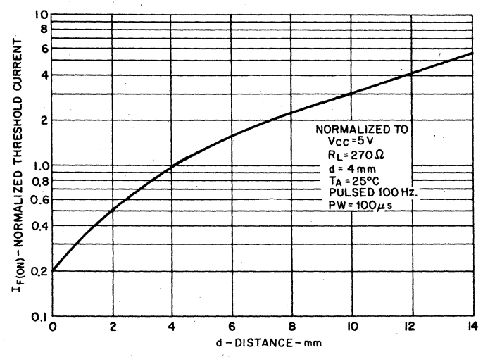
7. THRESHOLD CURRENT VS. DISTANCE
