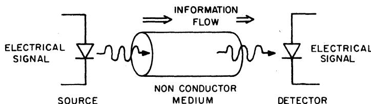
FIGURE 2.46: TYPICAL FIBER OPTIC SYSTEM
