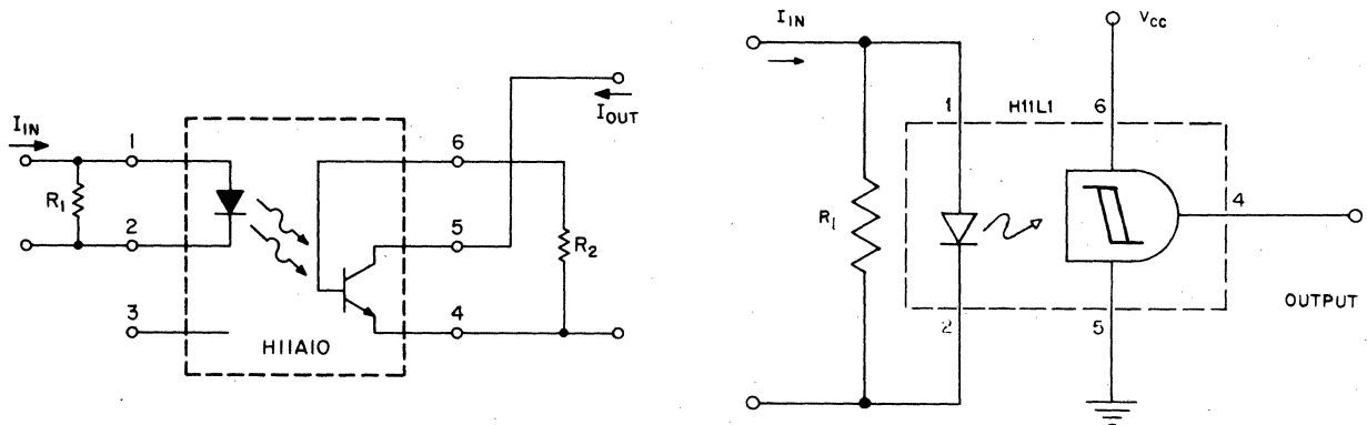
FIGURE 2.22: CURRENT THRESHOLD OPERATION OF OPTOCOUPLER
