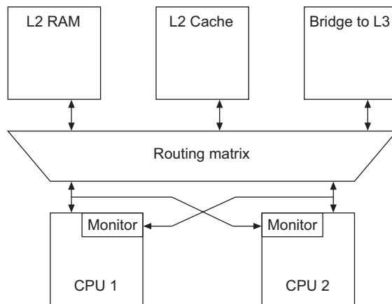
Figure A2-3 Write snoop monitor approach
