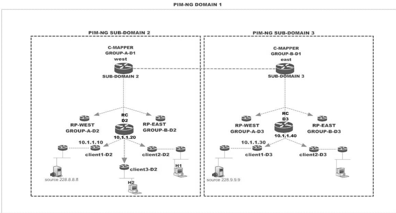
Figure 53 Sample PIM-NG domain Divided to Sub-Domains
