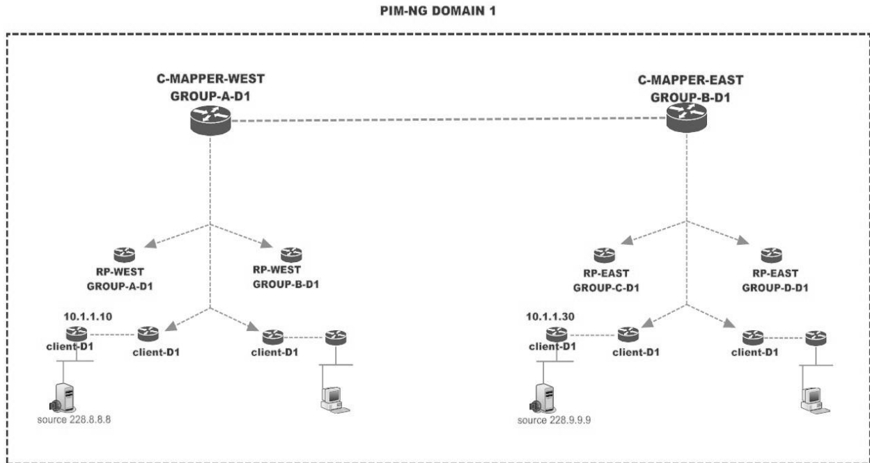
Figure 33 network with single multicast domain and redundant C-MAPPERS
