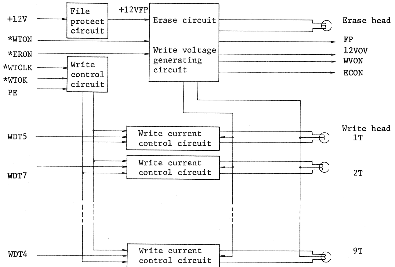
Figure 3.32 Write circuit
