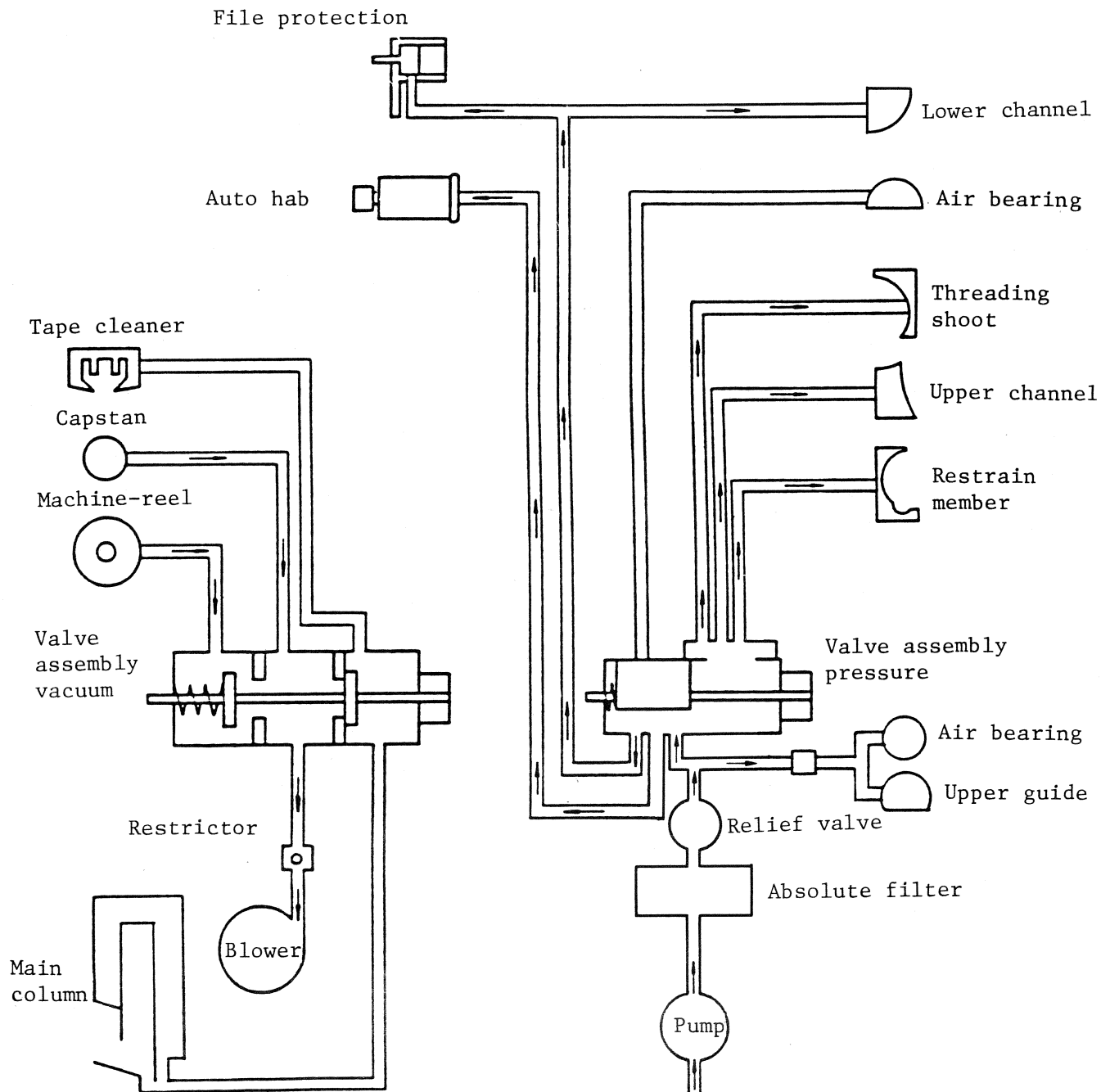
Figure 2.27 Air supply system during autoloading operation
