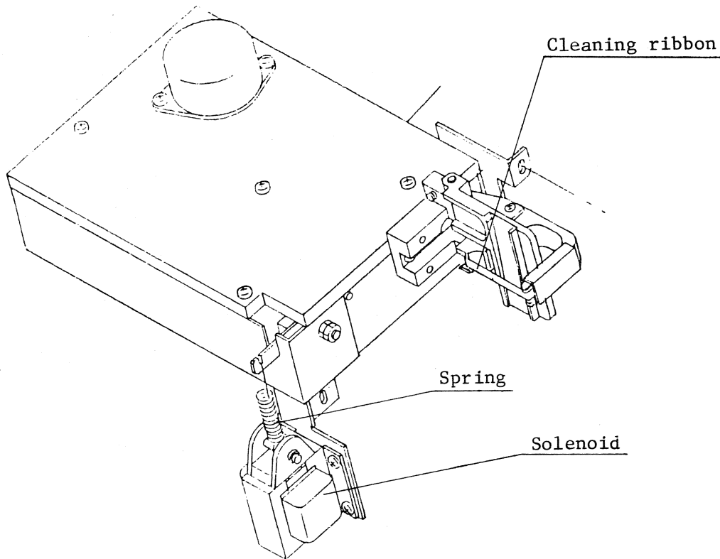
Figure 2.23 Autocleaner
