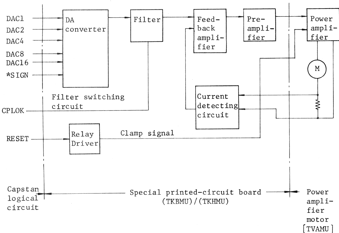
Figure 3.17 Block diagram of the capstan drive circuit
