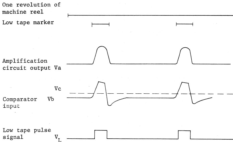
Figure 3.49 Low-tape waveforms
