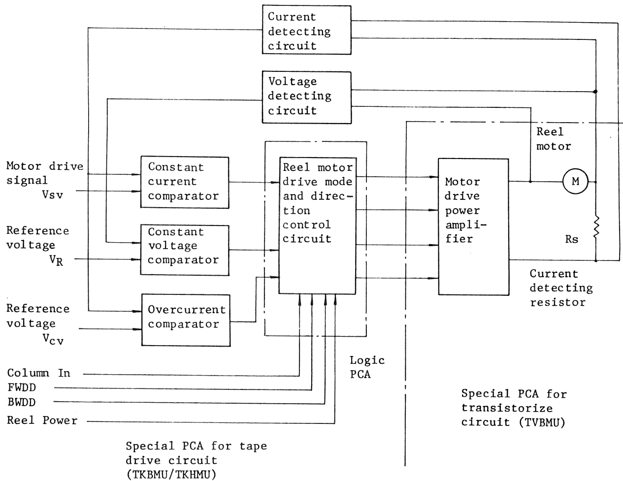
Figure 3.23 Reel motor drive circuit
