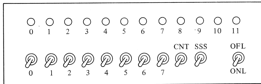
Figure 3.7 Maintenance panel
