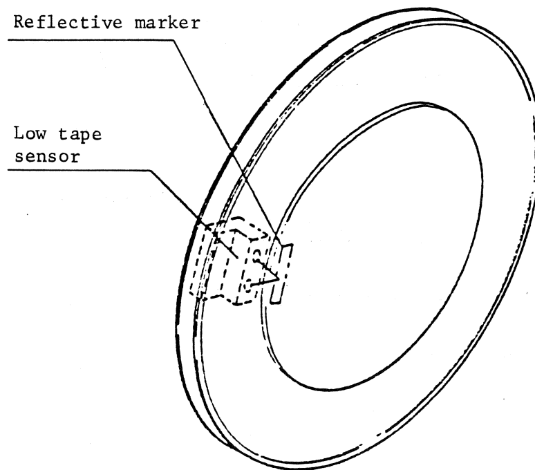
Figure 2.22 Low-tape sensor
