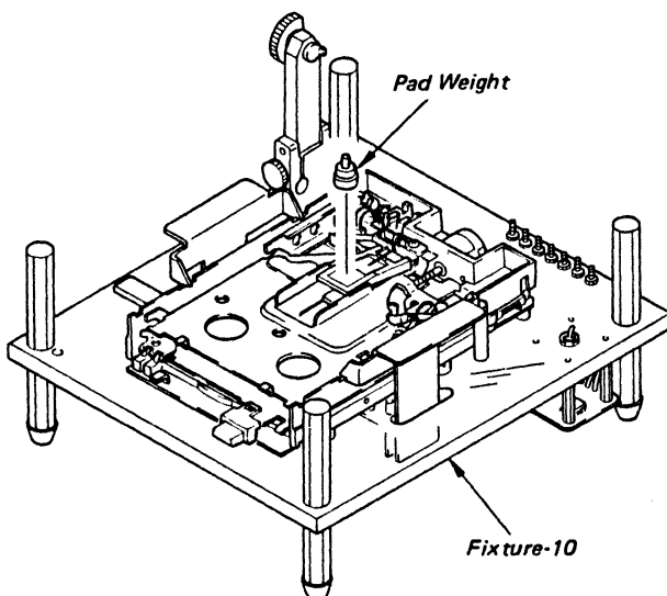
Fig. 5-2 Head Compliance Measurement
