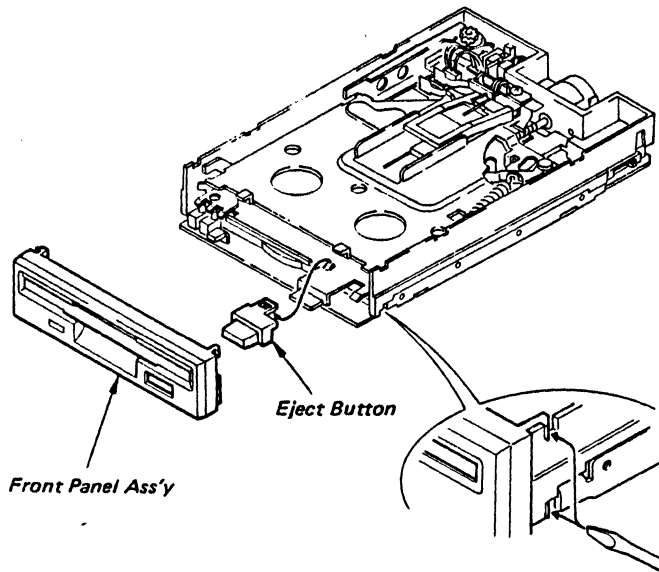
Fig. 4-2 Front Panel Ass'y Replacement
