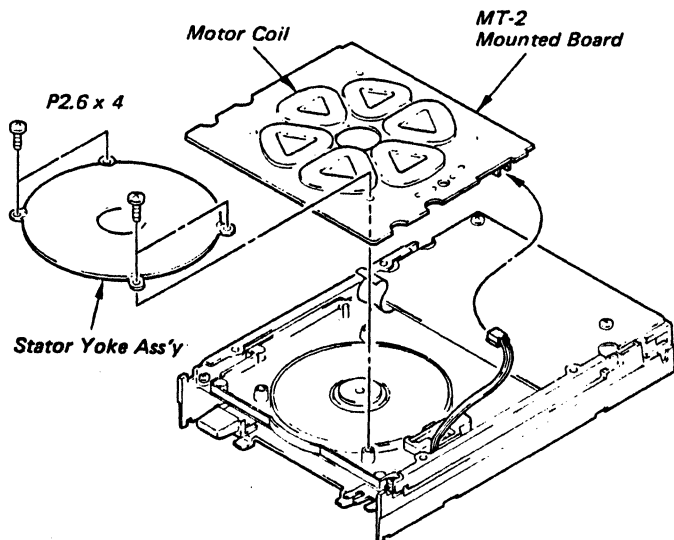
Fig. 4-4 MT-2 Mounted Board Replacement
