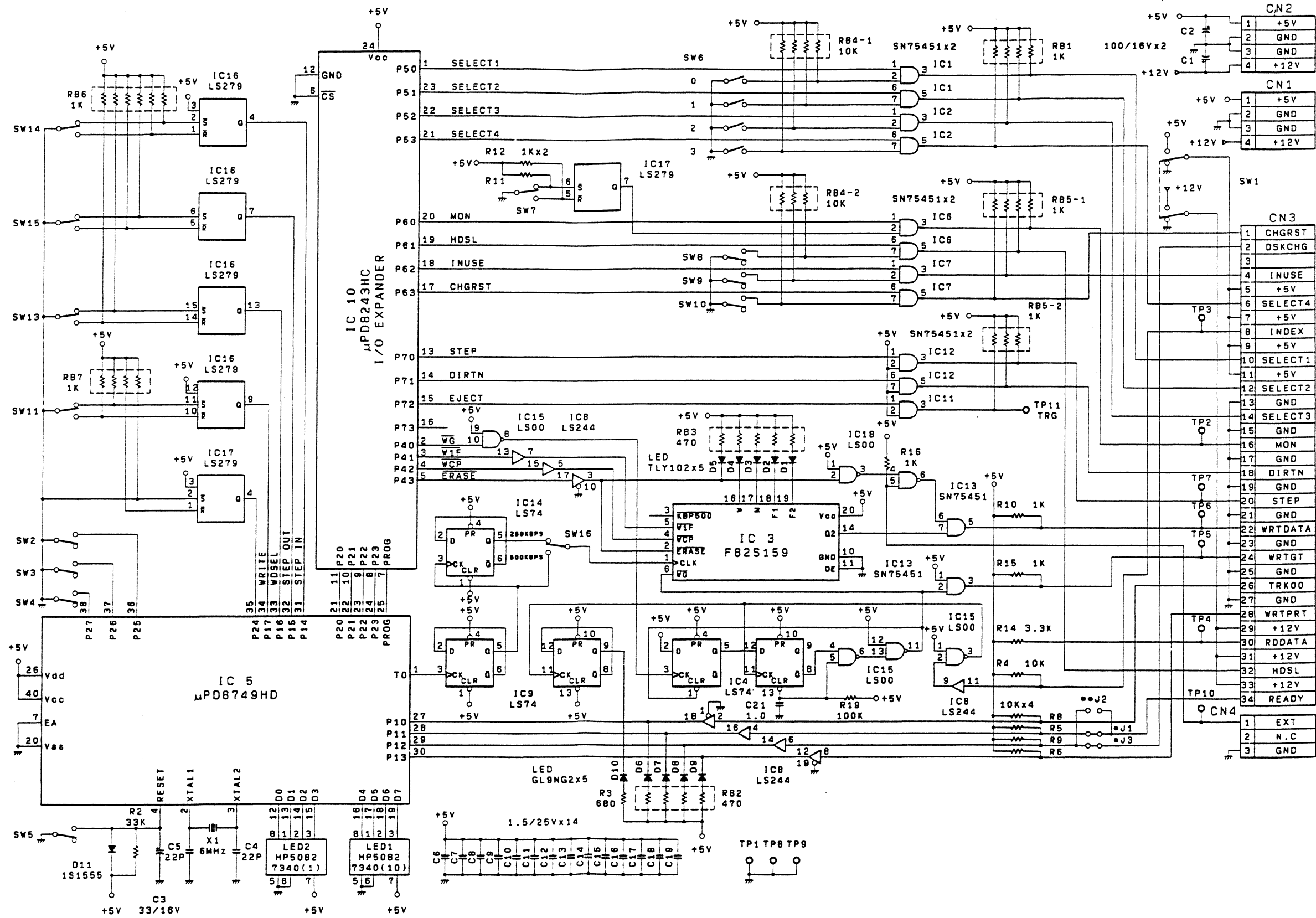
Fig. 2-3 MFD Function Checker II Circuit Diagram
