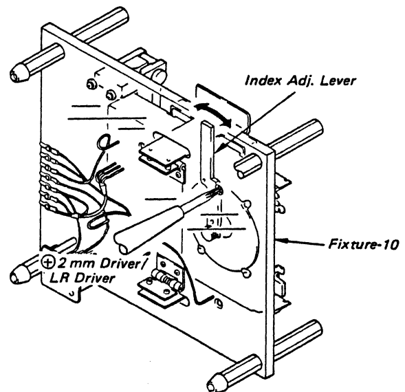
Fig. 5-3 (a) Index Phase Adjustment
