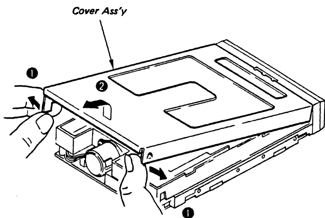
Fig. 4-1 Cover Ass'y Replacement
