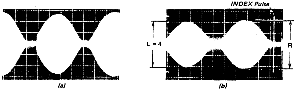
Fig. 3-4 Cat's eye Pattern Signal
