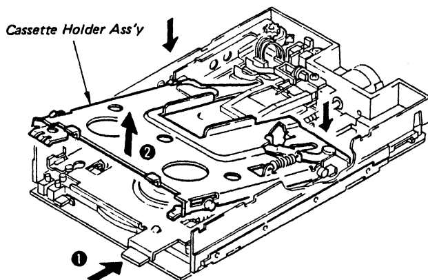
Fig. 4-6 Cassette Holder Ass'y Replacement
