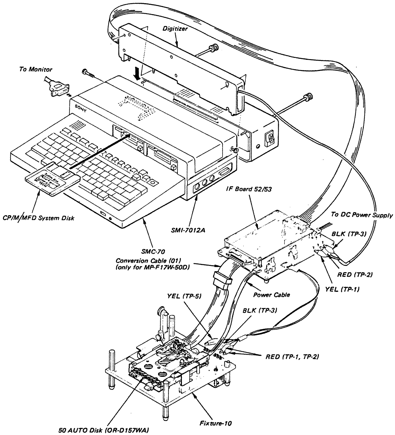
Fig. 2-16 System Configuration for Radial Alignment
