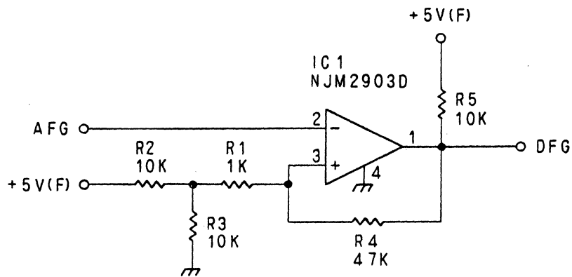
Fig. 2-12 FG PCB Circuit Diagram
