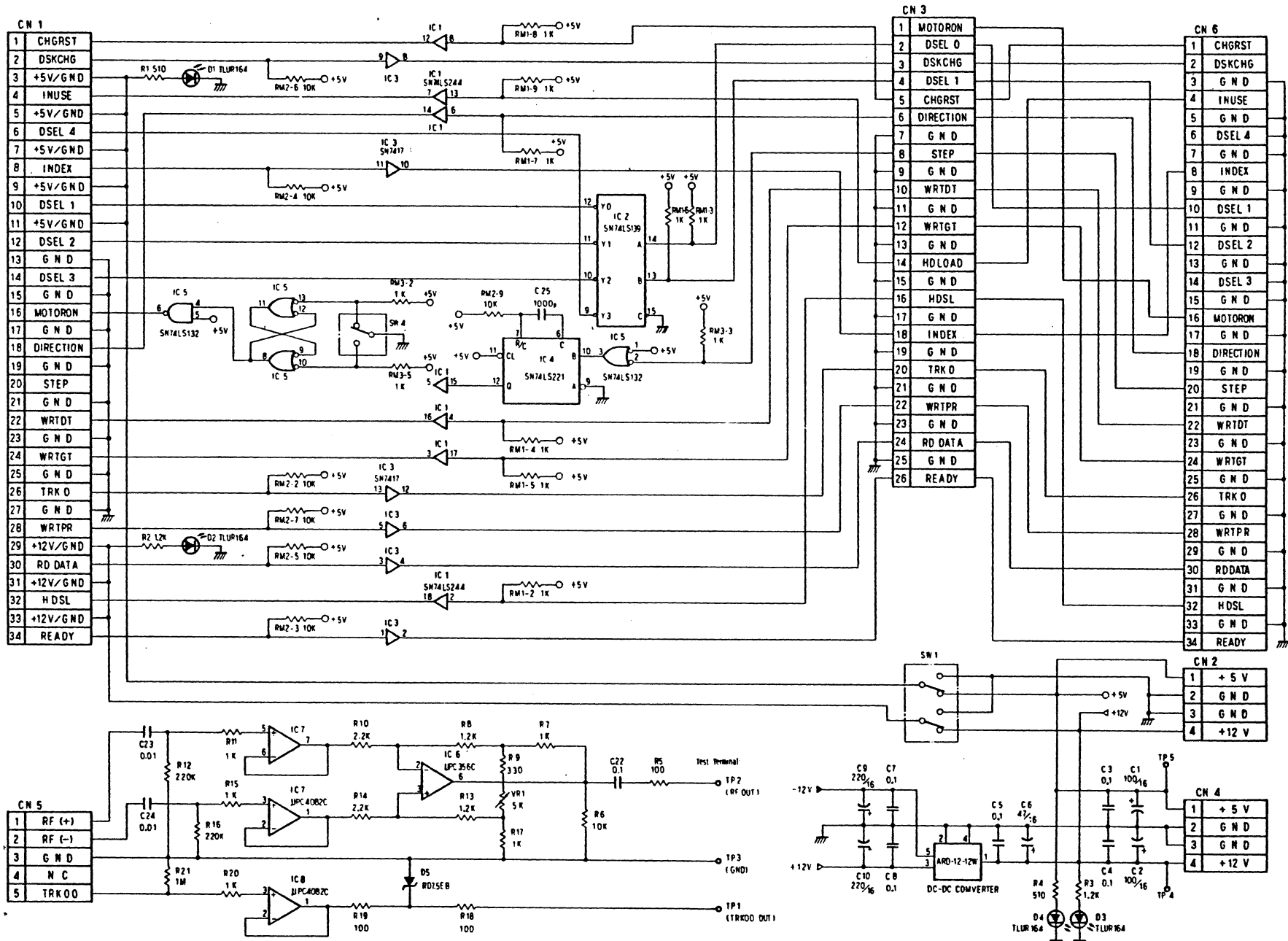
Fig. 2-6 IF Board Circuit Diagram
