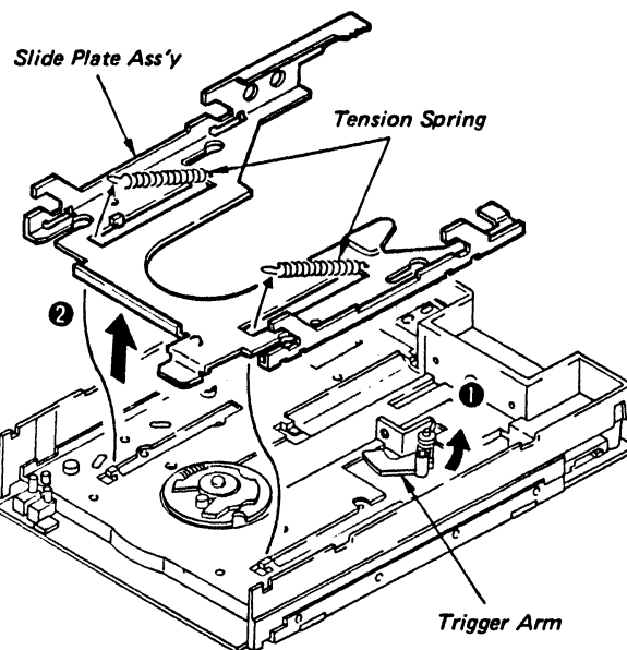
Fig. 4-7 Slide Plate Ass'y Replacement
