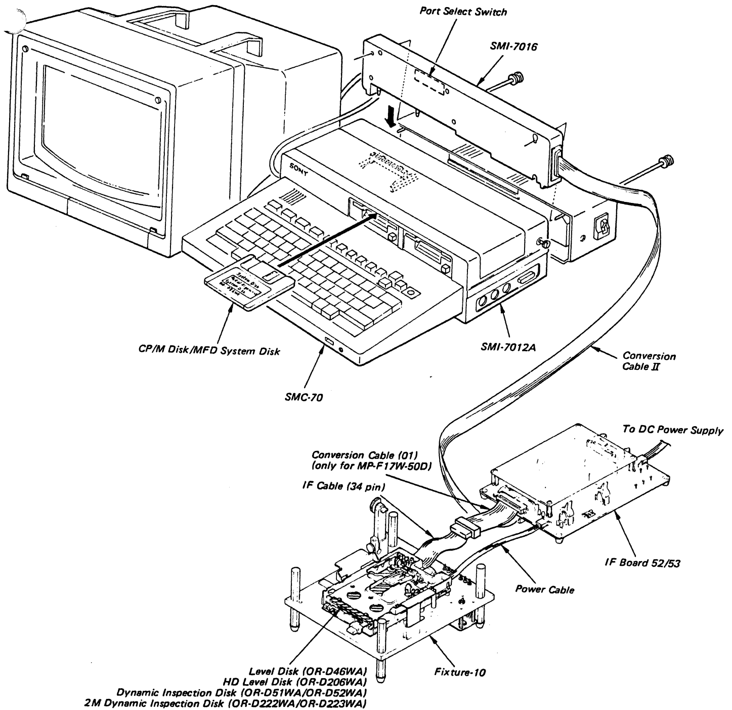
Fig. 2-15 System Configuration for Drive Test
