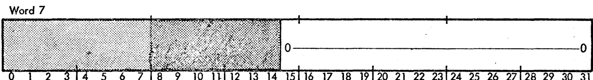
Figure 16. Format of the DDCB
