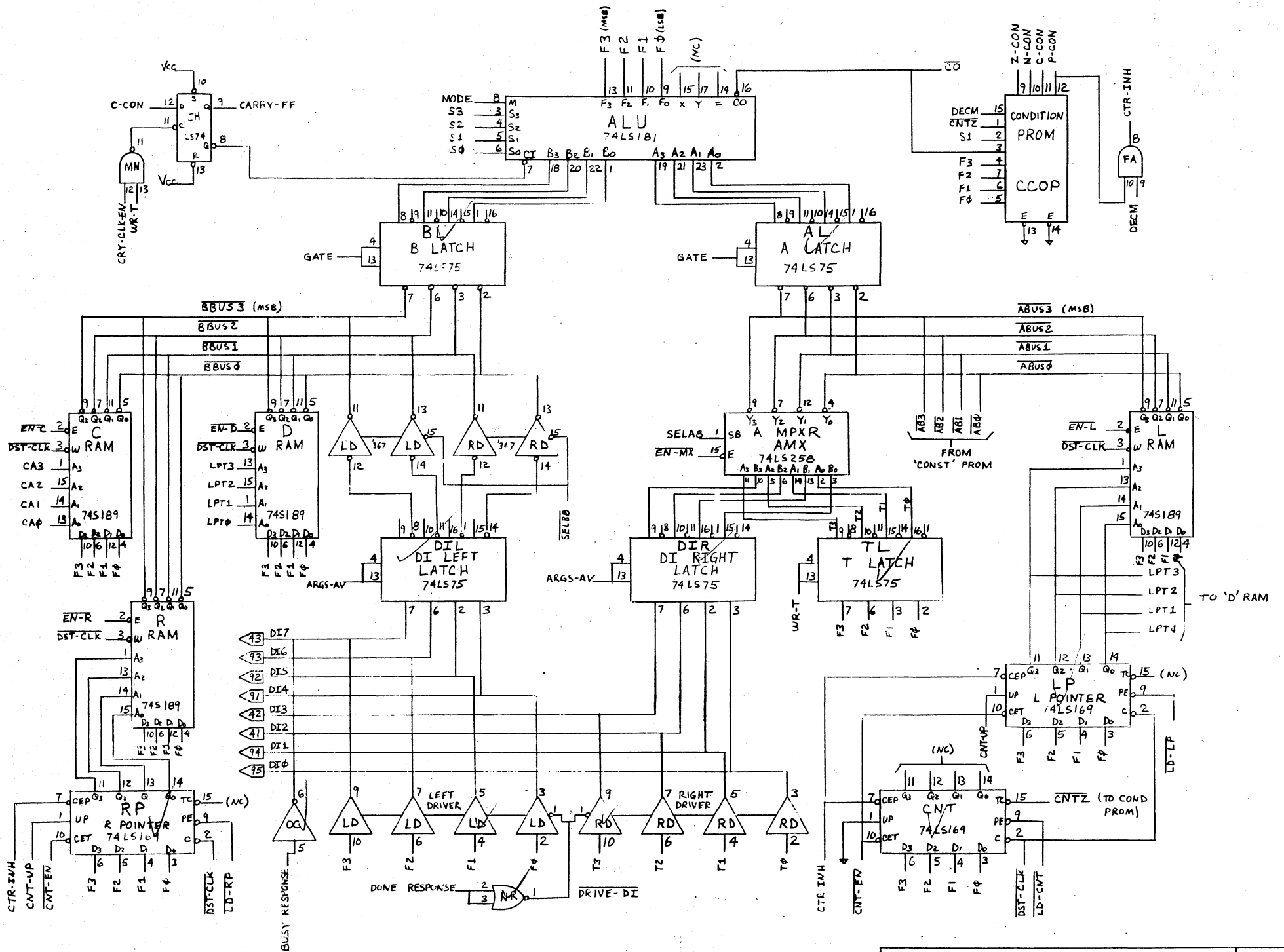
SCHEMATIC — DATA PATHS
