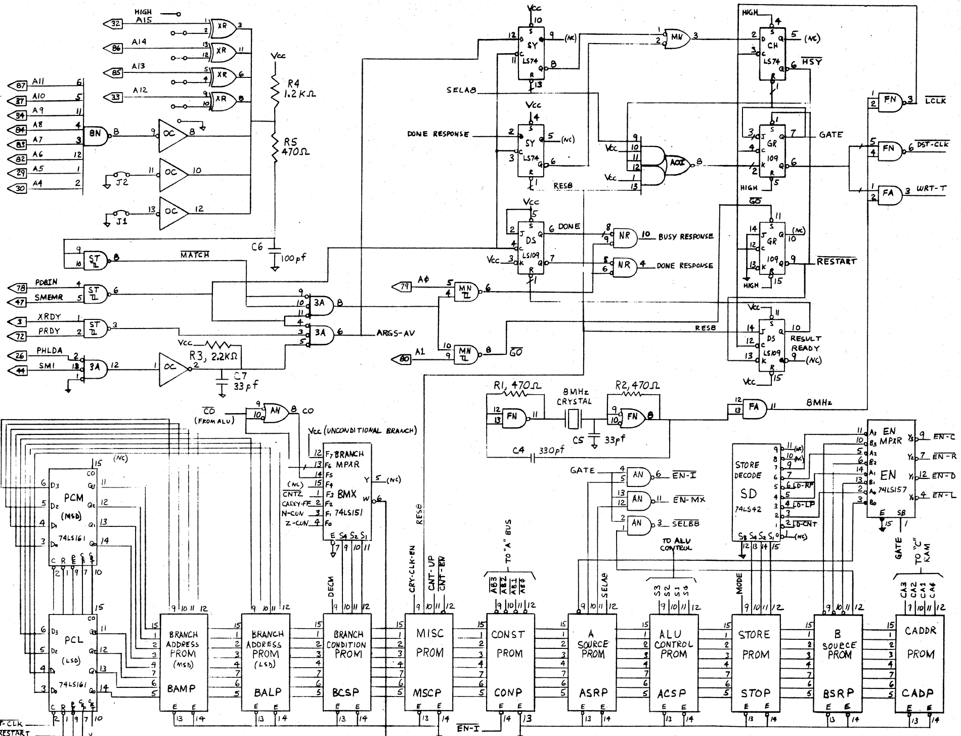
SCHEMATIC - CONTROL LOGIC
