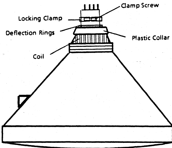
Figure 7.4 Yoke alignment
