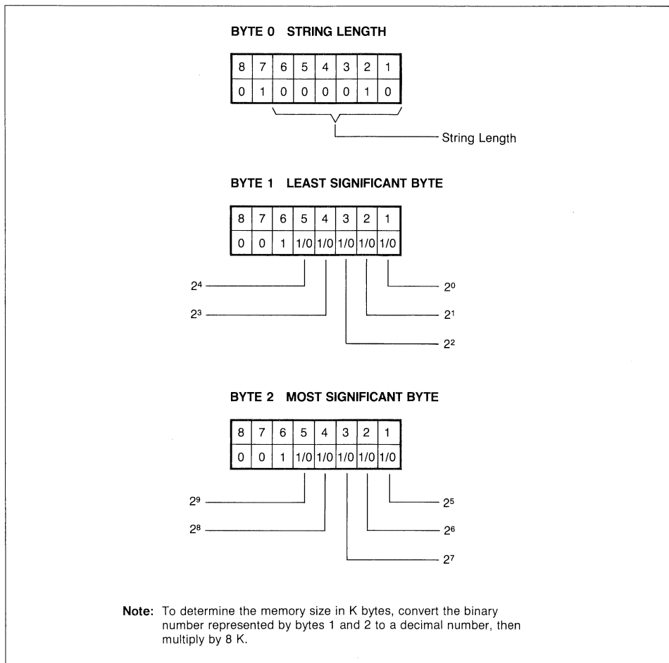
Figure 7-6. Installed Memory Status Bytes
