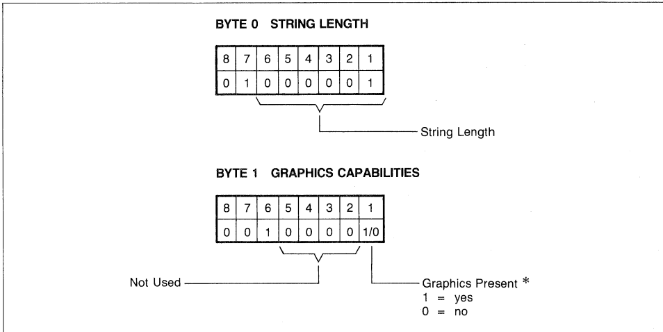
Figure 7-5. Terminal Graphics Capabilities Status Bytes
