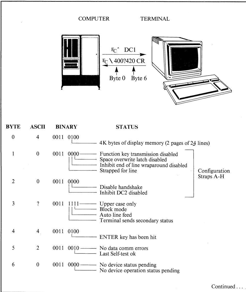
Figure 7-1. Primary Terminal Status Example
