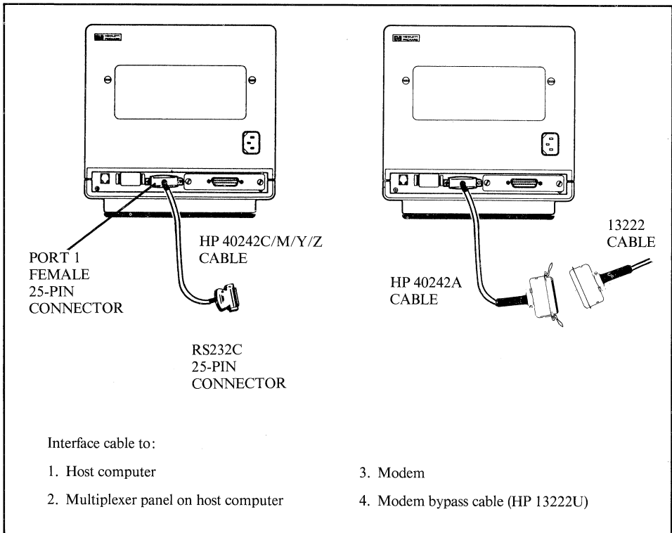
Figure 6-2. Terminal Cabling (HP 40242 and 13222 Cables)
