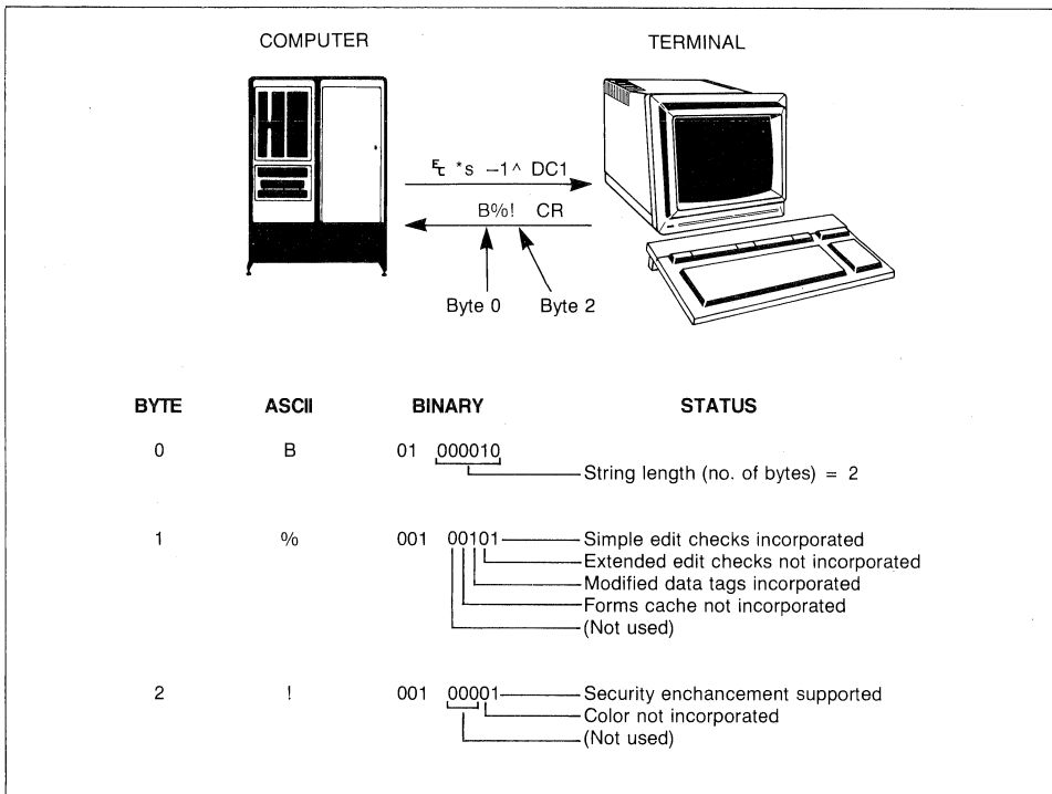
Figure 7-3. Terminal Capabilities (Alphanumeric-Typical) Status Example
