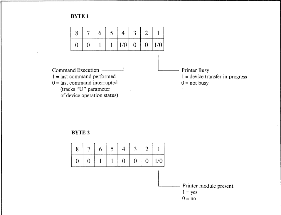
Figure 7-8. External Device Status Bytes (Continued)
