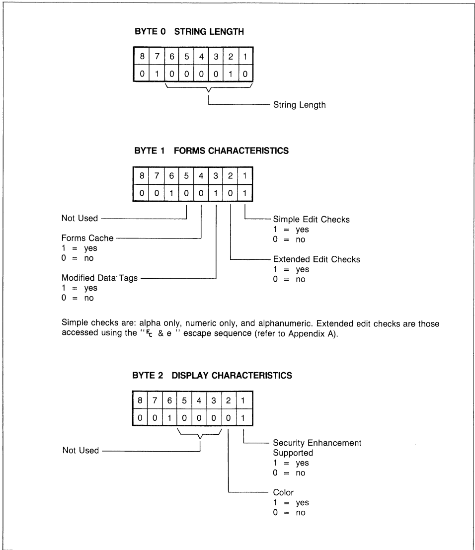
Figure 7-4. Terminal Alphanumeric Capabilities Status Bytes
