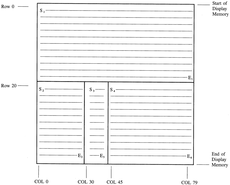
Figure 4-9. Bottom Horizontal Tab Sequence Example EC&a20i30s45S
