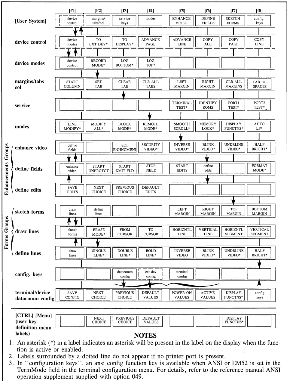
Figure 1-7. Function Key Hierarchy of the HP 2394A
