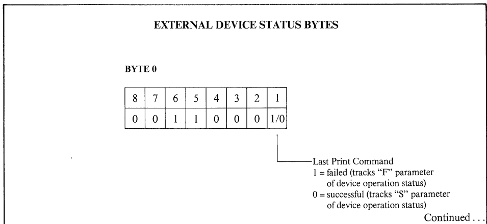
Figure 7-8. External Device Status Bytes
