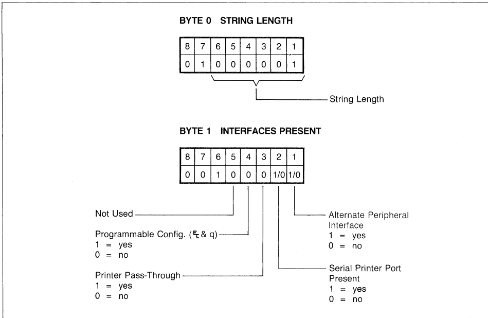
Figure 7-7. Terminal Interface Capabilities Status Bytes
