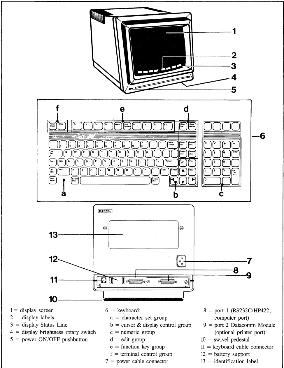
Figure 1-1. 2392A Display Terminal/2394A Data Entry Terminal
