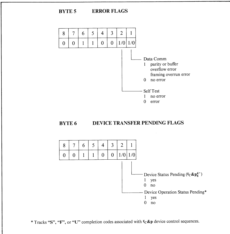
Figure 7-1. Primary Terminal Status Example (Continued)
