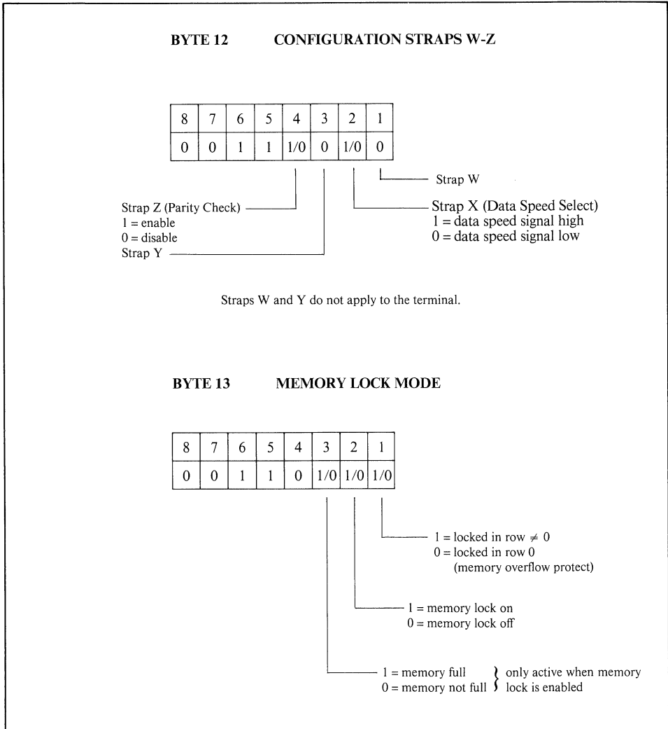
Figure 7-2. Secondary Terminal Status Example (Continued)
