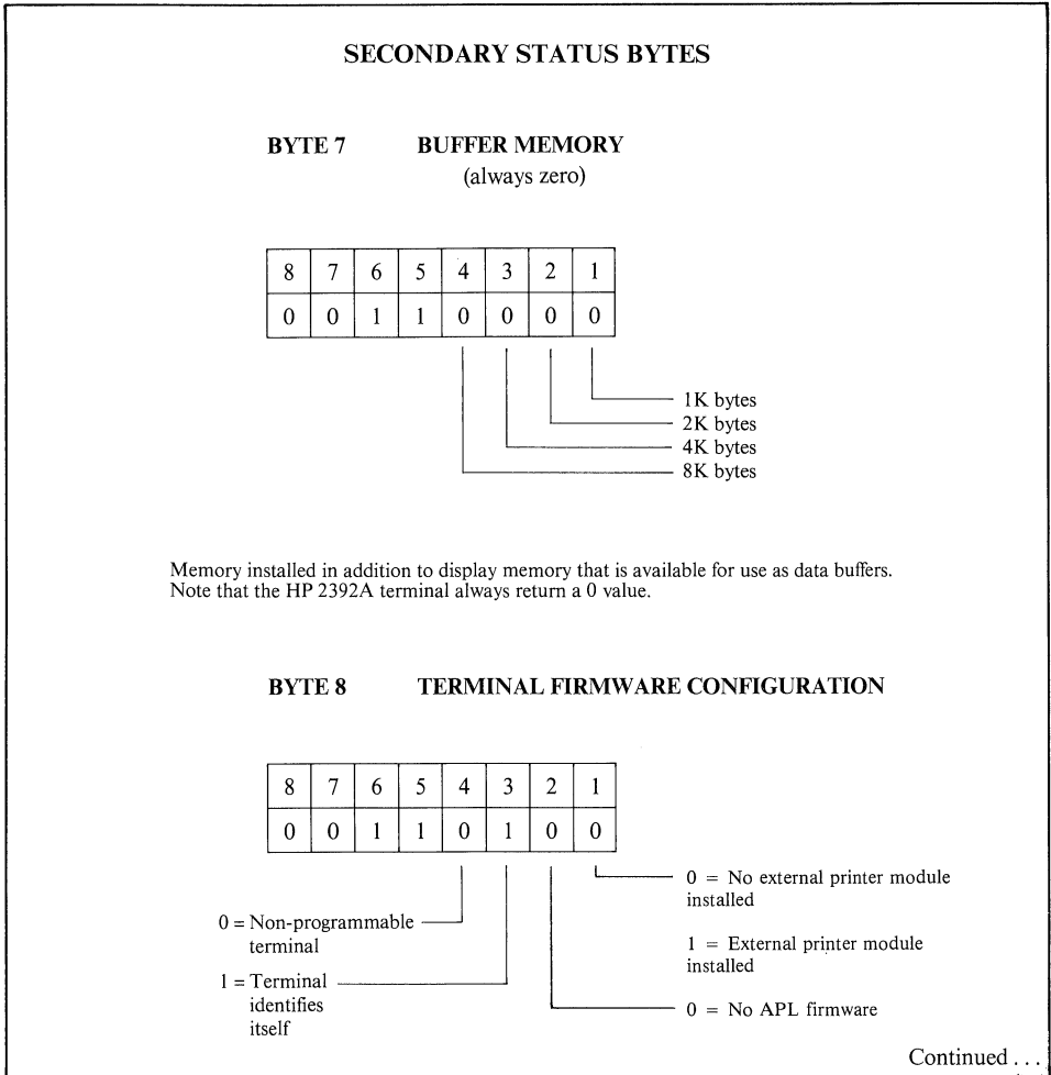
Figure 7-2. Secondary Terminal Status Example (Continued)
