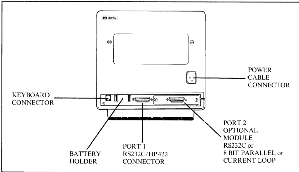
Figure 6-1. Terminal Rear View
